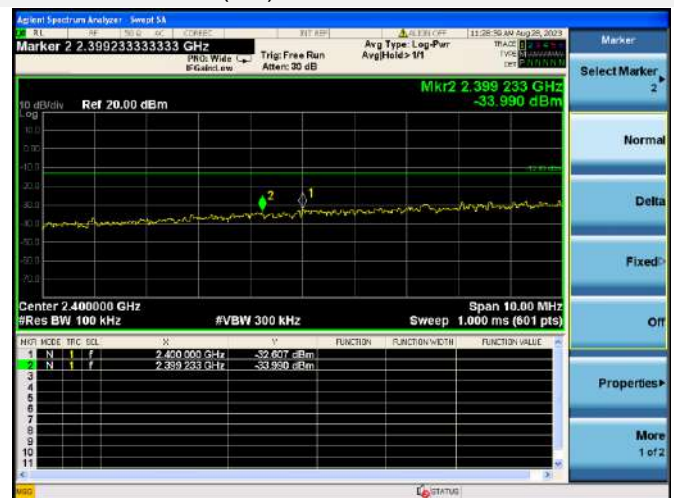
802.11ax-20 MHz(SU) CHANNEL 3, BAND EDGE
