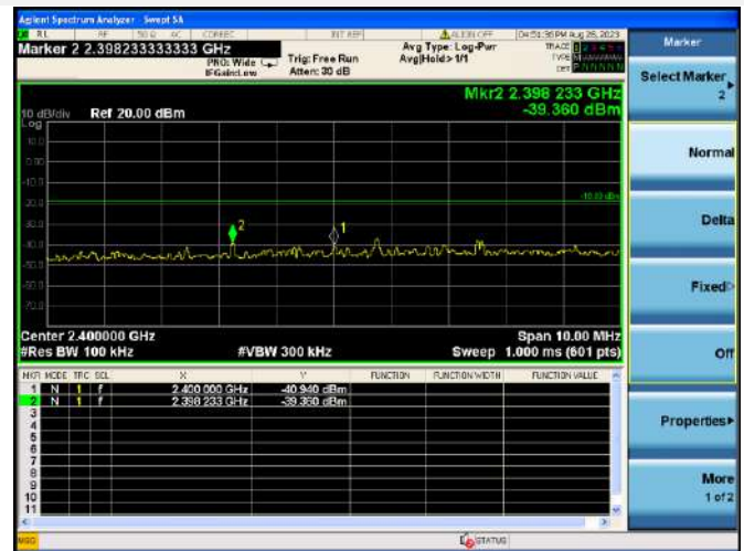
802.11ax-40 MHz(SU) CHANNEL 5, BAND EDGE
