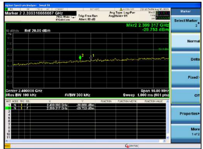
802.11ax-20 MHz(SU) CHANNEL 2, BAND EDGE
