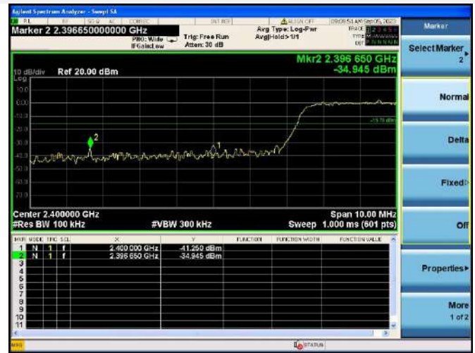
802.11ax-20 MHz(SU) CHANNEL 1, BAND EDGE
