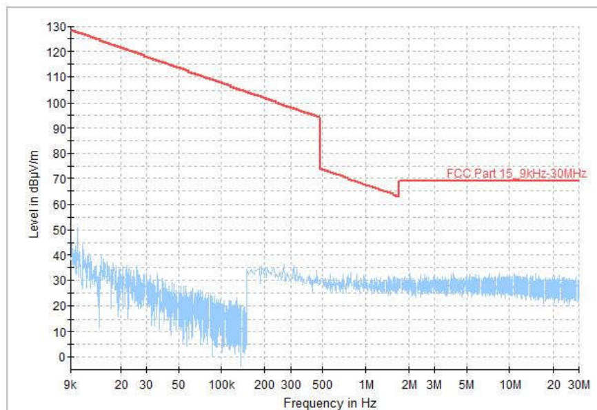
Fig.40 Radiated Spurious Emission (All Channels, 9kHz-30MHz), LE 1M
