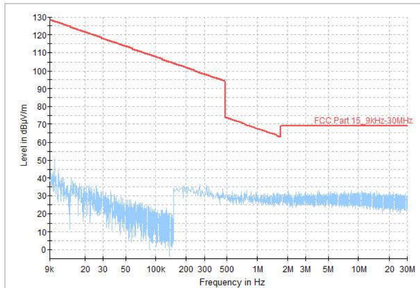
Fig.48 Radiated Spurious Emission (All Channels, 9kHz-30MHz), LE 2M
