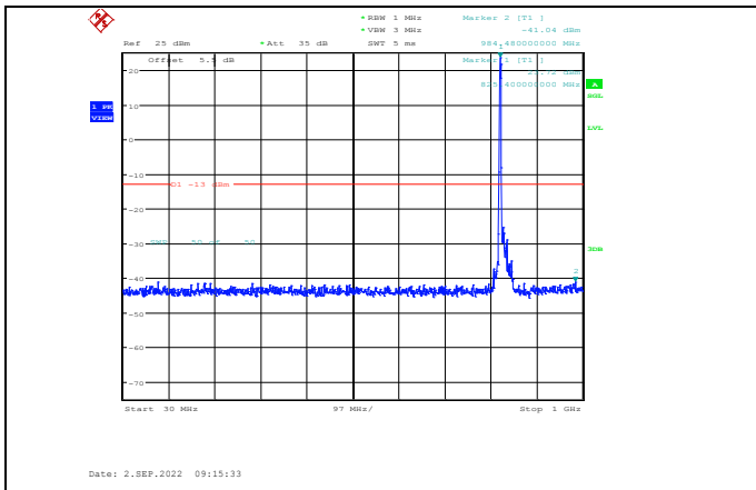
Band26-15MHz-64QAM-26865-1RB#0- Range1:30~1000MHz
