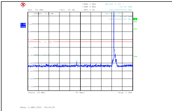
Band26-15MHz-16QAM-26865-1RB#0- Range1:30~1000MHz
