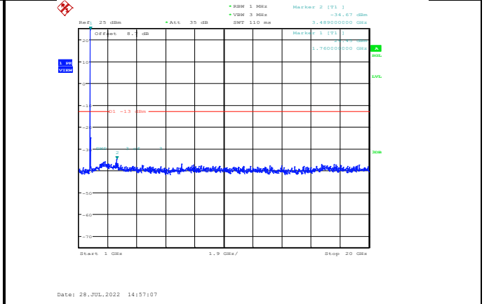
Band66-15MHz-16QAM-132597-1RB#0-Range2:1000~20000MHz
