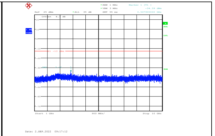
Band26-15MHz-64QAM-26915-1RB#0- Range2:1000~10000MHz
