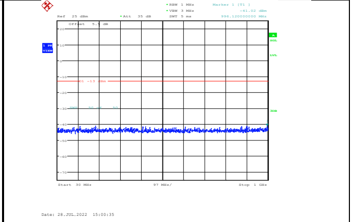
Band66-20MHz-16QAM-132572-1RB#0-Range1:30~1000MHz
