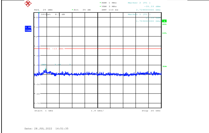
Band66-10MHz-16QAM-132022-1RB#0-Range2:1000~20000MHz
