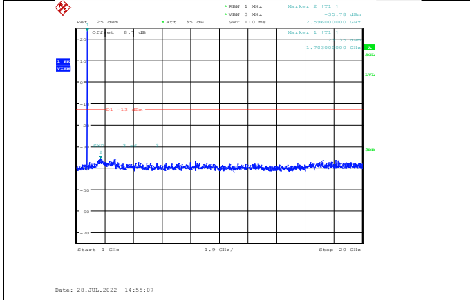
Band66-15MHz-16QAM-132047-1RB#0-Range2:1000~20000MHz
