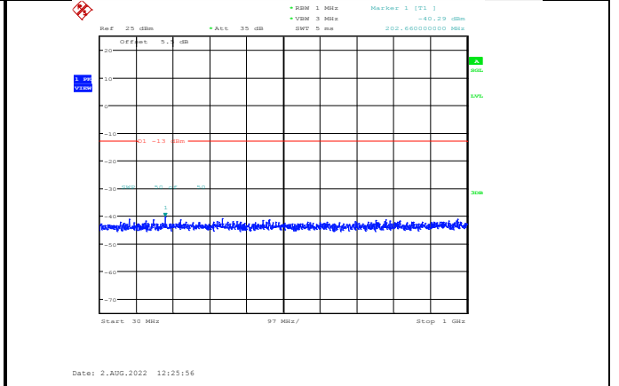
Band66-15MHz-64QAM-132597-1RB#0-Range1:30~1000MHz
