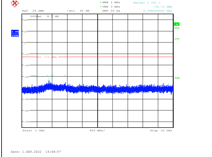
Band26-15MHz-QPSK-26765-1RB#0-Range2:1000~10000MHz
