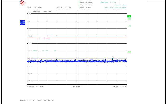
Band66-15MHz-16QAM-132597-1RB#0-Range1:30~1000MHz
