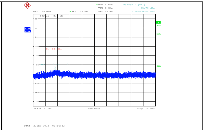
Band26-15MHz-16QAM-26915-1RB#0- Range2:1000~10000MHz
