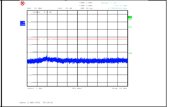
Band26-15MHz-64QAM-26965-1RB#0- Range2:1000~10000MHz
