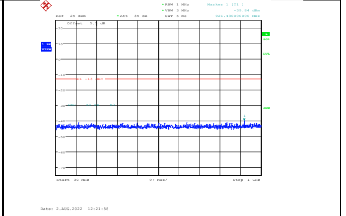
Band66-5MHz-64QAM-132647-1RB#0-Range1:30~1000MHz
