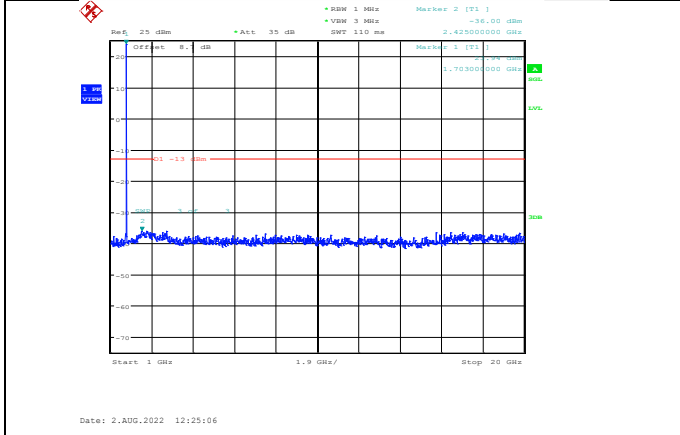
Band66-15MHz-64QAM-132047-1RB#0-Range2:1000~20000MHz
