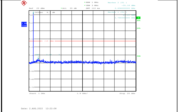
Band66-5MHz-64QAM-132647-1RB#0-Range2:1000~20000MHz
