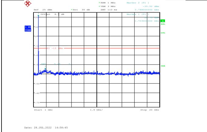
Band66-20MHz-16QAM-132072-1RB#0-Range2:1000~20000MHz
