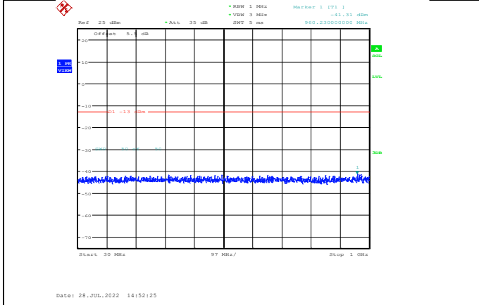
Band66-10MHz-16QAM-132322-1RB#0-Range1:30~1000MHz
