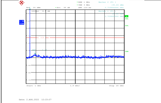
Band66-10MHz-64QAM-132022-1RB#0-Range2:1000~20000MHz
