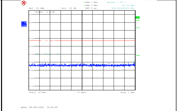
Band66-10MHz-QPSK-132622-1RB#0-Range1:30~1000MHz
