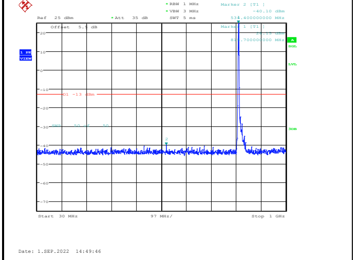
Band26-15MHz-64QAM-26765-1RB#0-Range1:30~1000MHz
