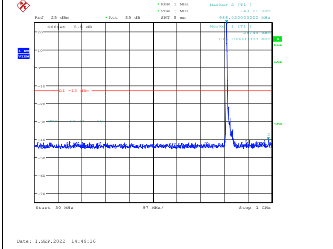
Band26-15MHz-16QAM-26765-1RB#0-Range1:30~1000MHz
