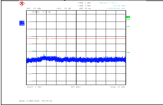
Band26-15MHz-16QAM-26865-1RB#0- Range2:1000~10000MHz
