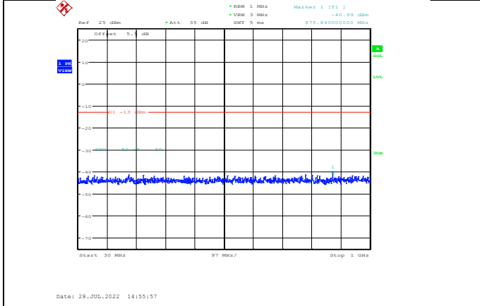
Band66-15MHz-16QAM-132322-1RB#0-Range1:30~1000MHz
