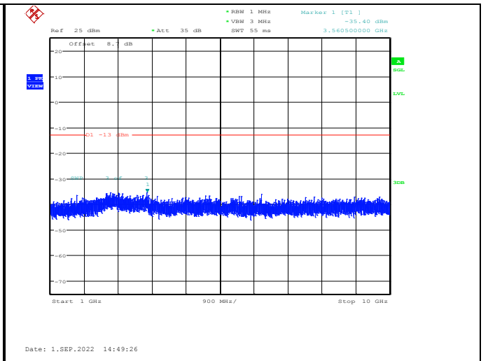
Band26-15MHz-16QAM-26765-1RB#0-Range2:1000~10000MHz
