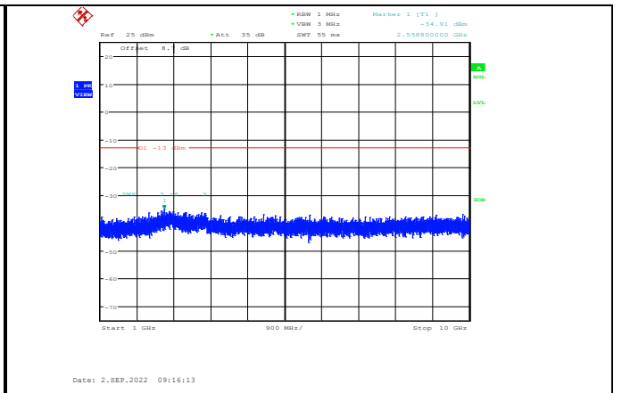
Band26-15MHz-QPSK-26915-1RB#0-Range2:1000~10000MHz
