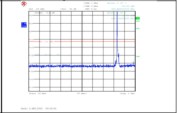
Band26-15MHz-16QAM-26965-1RB#0- Range1:30~1000MHz
