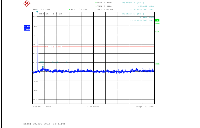
Band66-10MHz-QPSK-132022-1RB#0-Range2:1000~20000MHz
