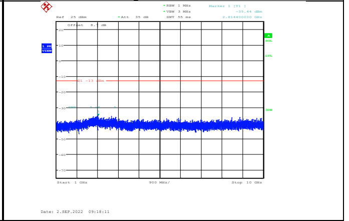
Band26-15MHz-16QAM-26965-1RB#0- Range2:1000~10000MHz
