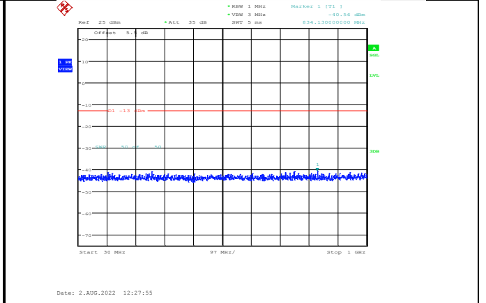
Band66-20MHz-64QAM-132572-1RB#0-Range1:30~1000MHz
