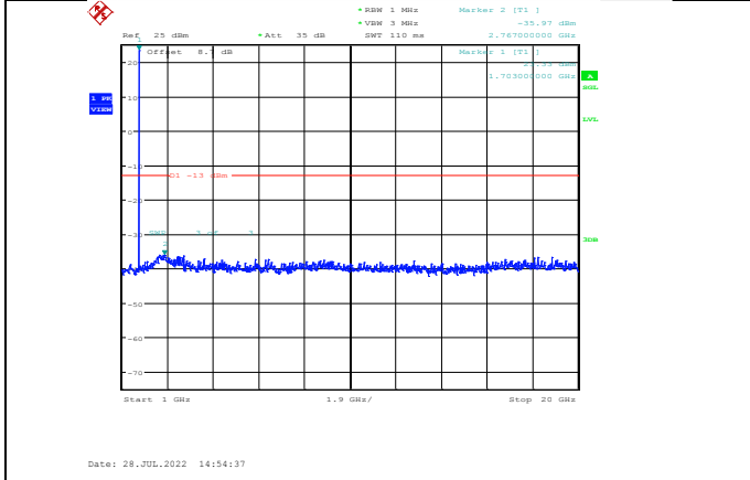
Band66-15MHz-QPSK-132047-1RB#0-Range2:1000~20000MHz
