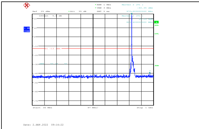
Band26-15MHz-QPSK-26865-1RB#0-Range1:30~1000MHz
