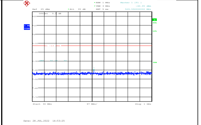
Band66-10MHz-16QAM-132622-1RB#0-Range1:30~1000MHz
