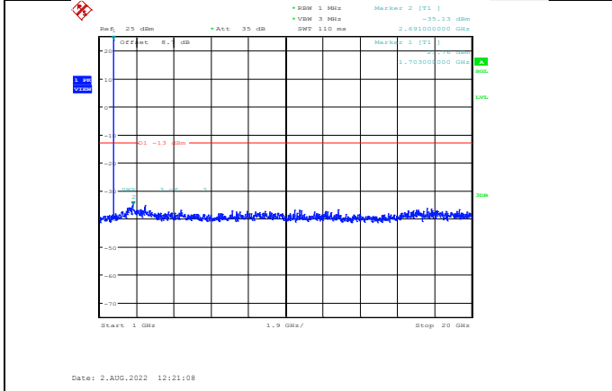
Band66-5MHz-64QAM-131997-1RB#0-Range2:1000~20000MHz
