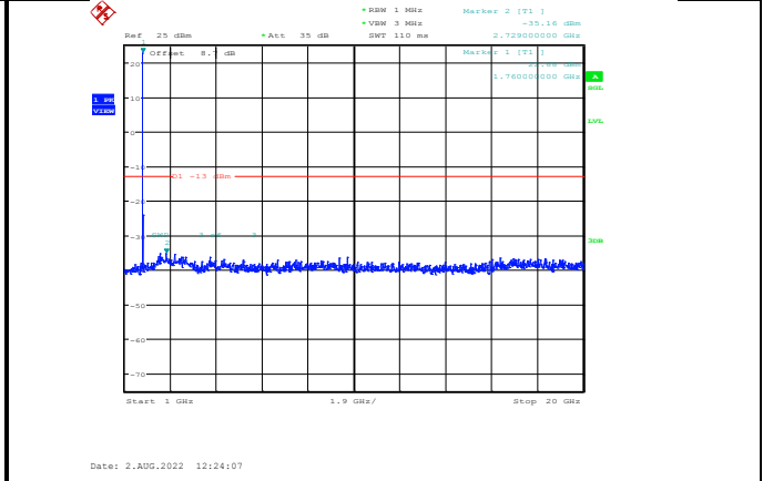
Band66-10MHz-64QAM-132622-1RB#0-Range2:1000~20000MHz
