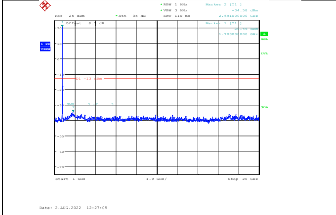
Band66-20MHz-64QAM-132072-1RB#0-Range2:1000~20000MHz
