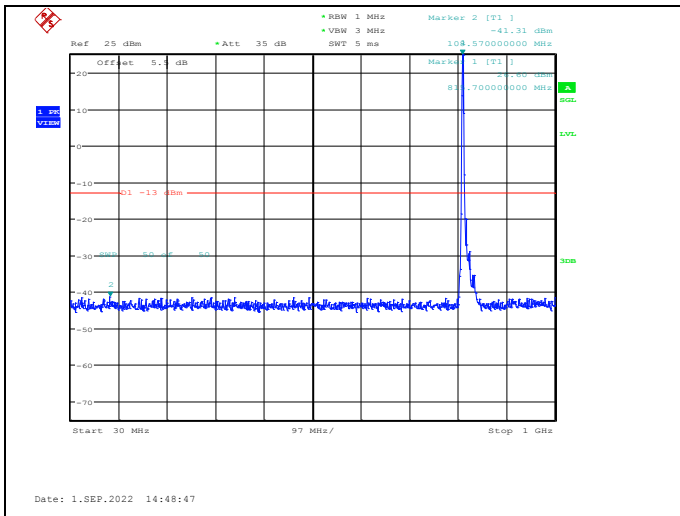
Band26-15MHz-QPSK-26765-1RB#0-Range1:30~1000MHz
