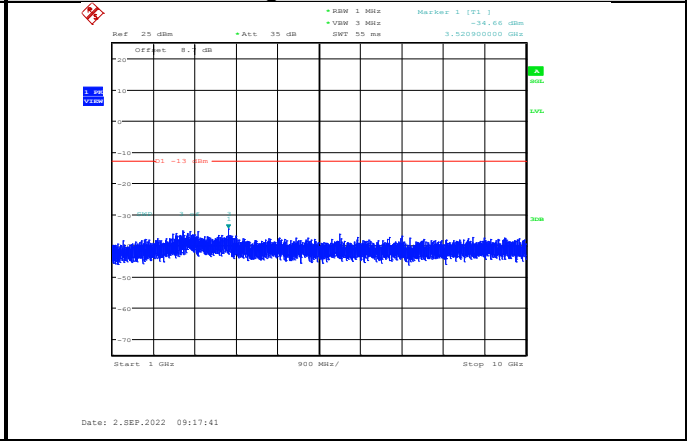
Band26-15MHz-QPSK-26965-1RB#0-Range2:1000~10000MHz
