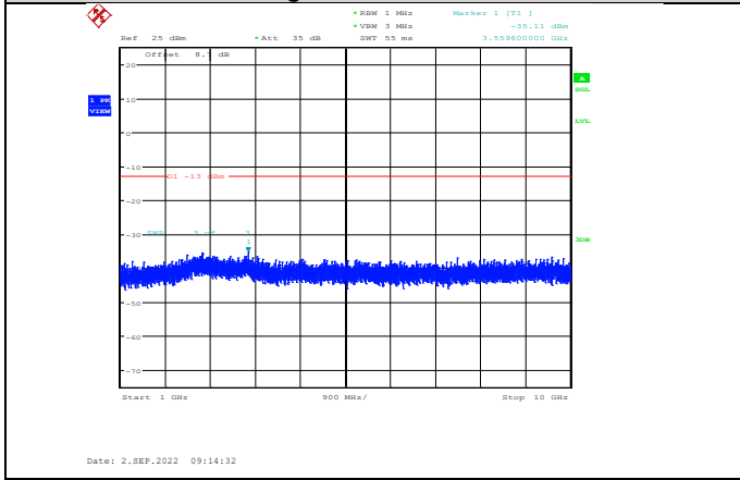
Band26-15MHz-QPSK-26865-1RB#0-Range2:1000~10000MHz
