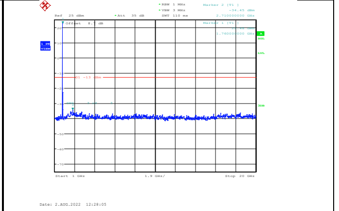
Band66-20MHz-64QAM-132572-1RB#0-Range2:1000~20000MHz
