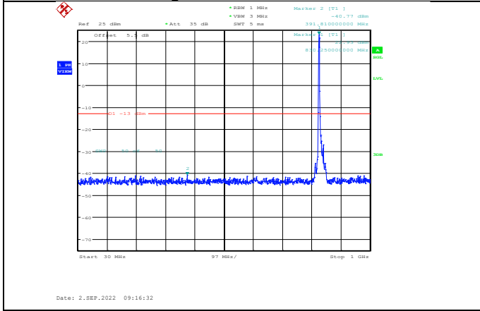
Band26-15MHz-16QAM-26915-1RB#0- Range1:30~1000MHz
