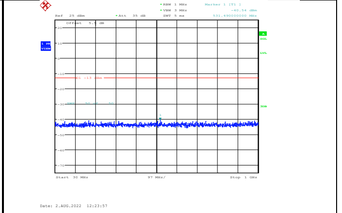
Band66-10MHz-64QAM-132622-1RB#0-Range1:30~1000MHz
