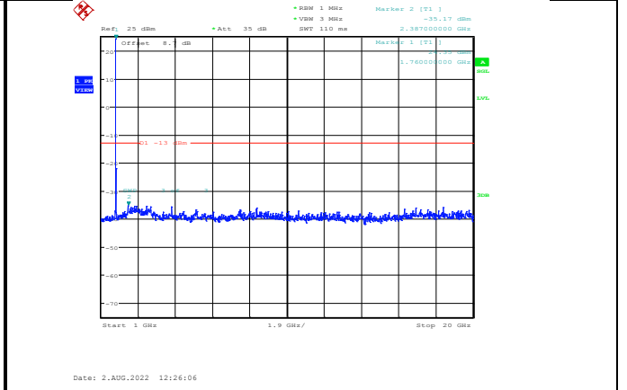
Band66-15MHz-64QAM-132597-1RB#0-Range2:1000~20000MHz
