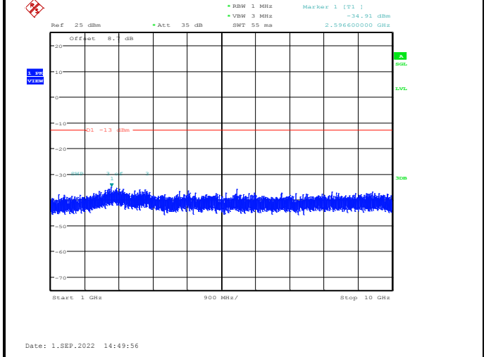
Band26-15MHz-64QAM-26765-1RB#0-Range2:1000~10000MHz
