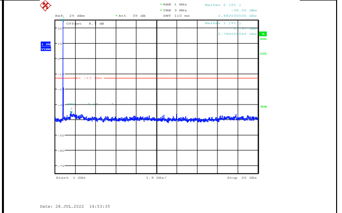
Band66-10MHz-16QAM-132622-1RB#0-Range2:1000~20000MHz
