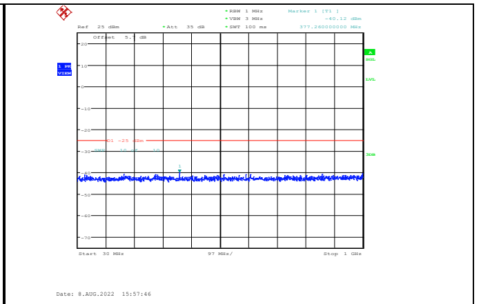
Band38-20MHz-16QAM-38000-1RB#0- Range1:30~1000MHz
