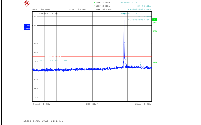
Band41-10MHz-64QAM-40090-1RB#0-Range2:1000~3000MHz
