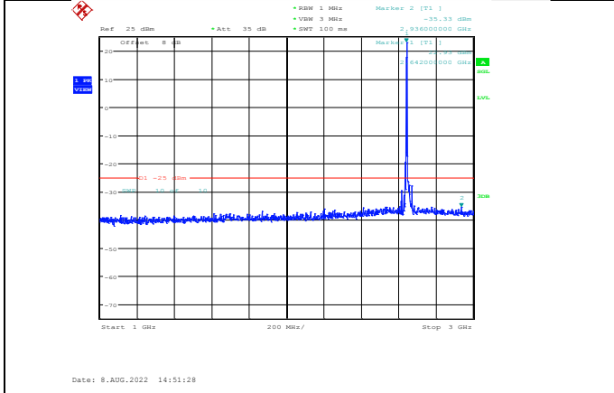
Band41-15MHz-64QAM-41165-1RB#0-Range2:1000~3000MHz
