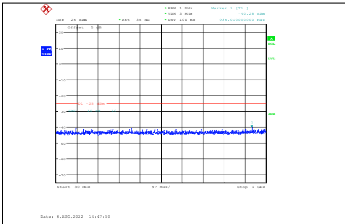
Band41-10MHz-64QAM-40590-1RB#0-Range1:30~1000MHz
