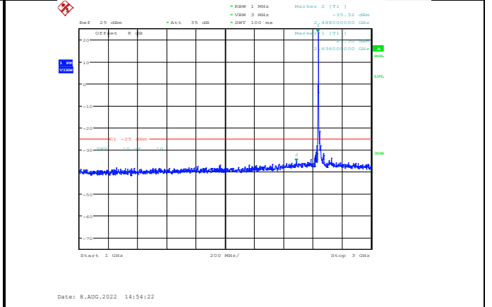
Band41-20MHz-64QAM-41140-1RB#0-Range2:1000~3000MHz
