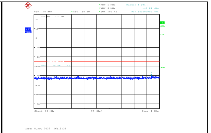
Band41-15MHz-QPSK-40590-1RB#0- Range1:30~1000MHz
