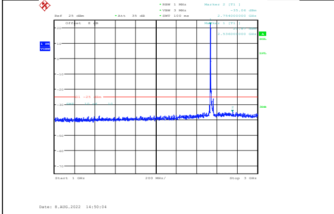
Band41-15MHz-64QAM-40115-1RB#0-Range2:1000~3000MHz
