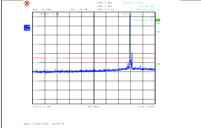
Band38-20MHz-64QAM-38000-1RB#0-Range2:1000~3000MHz
