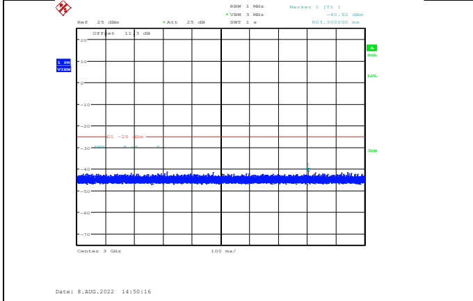
Band41-15MHz-64QAM-40115-1RB#0-Range3:3000~27000MHz
