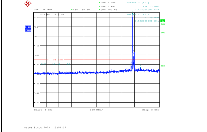
Band38-15MHz-QPSK-37825-1RB#0-Range2:1000~3000MHz
