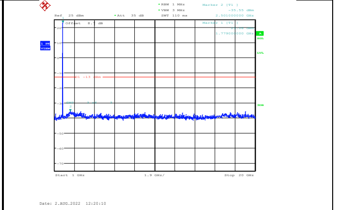
Band66-3MHz-64QAM-132657-1RB#0-Range2:1000~20000MHz
