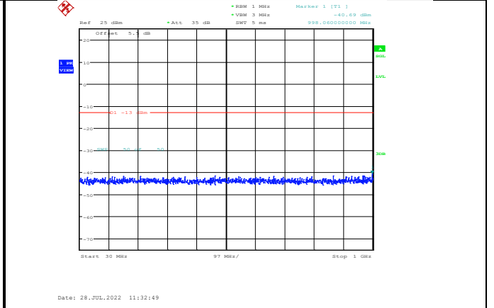
Band66-1.4MHz-16QAM-132665-1RB#0-Range1:30~1000MHz
