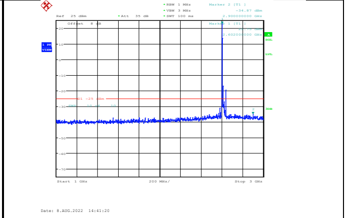
Band38-20MHz-64QAM-38150-1RB#0-Range2:1000~3000MHz
