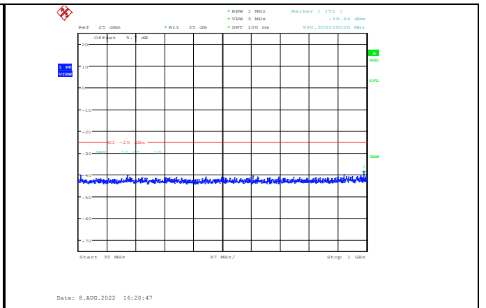
Band41-20MHz-16QAM-40590-1RB#0- Range1:30~1000MHz
