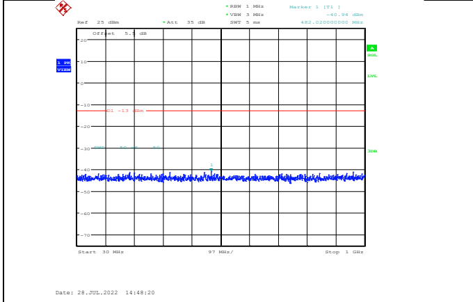
Band66-5MHz-16QAM-132322-1RB#0-Range1:30~1000MHz
