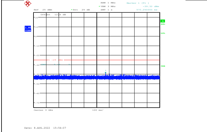
Band38-15MHz-QPSK-38175-1RB#0-Range3:3000~27000MHz
