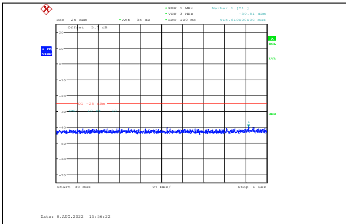
Band38-20MHz-16QAM-37850-1RB#0- Range1:30~1000MHz
