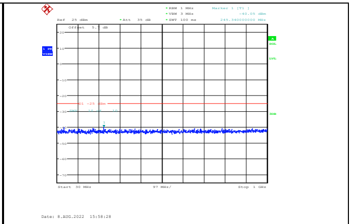
Band38-20MHz-QPSK-38150-1RB#0-Range1:30~1000MHz
