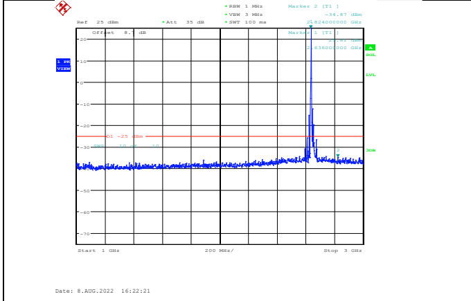
Band41-20MHz-16QAM-41140-1RB#0-Range2:1000~3000MHz
