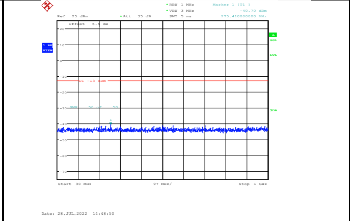
Band66-5MHz-QPSK-132647-1RB#0-Range1:30~1000MHz
