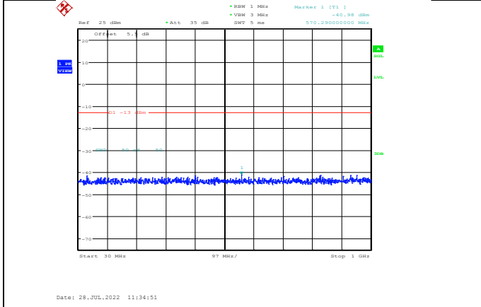
Band66-3MHz-QPSK-132322-1RB#0-Range1:30~1000MHz
