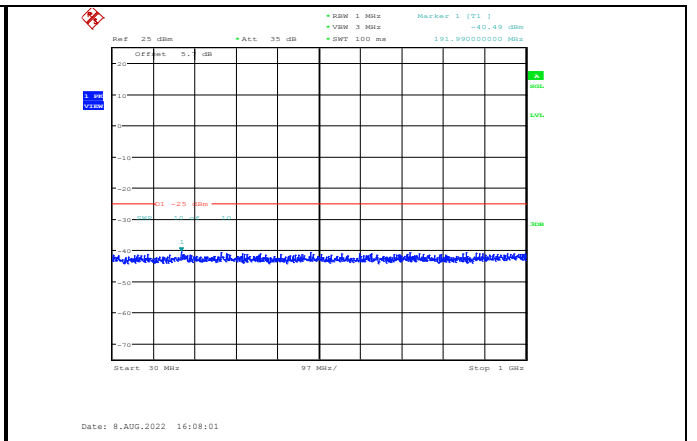
Band41-5MHz-16QAM-41215-1RB#0-Range1:30~1000MHz
