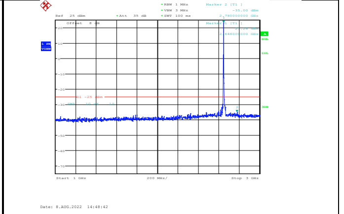
Band41-10MHz-64QAM-41190-1RB#0-Range2:1000~3000MHz
