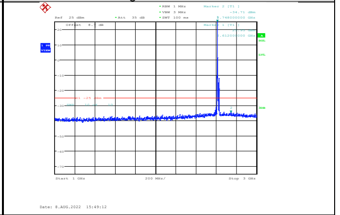
Band38-10MHz-QPSK-38200-1RB#0-Range2:1000~3000MHz
