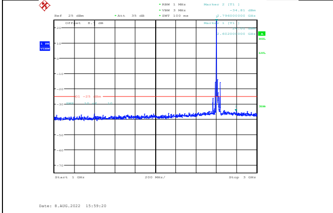
Band38-20MHz-16QAM-38150-1RB#0-Range2:1000~3000MHz
