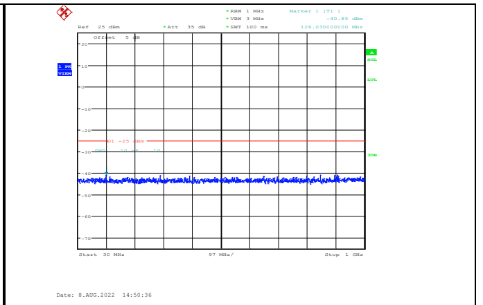
Band41-15MHz-64QAM-40590-1RB#0-Range1:30~1000MHz
