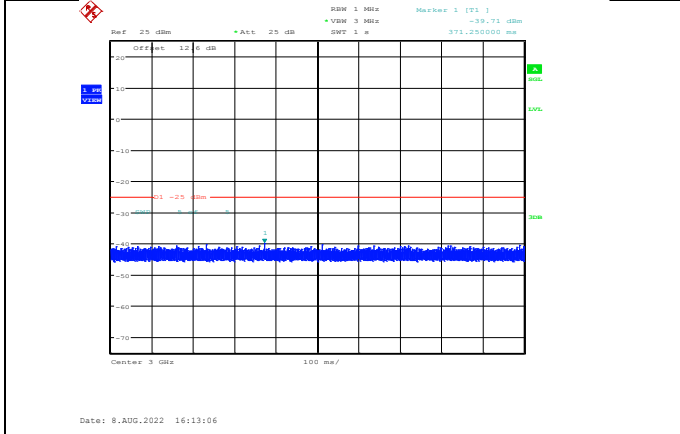
Band41-10MHz-16QAM-41190-1RB#0-Range3:3000~27000MHz
