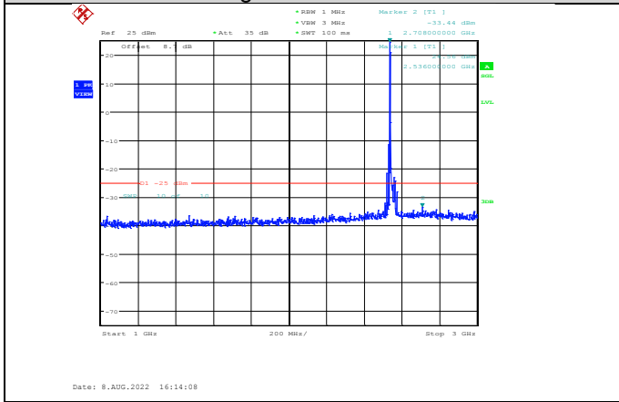
Band41-15MHz-QPSK-40115-1RB#0- Range2:1000~3000MHz
