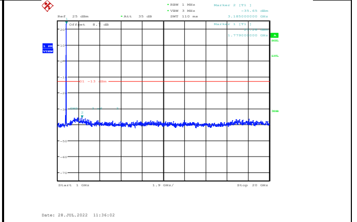
Band66-3MHz-QPSK-132657-1RB#0-Range2:1000~20000MHz
