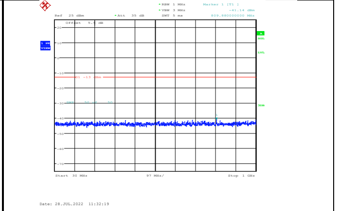
Band66-1.4MHz-QPSK-132665-1RB#0- Range1:30~1000MHz
