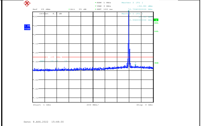
Band38-10MHz-16QAM-38000-1RB#0-Range2:1000~3000MHz
