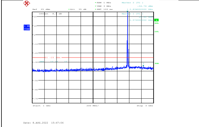
Band38-10MHz-16QAM-37800-1RB#0-Range2:1000~3000MHz
