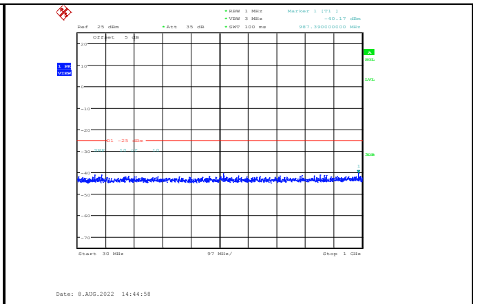
Band41-5MHz-64QAM-40590-1RB#0-Range1:30~1000MHz
