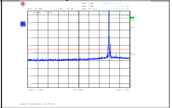
Band38-20MHz-16QAM-38000-1RB#0- Range2:1000~3000MHz
