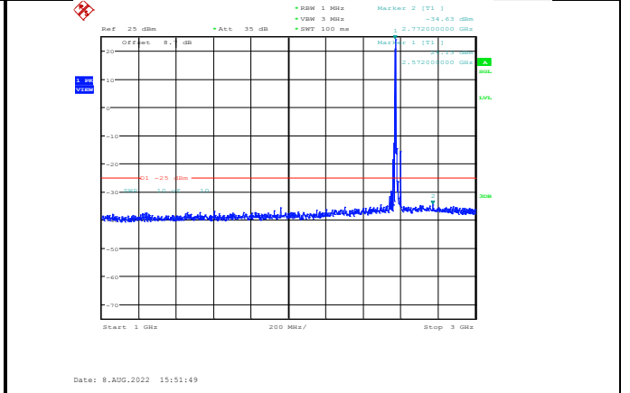
Band38-15MHz-16QAM-37825-1RB#0-Range2:1000~3000MHz
