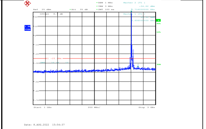
Band38-15MHz-16QAM-38175-1RB#0-Range2:1000~3000MHz
