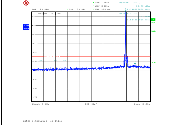
Band41-15MHz-16QAM-40590-1RB#0-Range2:1000~3000MHz
