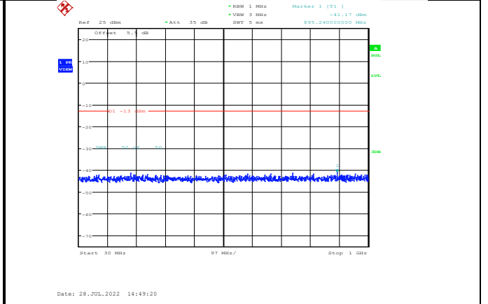
Band66-5MHz-16QAM-132647-1RB#0-Range1:30~1000MHz
