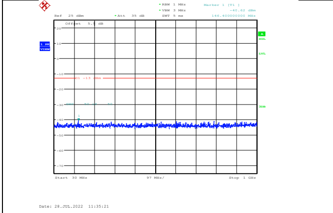
Band66-3MHz-16QAM-132322-1RB#0-Range1:30~1000MHz
