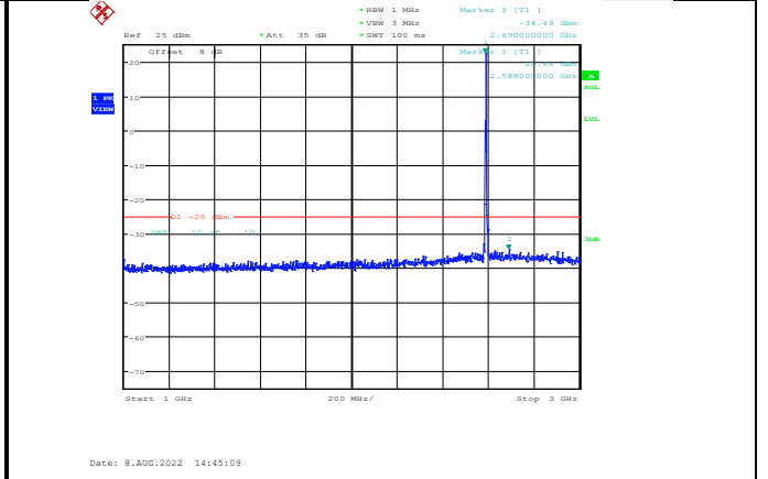
Band41-5MHz-64QAM-40590-1RB#0-Range2:1000~3000MHz
