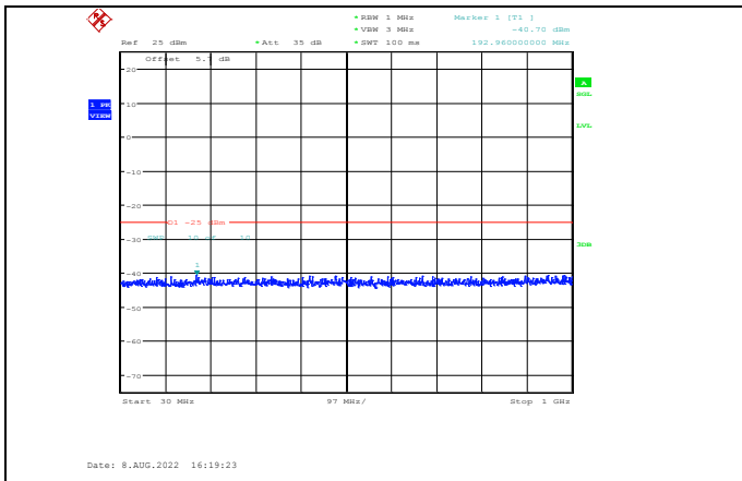
Band41-20MHz-16QAM-40140-1RB#0- Range1:30~1000MHz
