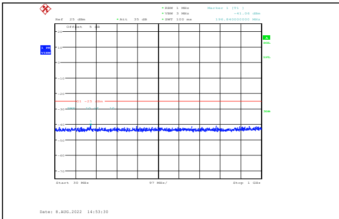
Band41-20MHz-64QAM-40590-1RB#0-Range1:30~1000MHz
