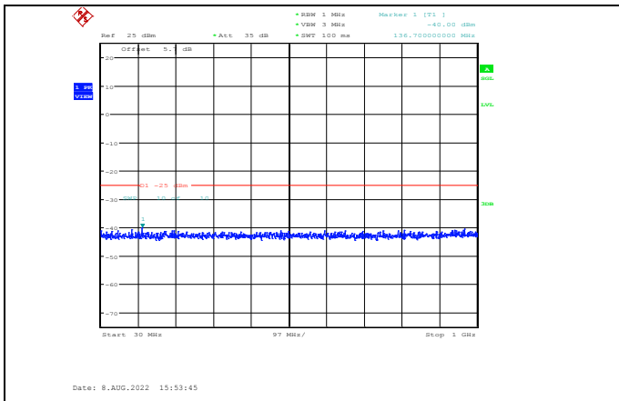
Band38-15MHz-QPSK-38175-1RB#0-Range1:30~1000MHz
