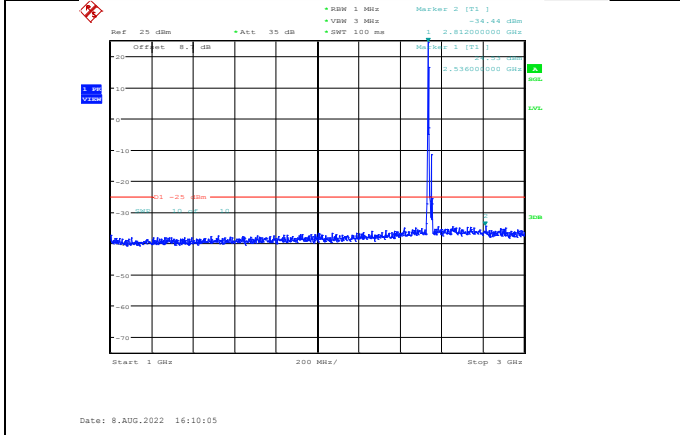
Band41-10MHz-16QAM-40090-1RB#0-Range2:1000~3000MHz
