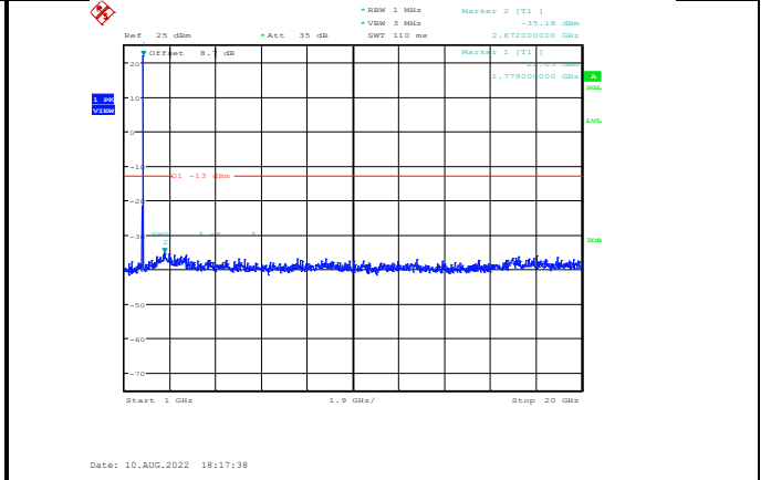
Band66-1.4MHz-64QAM-132665-1RB#0-Range2:1000~20000MHz
