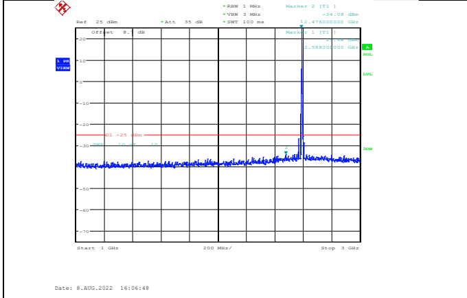
Band41-5MHz-16QAM-40590-1RB#0-Range2:1000~3000MHz
