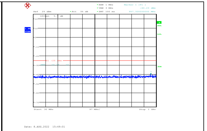
Band38-10MHz-QPSK-38200-1RB#0-Range1:30~1000MHz
