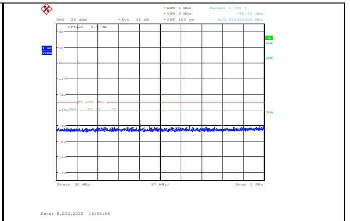
Band41-5MHz-QPSK-40590-1RB#0-Range1:30~1000MHz
