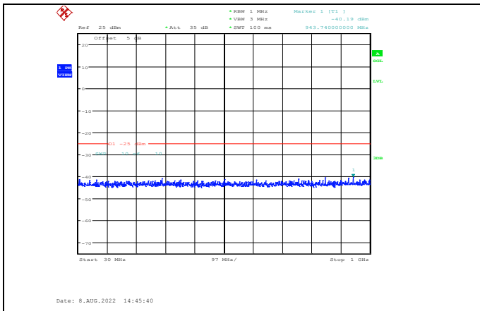
Band41-5MHz-64QAM-41215-1RB#0-Range1:30~1000MHz
