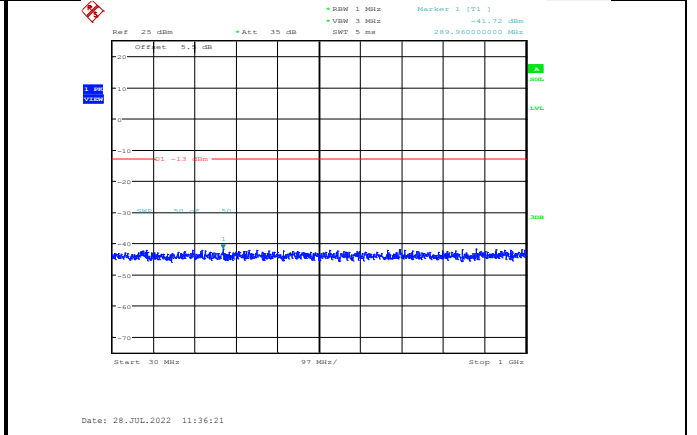
Band66-3MHz-16QAM-132657-1RB#0-Range1:30~1000MHz
