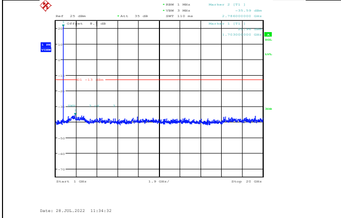
Band66-3MHz-16QAM-131987-1RB#0-Range2:1000~20000MHz
