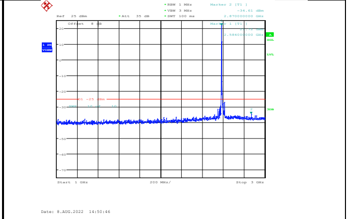
Band41-15MHz-64QAM-40590-1RB#0-Range2:1000~3000MHz
