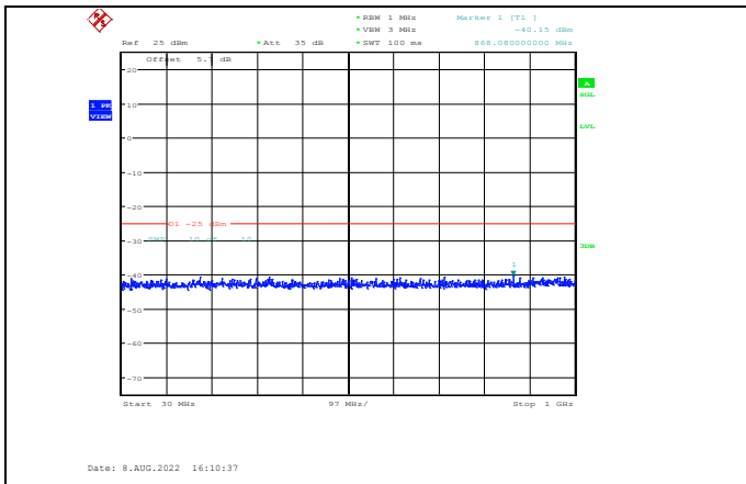
Band41-10MHz-QPSK-40590-1RB#0-Range1:30~1000MHz
