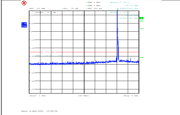
Band38-10MHz-16QAM-38200-1RB#0-Range2:1000~3000MHz
