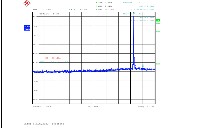
Band41-5MHz-64QAM-41215-1RB#0-Range2:1000~3000MHz
