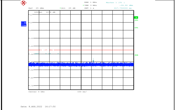
Band41-15MHz-16QAM-41165-1RB#0-Range3:3000~27000MHz
