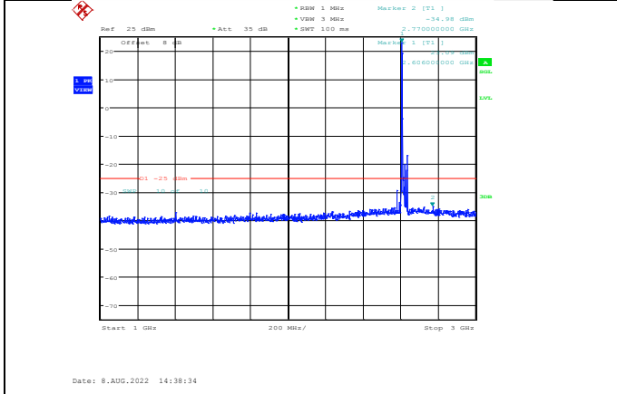
Band38-15MHz-64QAM-38175-1RB#0-Range2:1000~3000MHz
