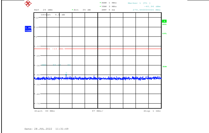
Band66-1.4MHz-16QAM-132322-1RB#0-Range1:30~1000MHz
