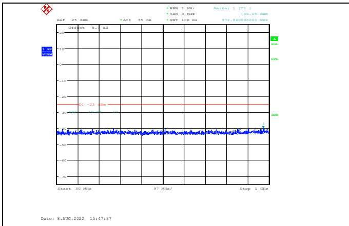
Band38-10MHz-QPSK-38000-1RB#0-Range1:30~1000MHz
