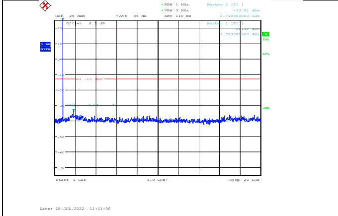
Band66-1.4MHz-16QAM-131979-1RB#0-Range2:1000~20000MHz
