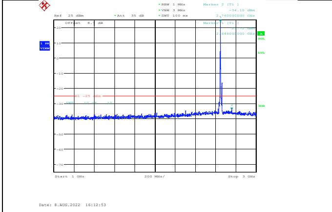
Band41-10MHz-16QAM-41190-1RB#0-Range2:1000~3000MHz
