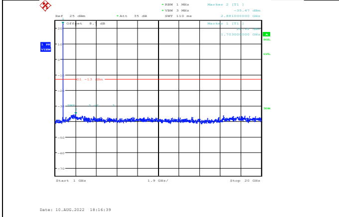
Band66-1.4MHz-64QAM-131979-1RB#0-Range2:1000~20000MHz
