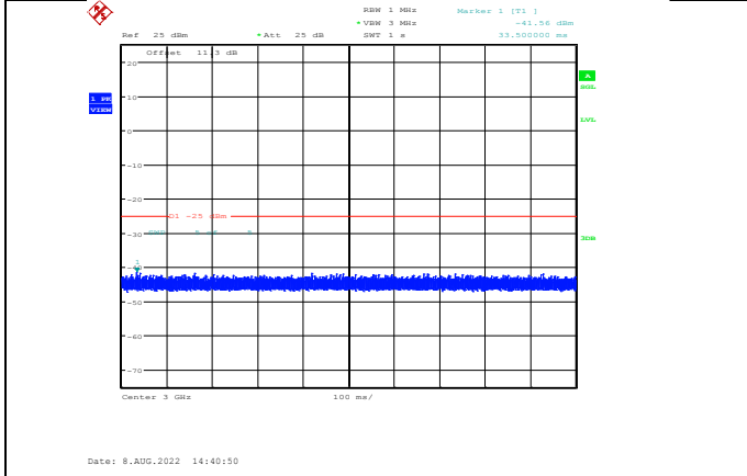
Band38-20MHz-64QAM-38000-1RB#0-Range3:3000~27000MHz
