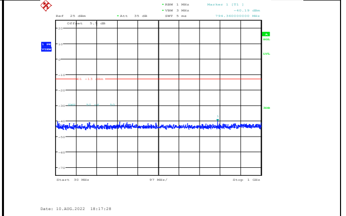
Band66-1.4MHz-64QAM-132665-1RB#0-Range1:30~1000MHz
