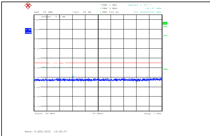
Band41-5MHz-16QAM-40590-1RB#0-Range1:30~1000MHz
