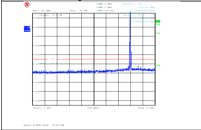
Band38-10MHz-QPSK-38000-1RB#0-Range2:1000~3000MHz
