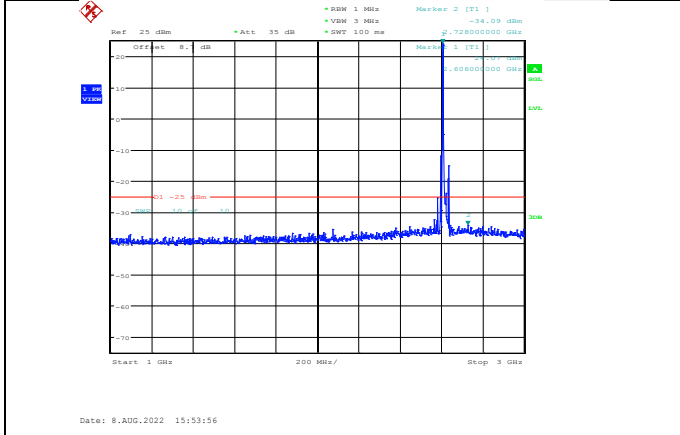
Band38-15MHz-QPSK-38175-1RB#0-Range2:1000~3000MHz
