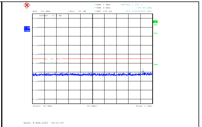
Band41-10MHz-16QAM-40590-1RB#0-Range1:30~1000MHz
