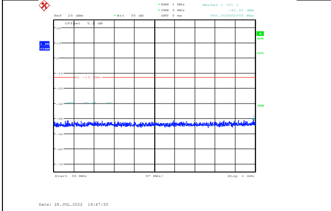
Band66-5MHz-QPSK-132322-1RB#0-Range1:30~1000MHz
