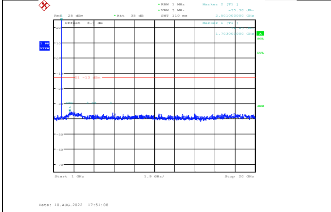
Band66-1.4MHz-QPSK-131979-1RB#0- Range2:1000~20000MHz
