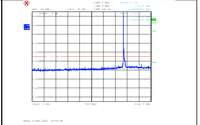
Band41-20MHz-64QAM-40140-1RB#0-Range2:1000~3000MHz
