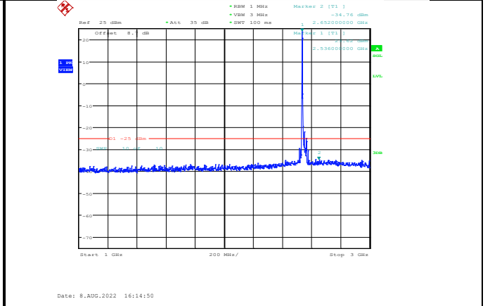
Band41-15MHz-16QAM-40115-1RB#0-Range2:1000~3000MHz
