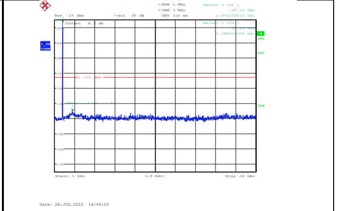
Band66-5MHz-QPSK-132647-1RB#0-Range2:1000~20000MHz
