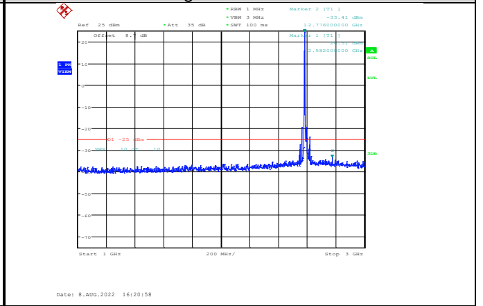
Band41-20MHz-16QAM-40590-1RB#0- Range2:1000~3000MHz
