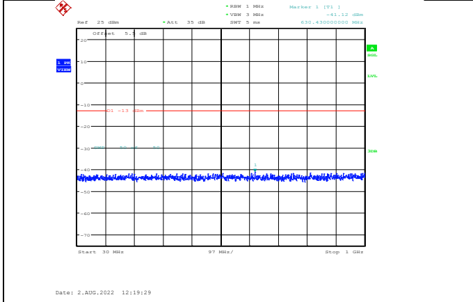
Band66-3MHz-64QAM-132322-1RB#0-Range1:30~1000MHz
