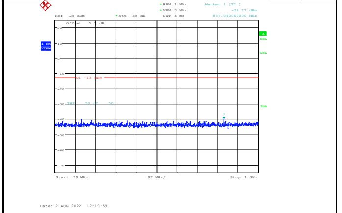
Band66-3MHz-64QAM-132657-1RB#0-Range1:30~1000MHz
