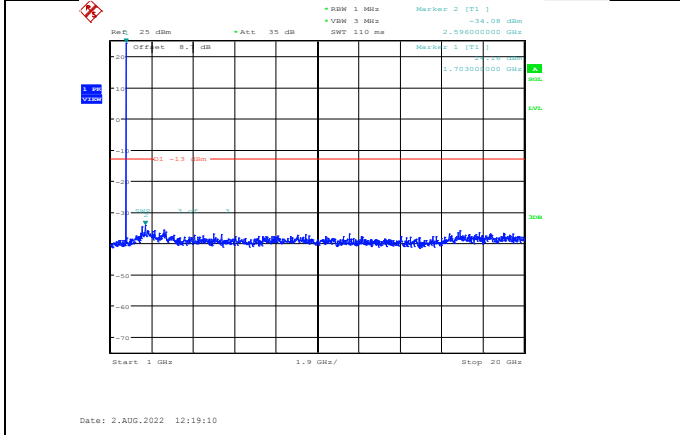
Band66-3MHz-64QAM-131987-1RB#0-Range2:1000~20000MHz
