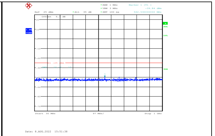
Band38-15MHz-16QAM-37825-1RB#0-Range1:30~1000MHz
