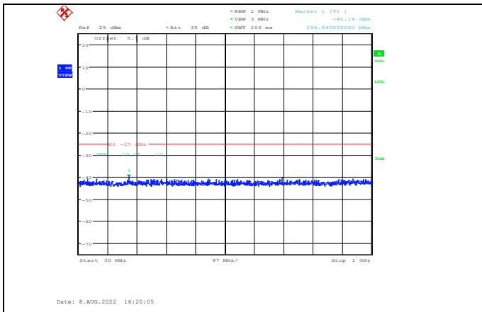
Band41-20MHz-QPSK-40590-1RB#0-Range1:30~1000MHz
