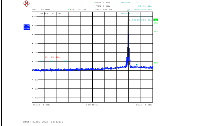
Band38-15MHz-16QAM-38000-1RB#0-Range2:1000~3000MHz
