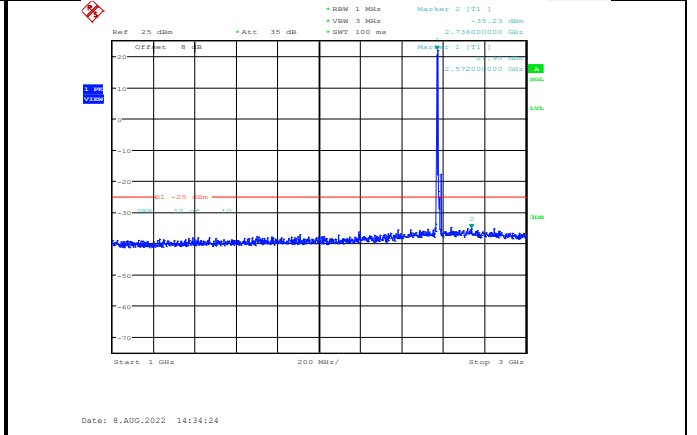
Band38-10MHz-64QAM-37800-1RB#0-Range2:1000~3000MHz
