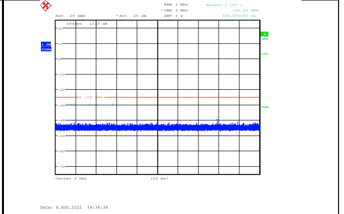
Band38-10MHz-64QAM-37800-1RB#0-Range3:3000~27000MHz
