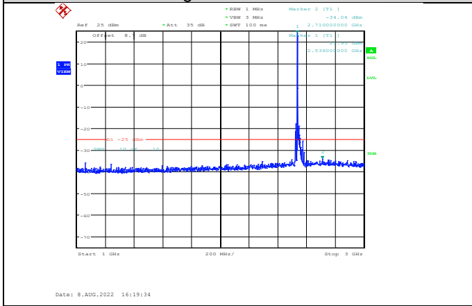
Band41-20MHz-16QAM-40140-1RB#0- Range2:1000~3000MHz
