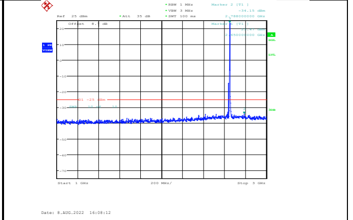
Band41-5MHz-16QAM-41215-1RB#0-Range2:1000~3000MHz
