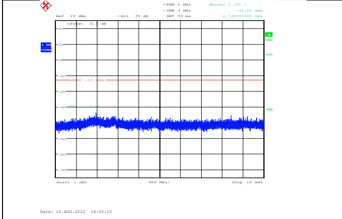
Band12-5MHz-64QAM-23035-1RB#0-Range2:1000~10000MHz
