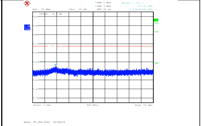
Band12-5MHz-16QAM-23155-1RB#0-Range2:1000~10000MHz
