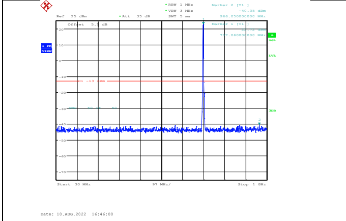
Band12-3MHz-64QAM-23095-1RB#0-Range1:30~1000MHz
