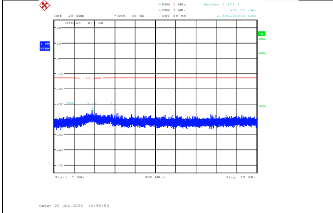
Band12-5MHz-QPSK-23035-1RB#0-Range2:1000~10000MHz
