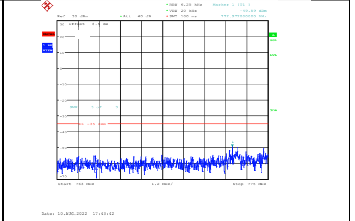
Band13-10MHz-QPSK-23230-1RB#0-Range3:763~775MHz
