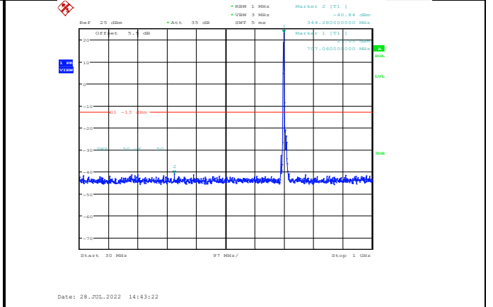
Band17-10MHz-16QAM-23800-1RB#0- Range1:30~1000MHz
