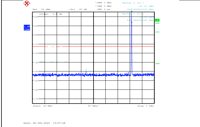
Band26-1.4MHz-16QAM-26740-1RB#0- Range1:30~1000MHz
