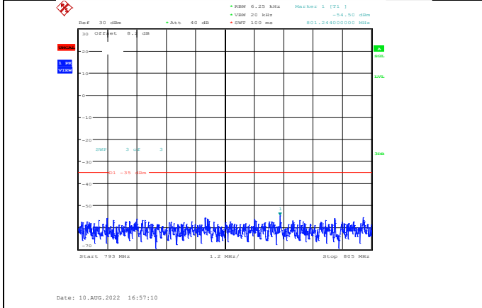
Band13-5MHz-64QAM-23230-1RB#0-Range4:793~805MHz
