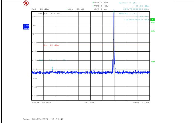
Band12-5MHz-QPSK-23095-1RB#0-Range1:30~1000MHz
