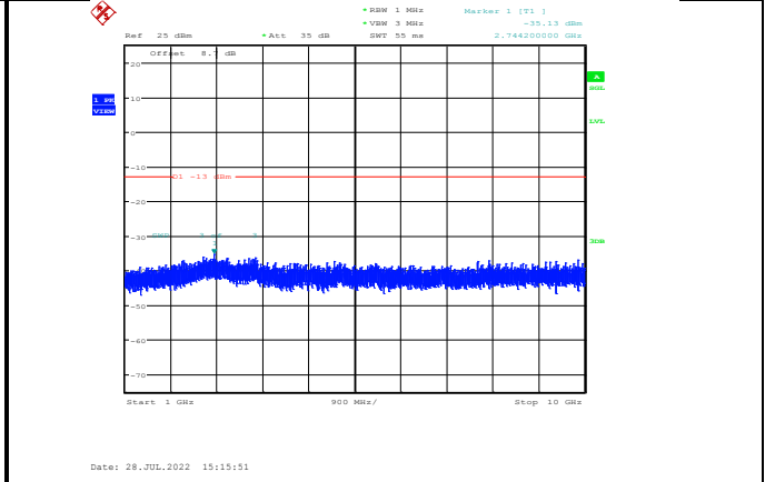
Band26-5MHz-16QAM-26765-1RB#0-Range2:1000~10000MHz
