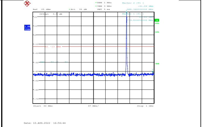
Band13-5MHz-64QAM-23230-1RB#0-Range1:30~1000MHz
