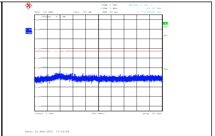
Band26-5MHz-64QAM-26740-1RB#0-Range2:1000~10000MHz
