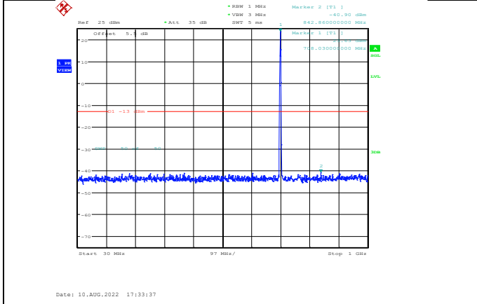
Band12-1.4MHz-QPSK-23095-1RB#0-Range1:30~1000MHz
