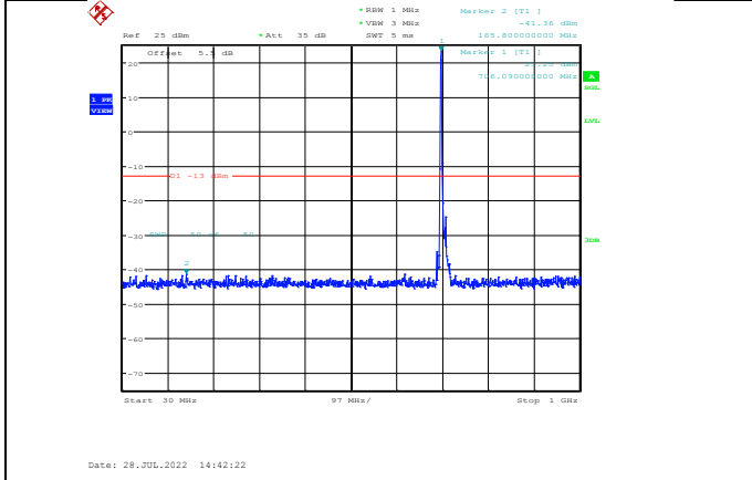
Band17-10MHz-16QAM-23790-1RB#0- Range1:30~1000MHz
