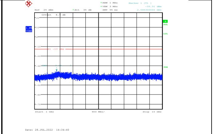
Band12-10MHz-16QAM-23130-1RB#0- Range2:1000~10000MHz
