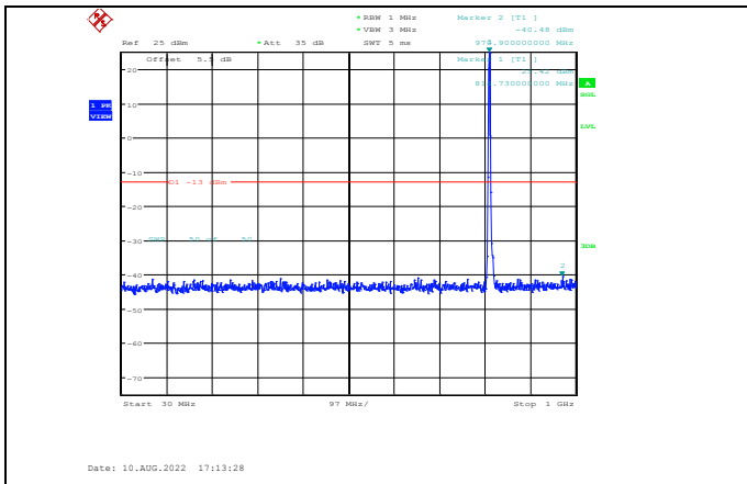
Band26-5MHz-64QAM-26715-1RB#0-Range1:30~1000MHz
