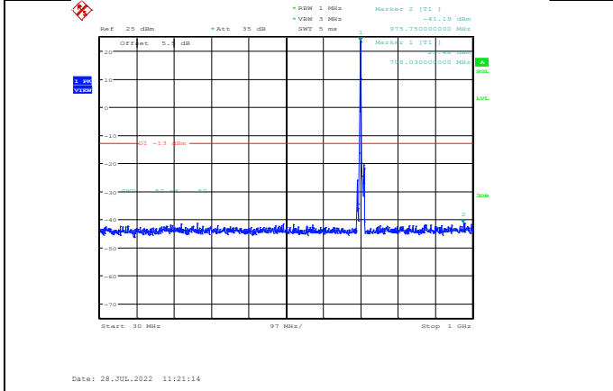
Band17-5MHz-QPSK-23790-1RB#0-Range1:30~1000MHz
