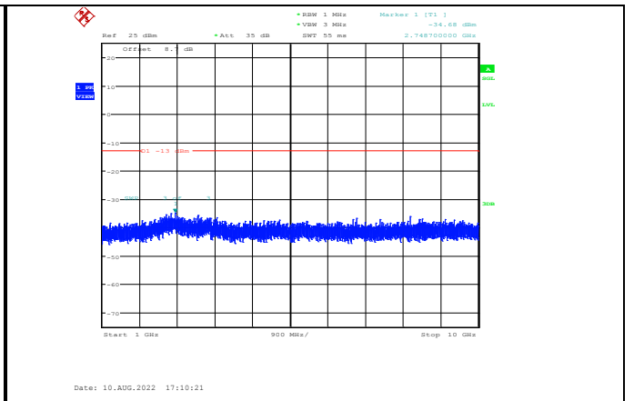
Band26-3MHz-64QAM-26740-1RB#0-Range2:1000~10000MHz
