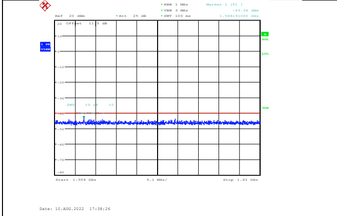
Band13-5MHz-16QAM-23205-1RB#0-Range5:1559~1610MHz
