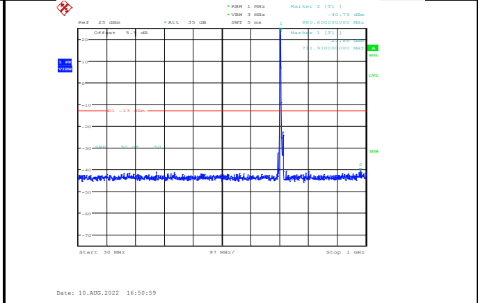
Band12-5MHz-64QAM-23155-1RB#0-Range1:30~1000MHz
