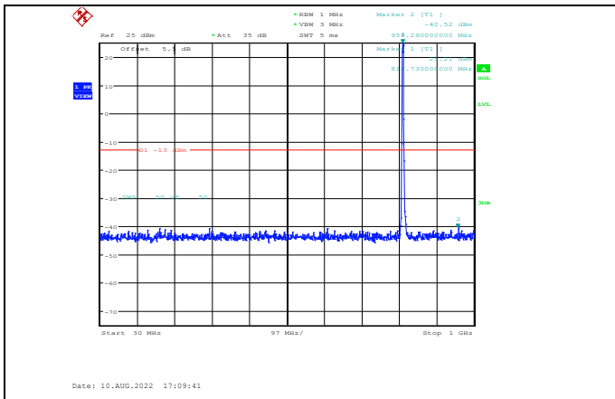
Band26-3MHz-64QAM-26705-1RB#0-Range1:30~1000MHz
