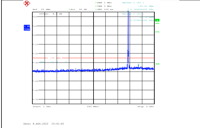
Band38-5MHz-QPSK-37775-1RB#0-Range2:1000~3000MHz
