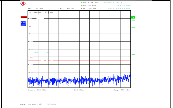
Band13-5MHz-16QAM-23205-1RB#0-Range3:763~775MHz
