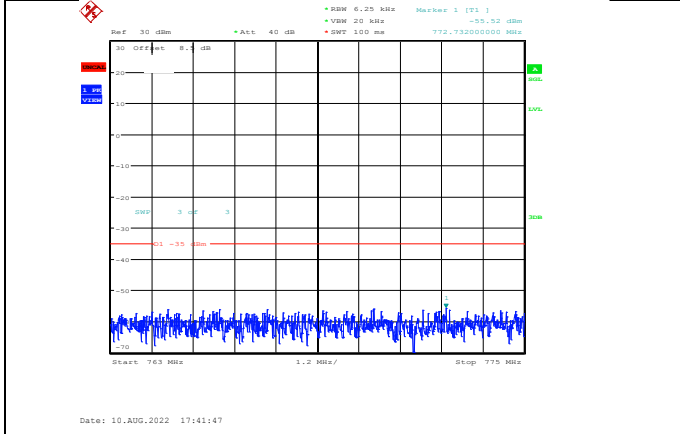
Band13-5MHz-16QAM-23255-1RB#0-Range3:763~775MHz
