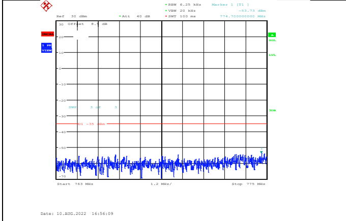
Band13-5MHz-64QAM-23205-1RB#0-Range3:763~775MHz
