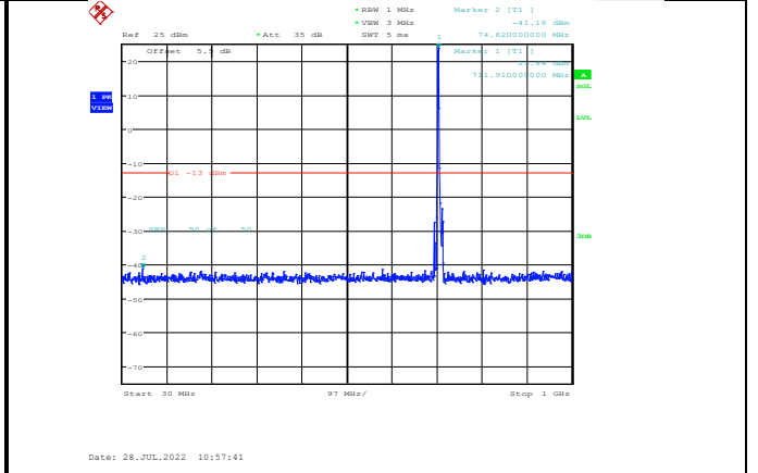
Band12-5MHz-QPSK-23155-1RB#0-Range1:30~1000MHz
