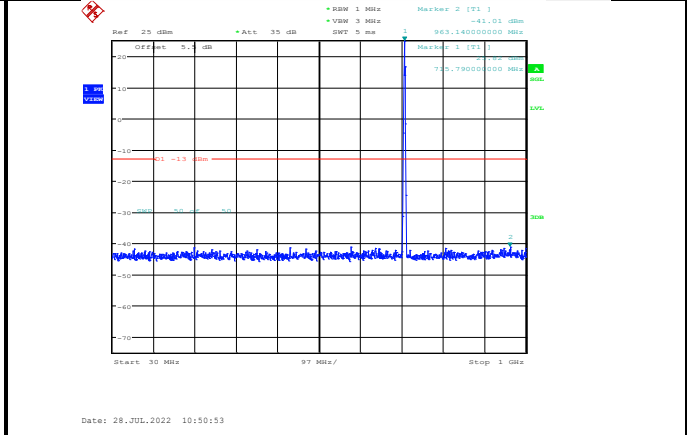
Band12-1.4MHz-16QAM-23173-1RB#0- Range1:30~1000MHz
