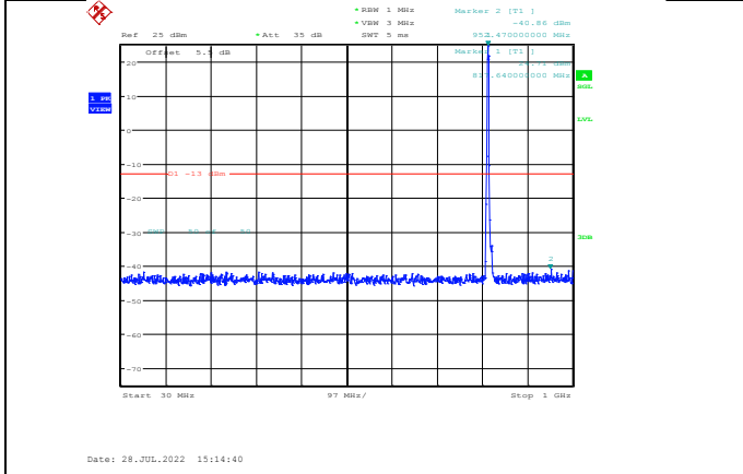
Band26-5MHz-16QAM-26740-1RB#0-Range1:30~1000MHz
