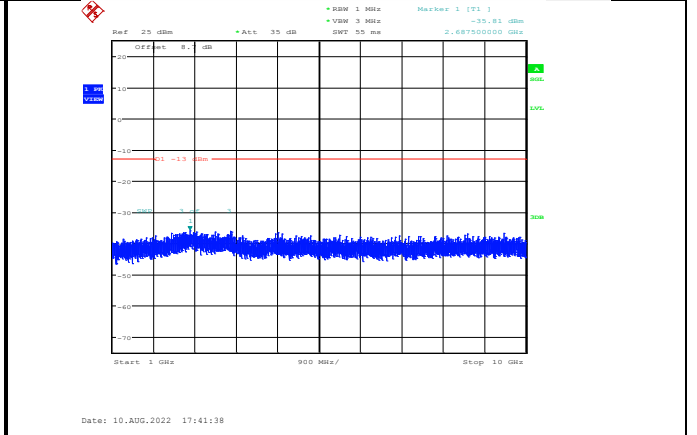
Band13-5MHz-16QAM-23255-1RB#0-Range2:1000~10000MHz
