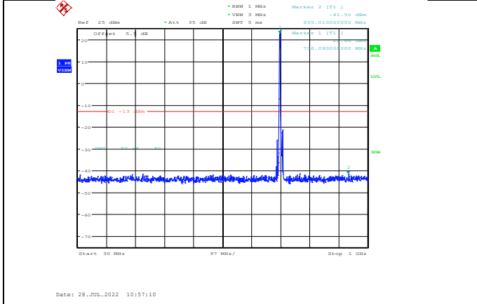
Band12-5MHz-16QAM-23095-1RB#0-Range1:30~1000MHz
