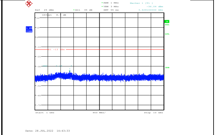
Band17-10MHz-16QAM-23800-1RB#0- Range2:1000~10000MHz
