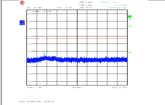
Band12-3MHz-64QAM-23025-1RB#0-Range2:1000~10000MHz
