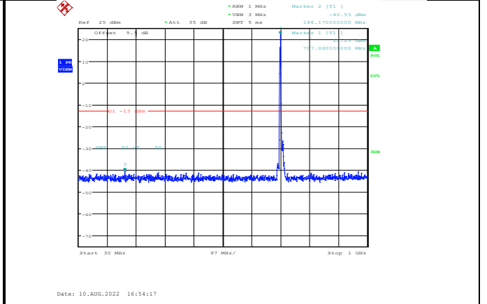
Band12-10MHz-64QAM-23130-1RB#0- Range1:30~1000MHz
