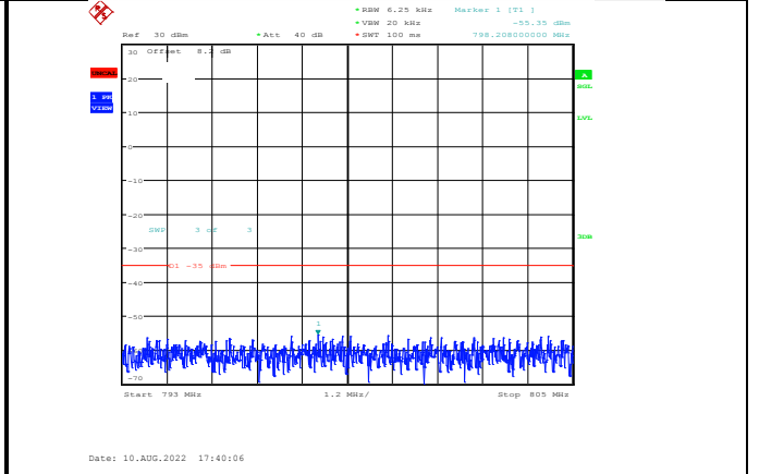
Band13-5MHz-16QAM-23230-1RB#0-Range4:793~805MHz
