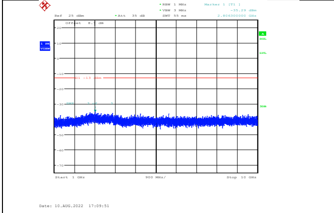
Band26-3MHz-64QAM-26705-1RB#0-Range2:1000~10000MHz
