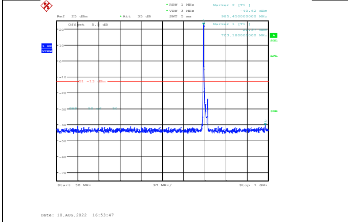
Band12-10MHz-64QAM-23095-1RB#0- Range1:30~1000MHz
