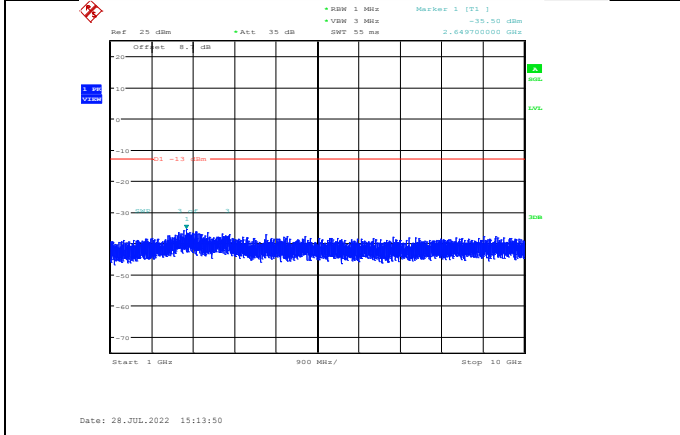
Band26-5MHz-16QAM-26715-1RB#0-Range2:1000~10000MHz
