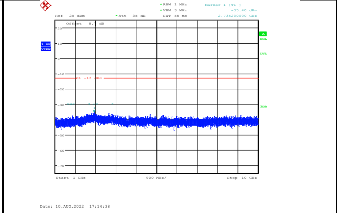
Band26-5MHz-64QAM-26765-1RB#0-Range2:1000~10000MHz
