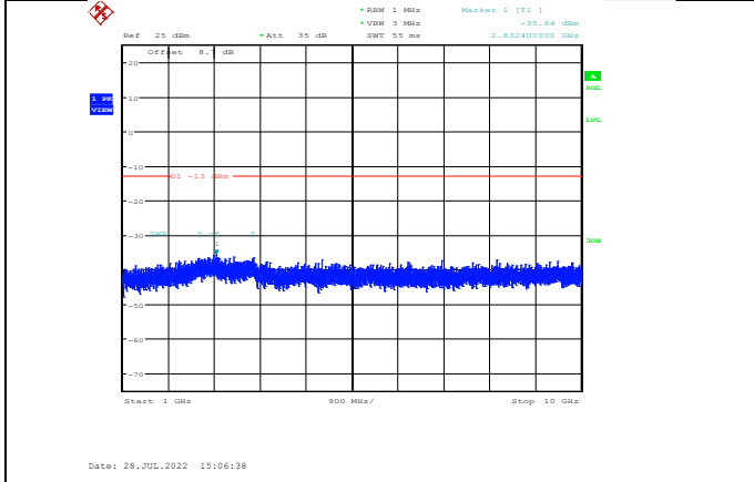
Band26-1.4MHz-16QAM-26697-1RB#0- Range2:1000~10000MHz
