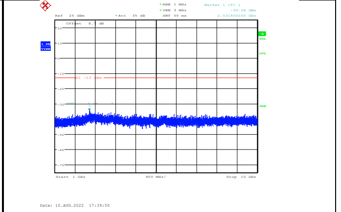
Band13-5MHz-16QAM-23230-1RB#0-Range2:1000~10000MHz
