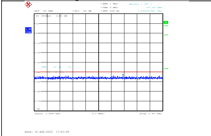
Band13-5MHz-QPSK-23255-1RB#0-Range5:1559~1610MHz
