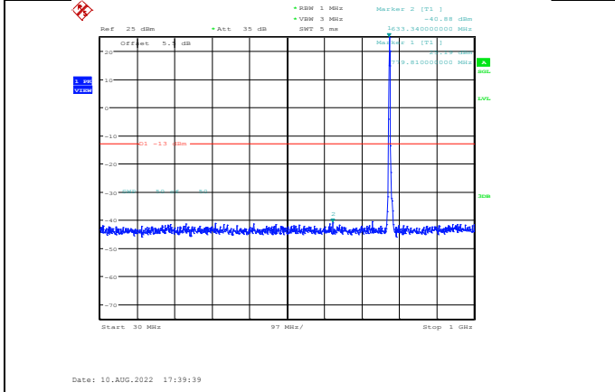
Band13-5MHz-16QAM-23230-1RB#0-Range1:30~1000MHz
