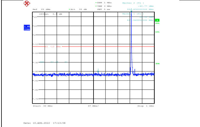
Band26-5MHz-64QAM-26740-1RB#0-Range1:30~1000MHz
