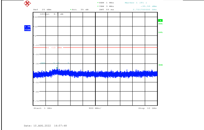
Band13-5MHz-64QAM-23255-1RB#0-Range2:1000~10000MHz
