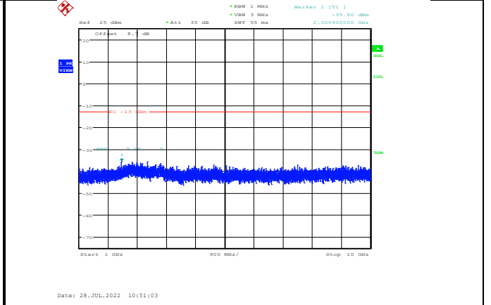
Band12-1.4MHz-16QAM-23173-1RB#0- Range2:1000~10000MHz
