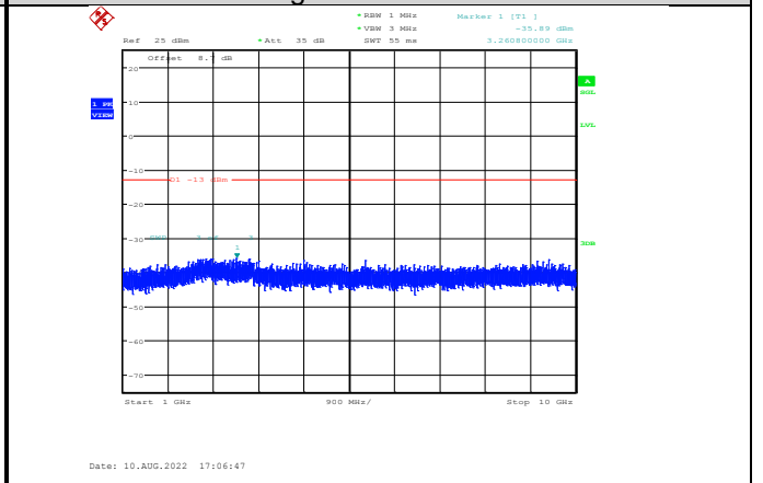
Band26-1.4MHz-64QAM-26783-1RB#0- Range2:1000~10000MHz
