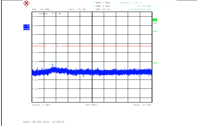
Band12-5MHz-16QAM-23035-1RB#0-Range2:1000~10000MHz
