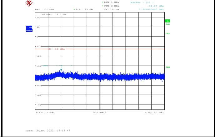
Band26-10MHz-64QAM-26740-1RB#0-Range2:1000~10000MHz
