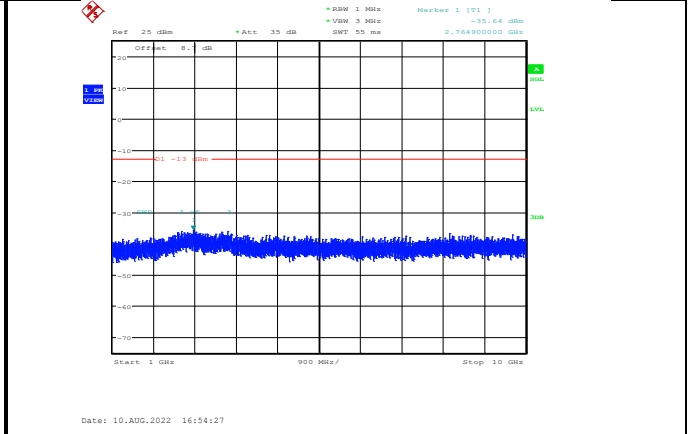
Band12-10MHz-64QAM-23130-1RB#0- Range2:1000~10000MHz
