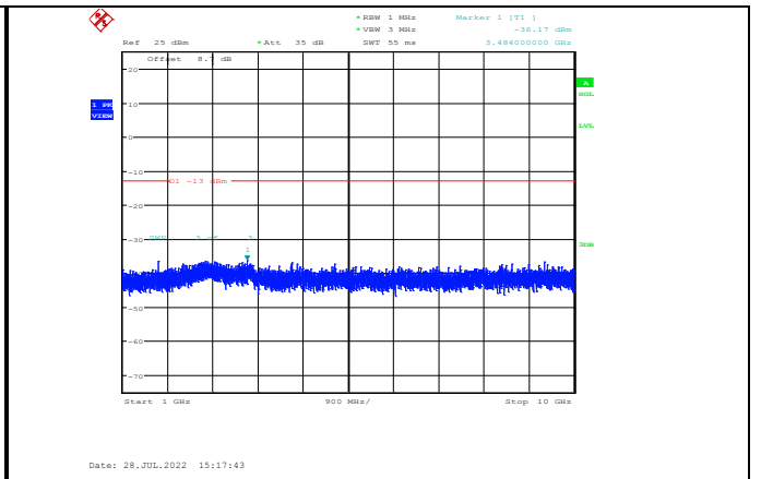
Band26-10MHz-16QAM-26740-1RB#0-Range2:1000~10000MHz
