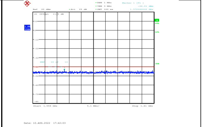
Band13-5MHz-16QAM-23255-1RB#0-Range5:1559~1610MHz
