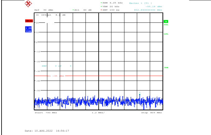
Band13-5MHz-64QAM-23205-1RB#0-Range4:793~805MHz
