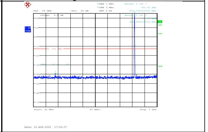
Band26-1.4MHz-64QAM-26783-1RB#0- Range1:30~1000MHz
