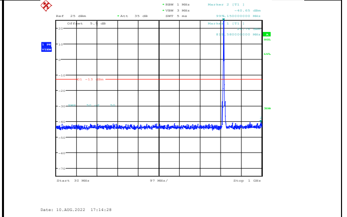
Band26-5MHz-64QAM-26765-1RB#0-Range1:30~1000MHz
