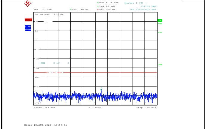
Band13-5MHz-64QAM-23255-1RB#0-Range3:763~775MHz
