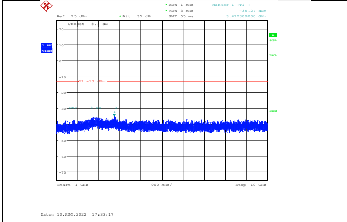
Band12-1.4MHz-16QAM-23017-1RB#0- Range2:1000~10000MHz
