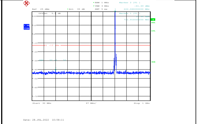
Band12-5MHz-16QAM-23155-1RB#0-Range1:30~1000MHz
