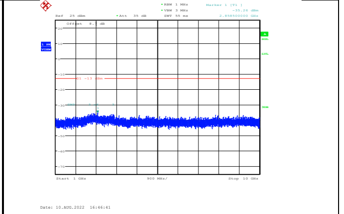
Band12-3MHz-64QAM-23165-1RB#0-Range2:1000~10000MHz
