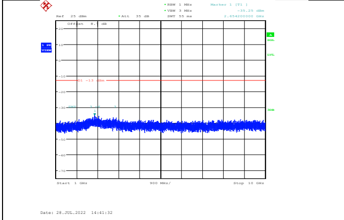
Band17-10MHz-16QAM-23780-1RB#0- Range2:1000~10000MHz
