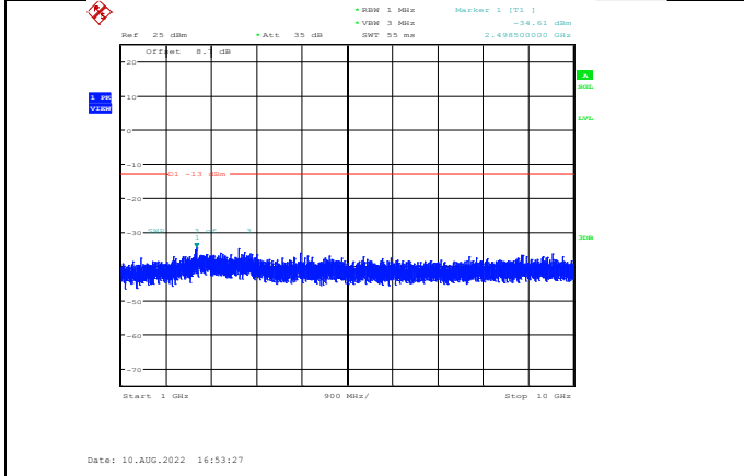
Band12-10MHz-64QAM-23060-1RB#0- Range2:1000~10000MHz
