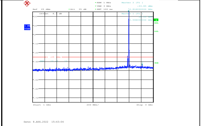
Band38-5MHz-QPSK-38000-1RB#0-Range2:1000~3000MHz
