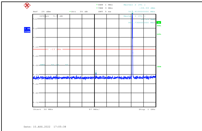
Band26-1.4MHz-64QAM-26697-1RB#0- Range1:30~1000MHz
