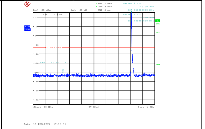
Band26-10MHz-64QAM-26740-1RB#0-Range1:30~1000MHz
