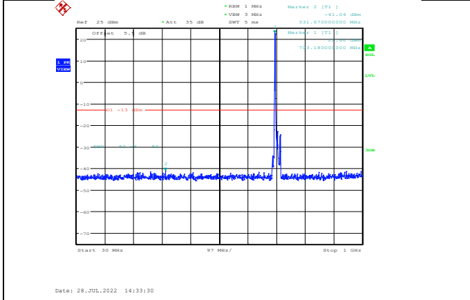
Band12-10MHz-16QAM-23095-1RB#0- Range1:30~1000MHz
