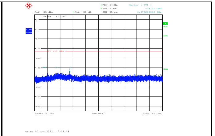
Band26-1.4MHz-64QAM-26740-1RB#0- Range2:1000~10000MHz
