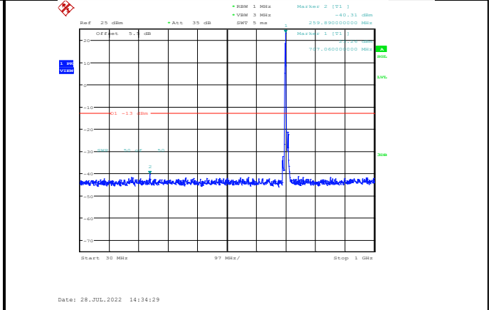
Band12-10MHz-16QAM-23130-1RB#0- Range1:30~1000MHz
