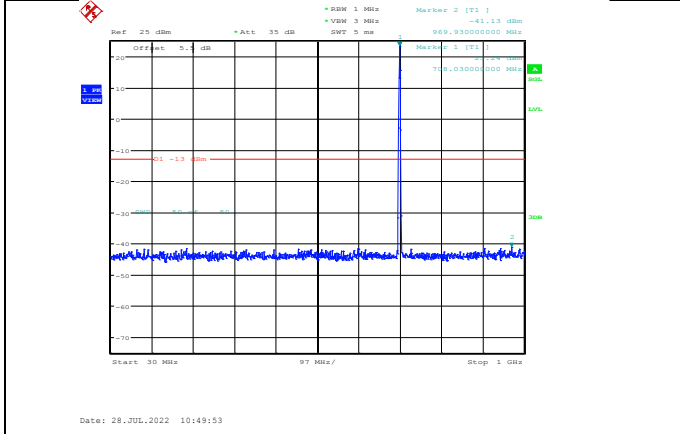
Band12-1.4MHz-16QAM-23095-1RB#0- Range1:30~1000MHz
