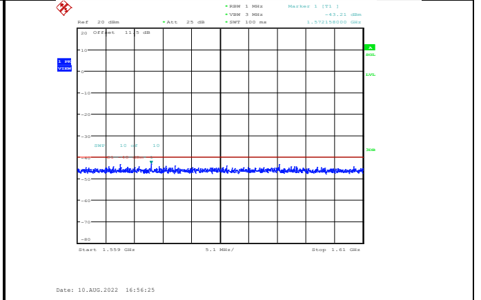
Band13-5MHz-64QAM-23205-1RB#0-Range5:1559~1610MHz
