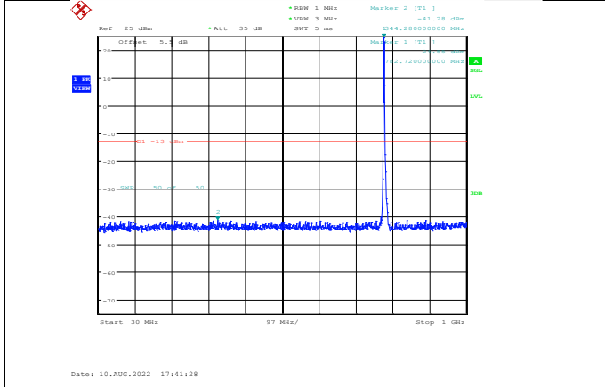
Band13-5MHz-16QAM-23255-1RB#0-Range1:30~1000MHz
