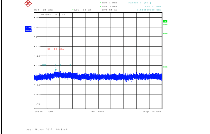
Band12-10MHz-16QAM-23060-1RB#0- Range2:1000~10000MHz
