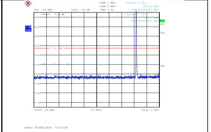
Band26-3MHz-64QAM-26775-1RB#0-Range1:30~1000MHz
