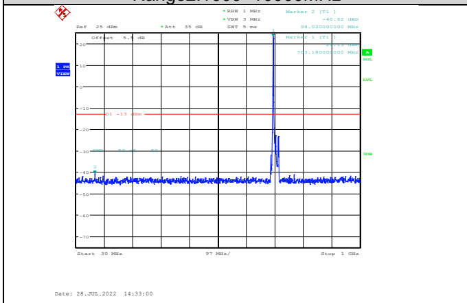
Band12-10MHz-QPSK-23095-1RB#0- Range1:30~1000MHz
