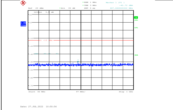
Band4-20MHz-16QAM-20175-1RB#0-Range1:30~1000MHz
