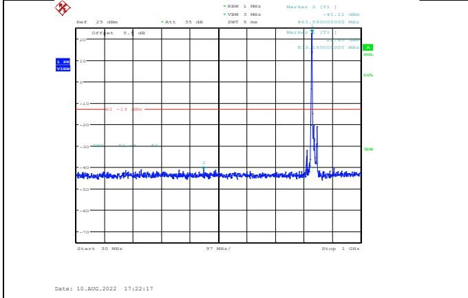
Band5-10MHz-64QAM-20525-1RB#0-Range1:30~1000MHz
