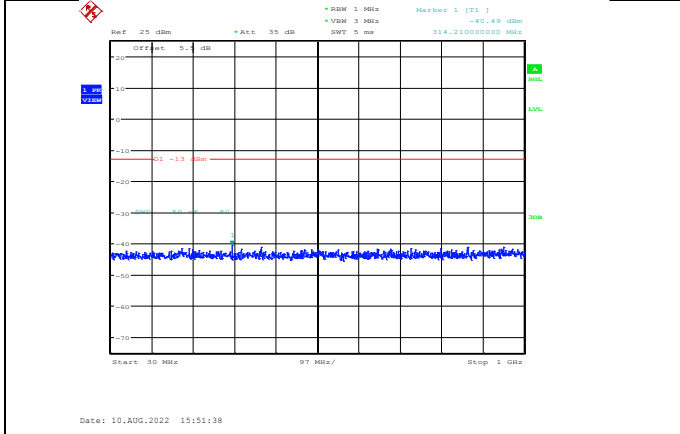
Band4-10MHz-64QAM-20175-1RB#0-Range1:30~1000MHz
