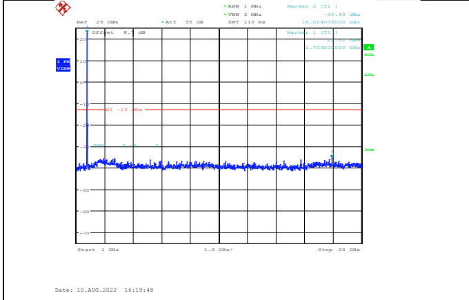
Band4-20MHz-64QAM-20050-1RB#0-Range2:1000~20000MHz
