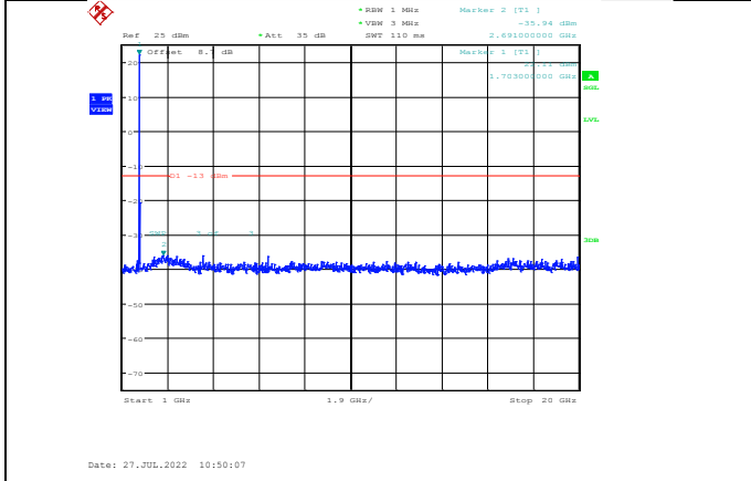
Band4-20MHz-16QAM-20050-1RB#0-Range2:1000~20000MHz
