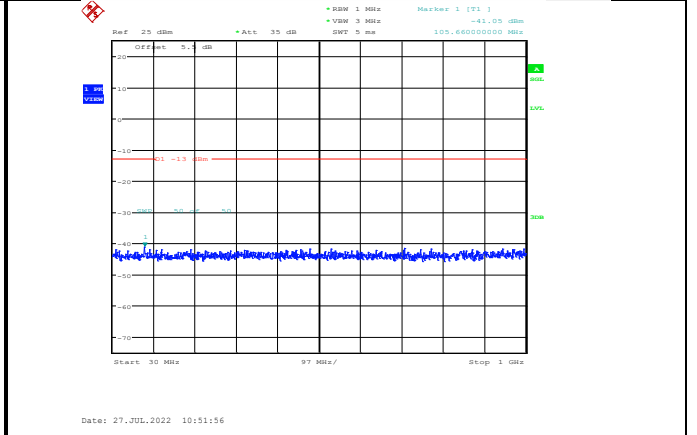
Band4-20MHz-16QAM-20300-1RB#0-Range1:30~1000MHz
