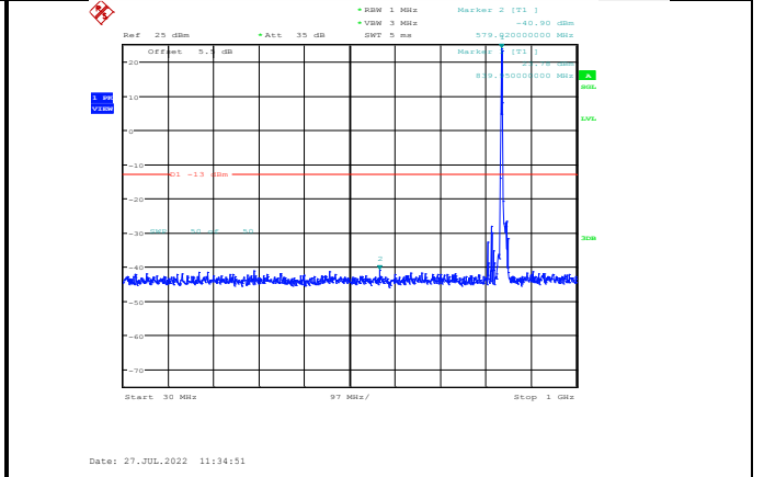
Band5-10MHz-QPSK-20600-1RB#0- Range1:30~1000MHz
