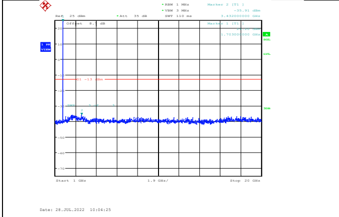
Band4-5MHz-16QAM-19975-1RB#0-Range2:1000~20000MHz
