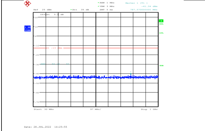
Band4-10MHz-16QAM-20175-1RB#0-Range1:30~1000MHz
