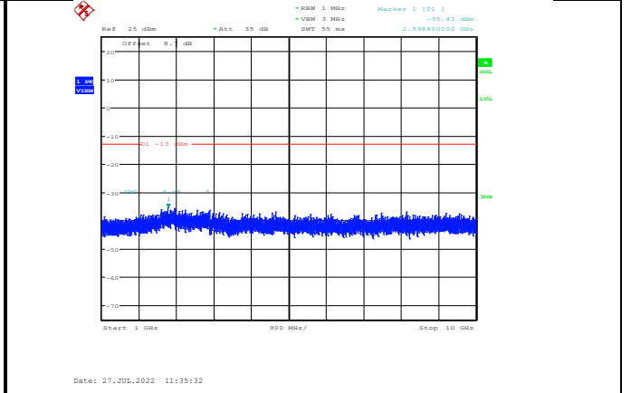
Band5-10MHz-16QAM-20600-1RB#0-Range2:1000~10000MHz
