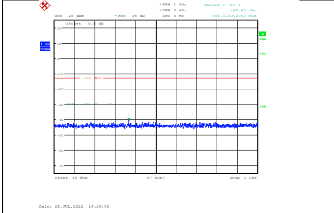
Band4-15MHz-QPSK-20175-1RB#0-Range1:30~1000MHz
