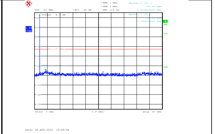
Band4-5MHz-64QAM-20375-1RB#0- Range2:1000~20000MHz
