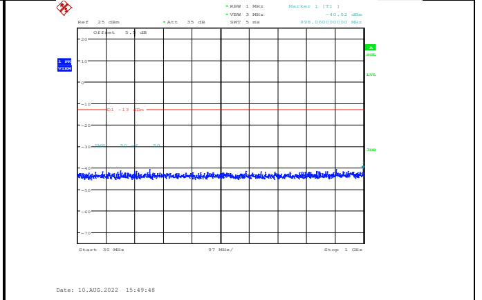
Band4-5MHz-64QAM-20375-1RB#0- Range1:30~1000MHz
