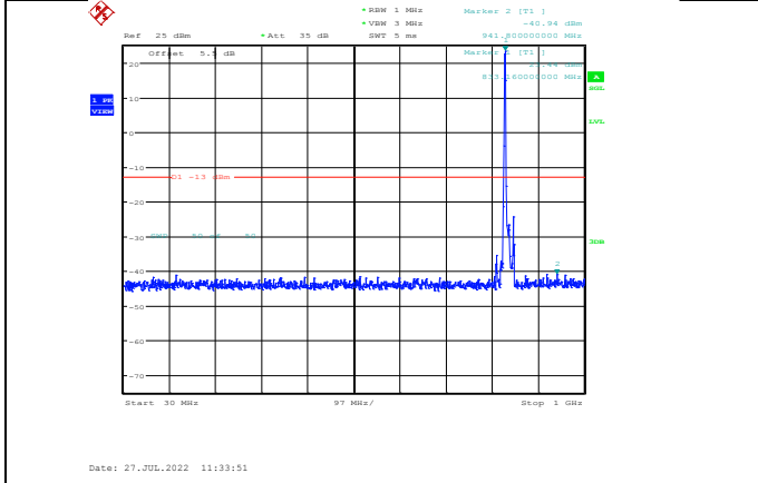
Band5-10MHz-QPSK-20525-1RB#0- Range1:30~1000MHz
