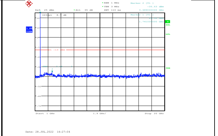
Band4-10MHz-16QAM-20350-1RB#0-Range2:1000~20000MHz
