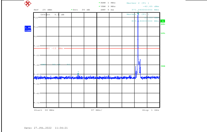
Band5-10MHz-16QAM-20525-1RB#0-Range1:30~1000MHz
