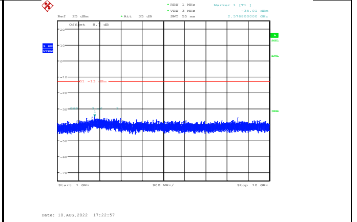
Band5-10MHz-64QAM-20600-1RB#0-Range2:1000~10000MHz
