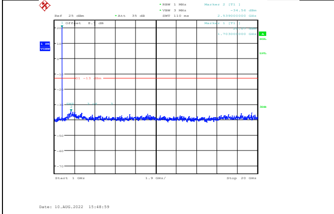
Band4-5MHz-64QAM-19975-1RB#0- Range2:1000~20000MHz
