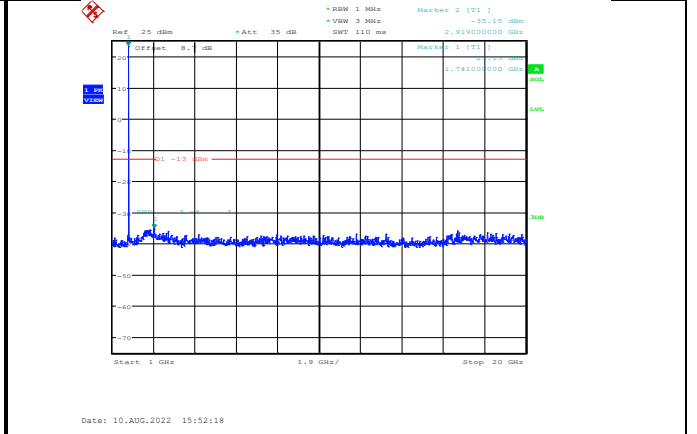
Band4-10MHz-64QAM-20350-1RB#0-Range2:1000~20000MHz
