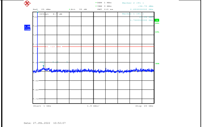
Band4-20MHz-16QAM-20300-1RB#0-Range2:1000~20000MHz
