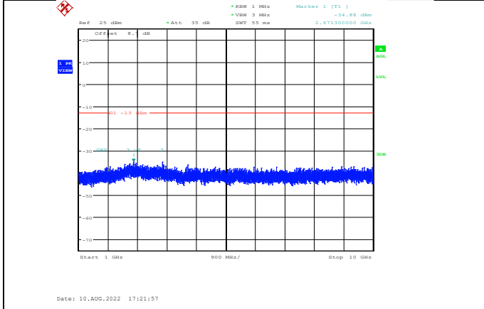
Band5-10MHz-64QAM-20450-1RB#0-Range2:1000~10000MHz
