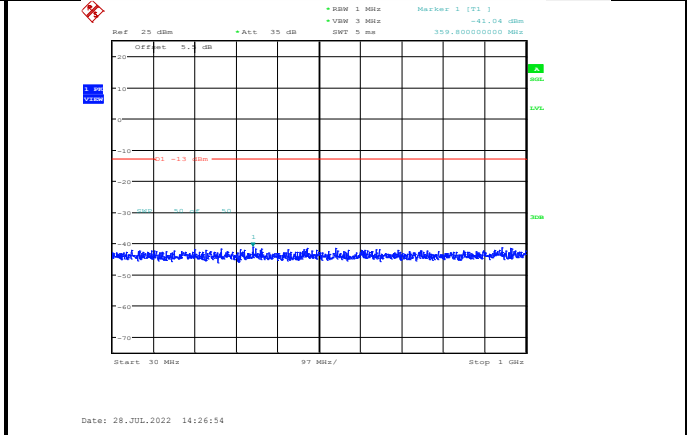
Band4-10MHz-16QAM-20350-1RB#0-Range1:30~1000MHz
