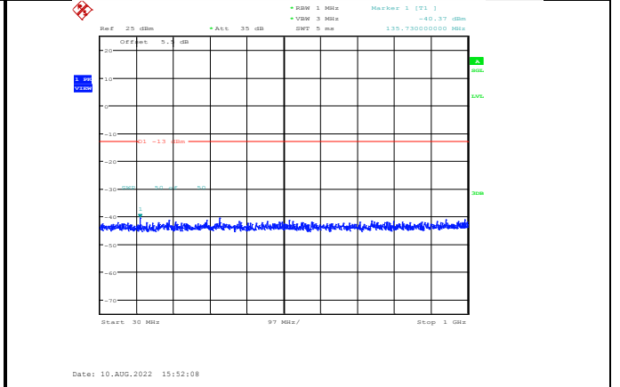
Band4-10MHz-64QAM-20350-1RB#0-Range1:30~1000MHz
