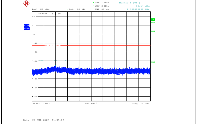
Band5-10MHz-QPSK-20600-1RB#0- Range2:1000~10000MHz
