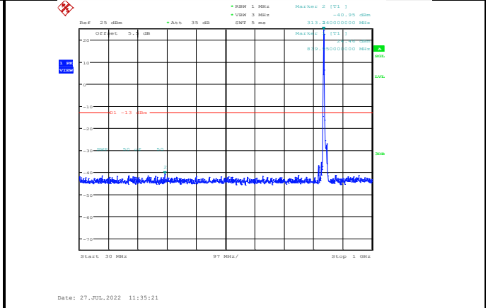
Band5-10MHz-16QAM-20600-1RB#0-Range1:30~1000MHz
