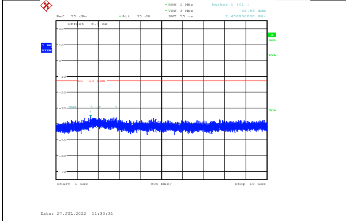
Band5-10MHz-16QAM-20450-1RB#0-Range2:1000~10000MHz
