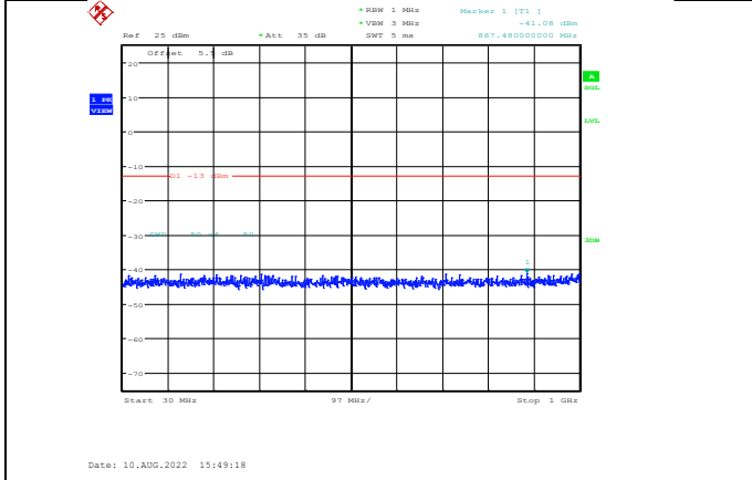
Band4-5MHz-64QAM-20175-1RB#0- Range1:30~1000MHz
