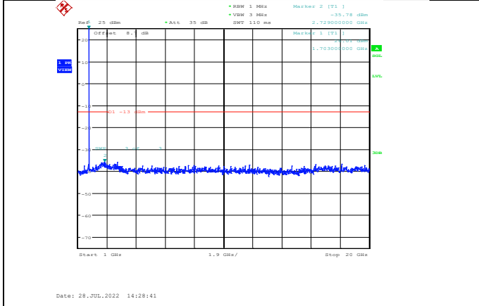
Band4-15MHz-16QAM-20025-1RB#0-Range2:1000~20000MHz
