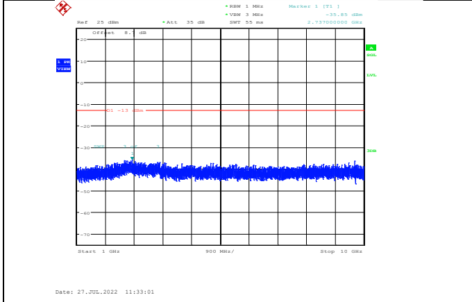
Band5-10MHz-QPSK-20450-1RB#0- Range2:1000~10000MHz
