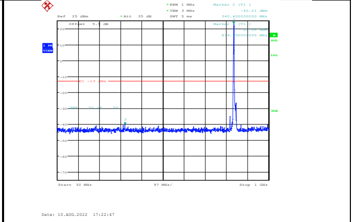
Band5-10MHz-64QAM-20600-1RB#0-Range1:30~1000MHz
