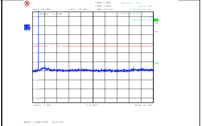
Band2-5MHz-64QAM-19175-1RB#0-Range2:1000~20000MHz
