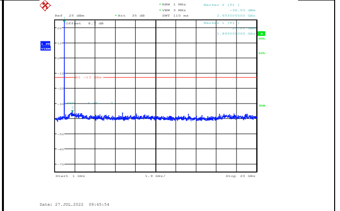
Band2-10MHz-16QAM-19150-1RB#0-Range2:1000~20000MHz
