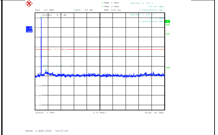
Band2-20MHz-64QAM-19100-1RB#0-Range2:1000~20000MHz
