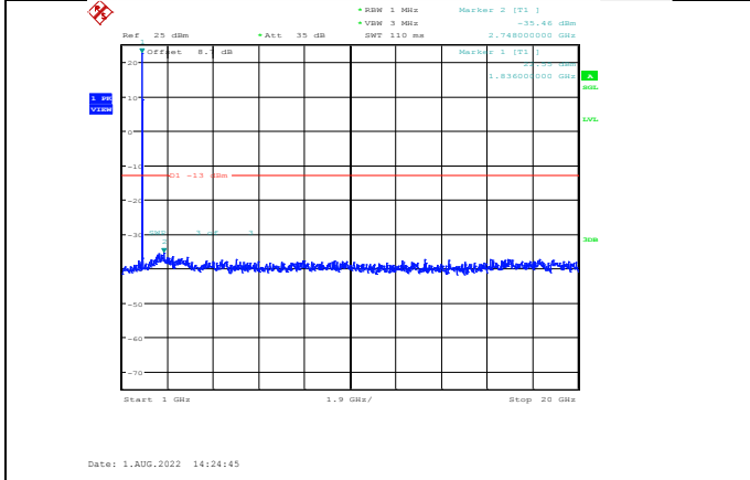
Band2-15MHz-64QAM-18675-1RB#0-Range2:1000~20000MHz
