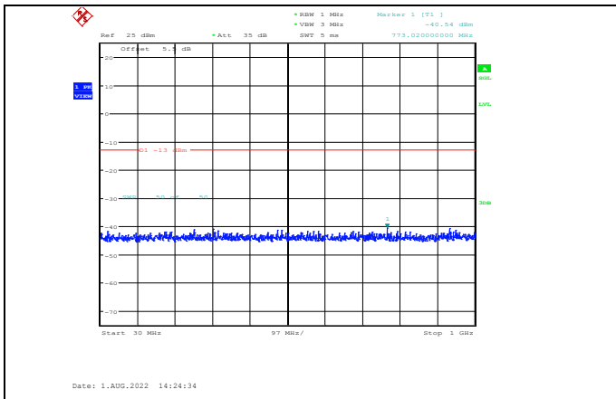
Band2-15MHz-64QAM-18675-1RB#0-Range1:30~1000MHz
