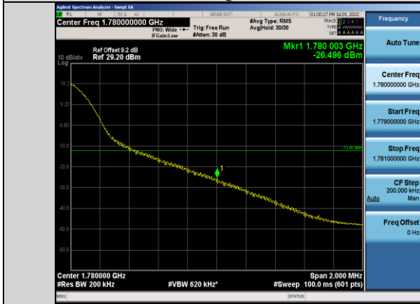
Band66-20MHz-16QAM-132572-1RB#99
