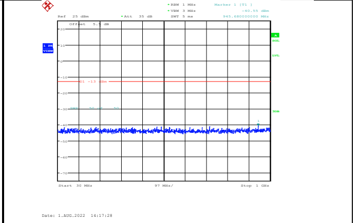
Band2-1.4MHz-64QAM-19193-1RB#0-Range1:30~1000MHz
