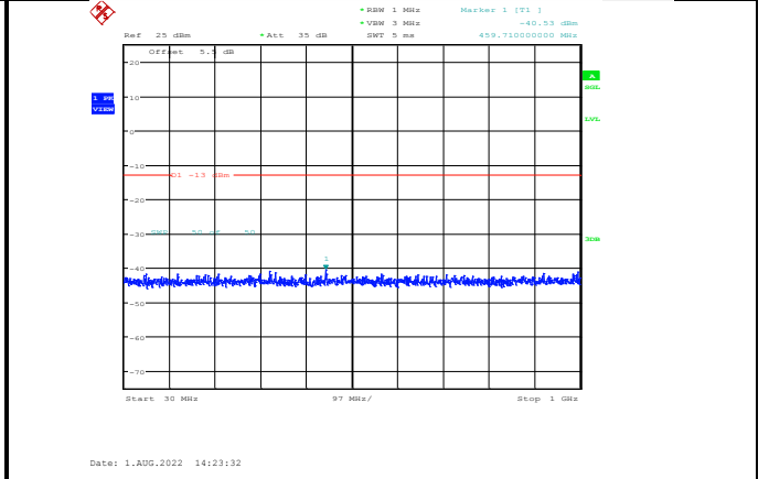
Band2-10MHz-64QAM-19150-1RB#0-Range1:30~1000MHz
