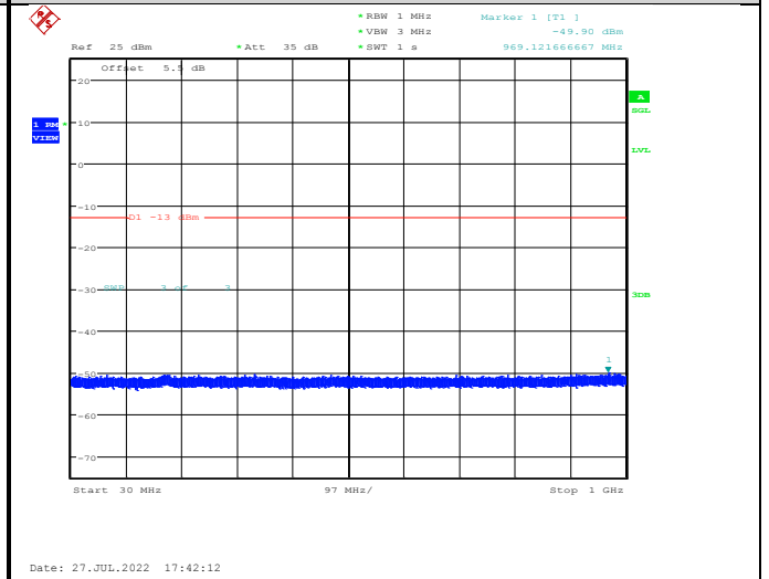
Band II-9538-30~1000MHz
