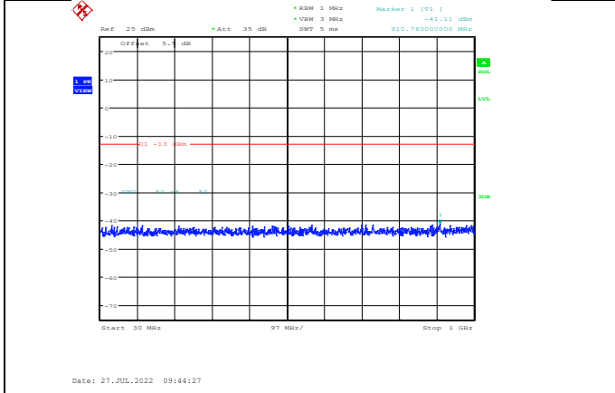
Band2-10MHz-16QAM-18900-1RB#0-Range1:30~1000MHz
