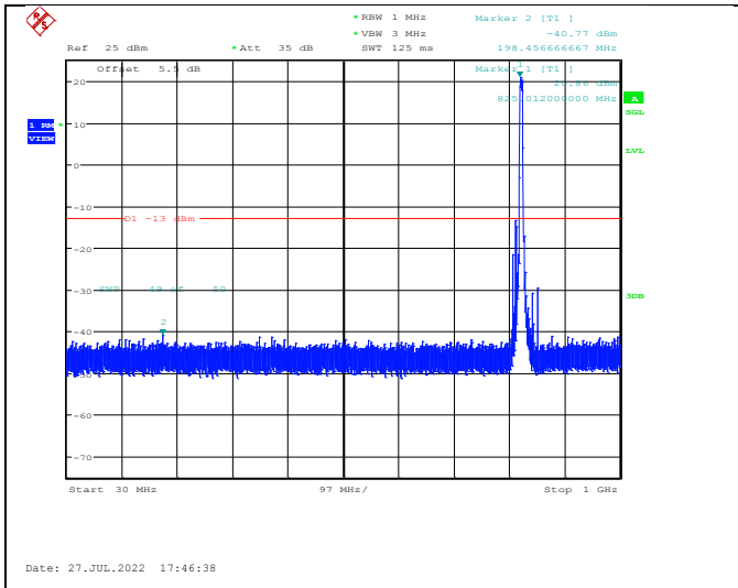
Band V-4132-30~1000MHz
