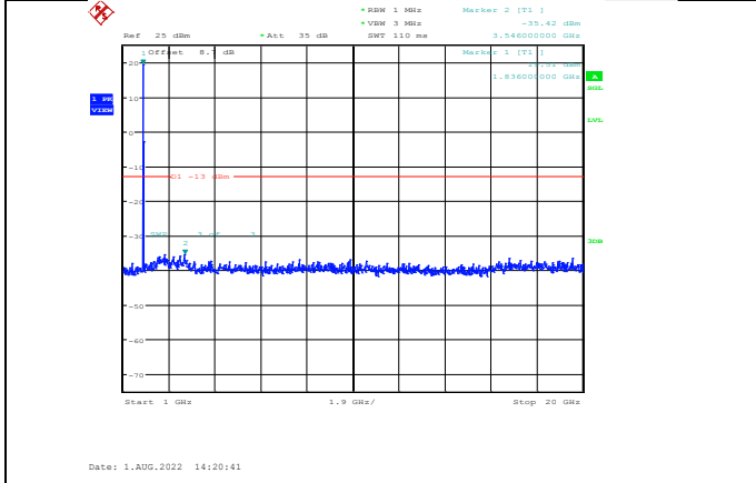
Band2-5MHz-64QAM-18625-1RB#0-Range2:1000~20000MHz
