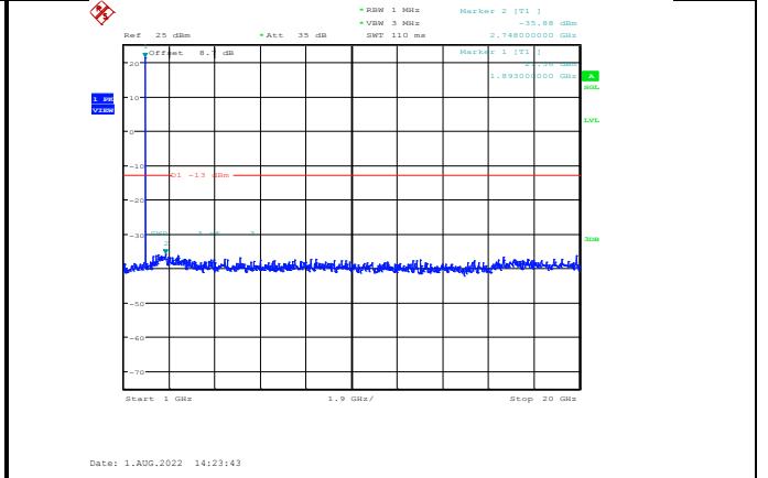
Band2-10MHz-64QAM-19150-1RB#0-Range2:1000~20000MHz
