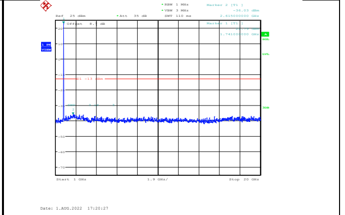
Band4-1.4MHz-64QAM-20393-1RB#0-Range2:1000~20000MHz
