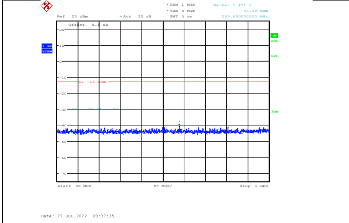
Band2-3MHz-16QAM-18900-1RB#0-Range1:30~1000MHz
