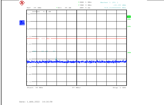
Band2-1.4MHz-64QAM-18900-1RB#0-Range1:30~1000MHz
