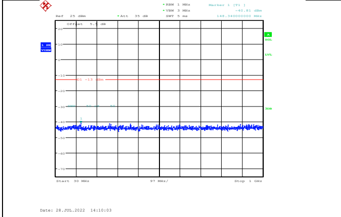
Band4-1.4MHz-QPSK-20175-1RB#0- Range1:30~1000MHz
