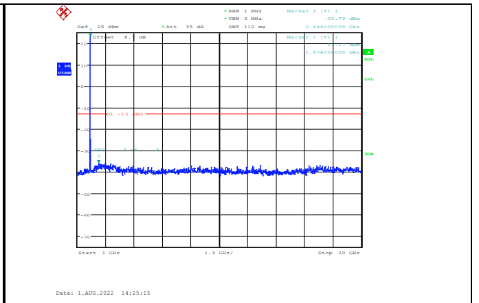
Band2-15MHz-64QAM-18900-1RB#0-Range2:1000~20000MHz
