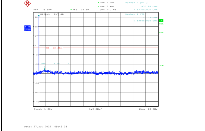
Band2-10MHz-16QAM-18650-1RB#0-Range2:1000~20000MHz
