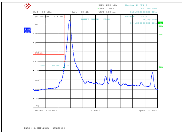
Band26-15MHz-QPSK-26765-1RB#0
