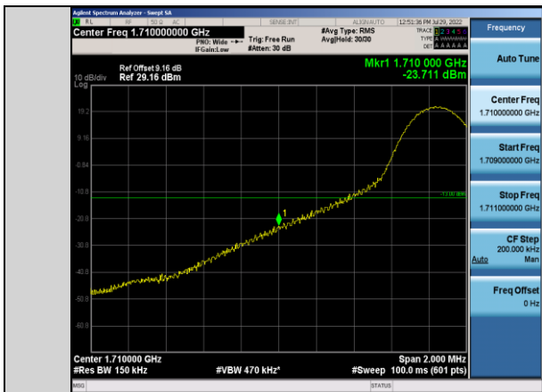
Band66-15MHz-16QAM-132047-1RB#0
