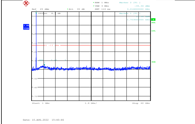
Band4-1.4MHz-64QAM-19957-1RB#0-Range2:1000~20000MHz
