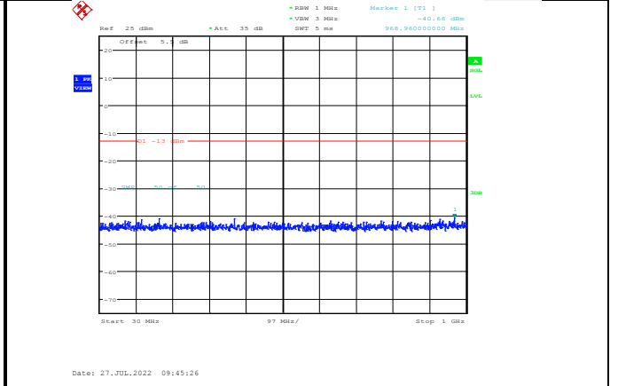
Band2-10MHz-16QAM-19150-1RB#0-Range1:30~1000MHz
