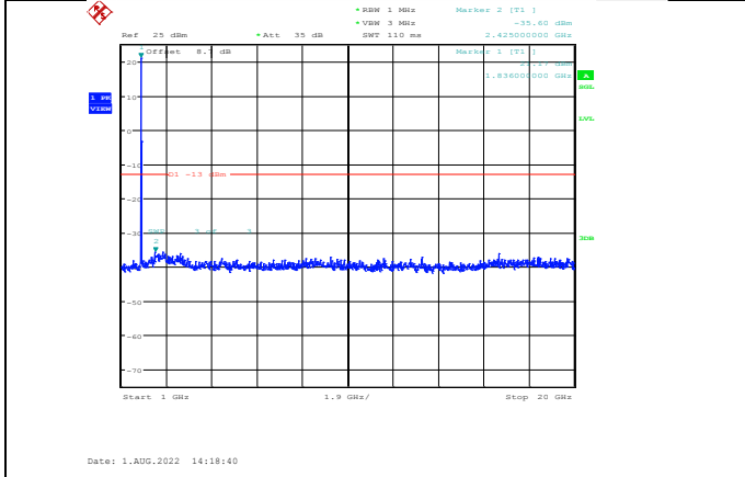
Band2-3MHz-64QAM-18615-1RB#0-Range2:1000~20000MHz
