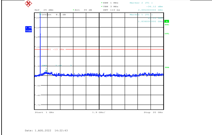
Band2-10MHz-64QAM-18650-1RB#0-Range2:1000~20000MHz
