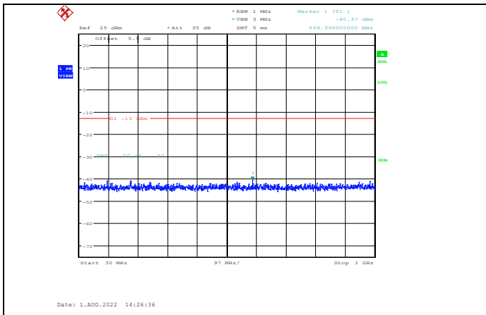
Band2-20MHz-64QAM-18700-1RB#0-Range1:30~1000MHz
