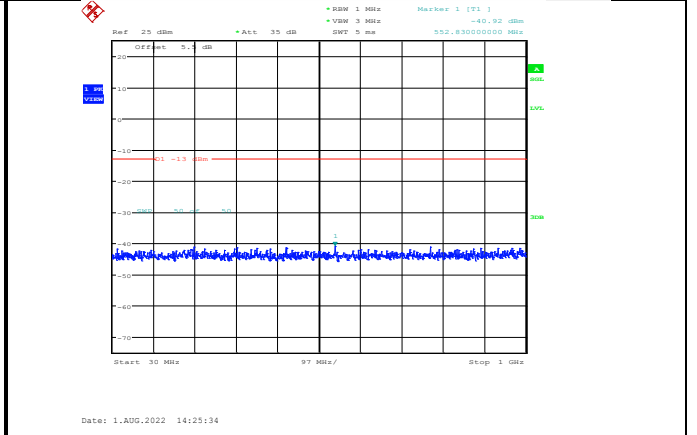
Band2-15MHz-64QAM-19125-1RB#0-Range1:30~1000MHz
