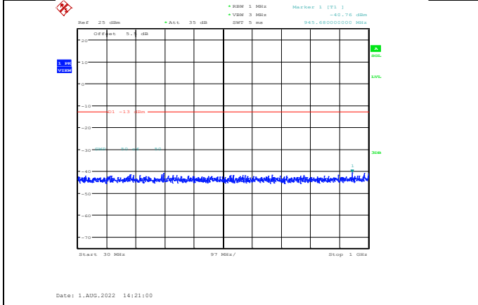
Band2-5MHz-64QAM-18900-1RB#0-Range1:30~1000MHz
