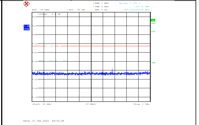
Band2-20MHz-16QAM-19100-1RB#0-Range1:30~1000MHz
