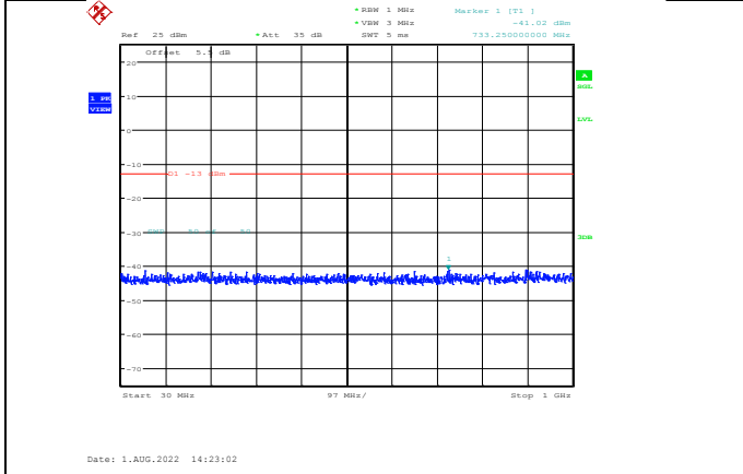
Band2-10MHz-64QAM-18900-1RB#0-Range1:30~1000MHz
