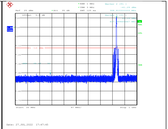
Band V-4182-30~1000MHz
