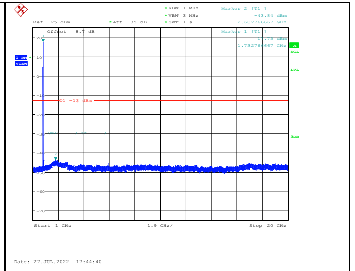
Band IV-1413-1000~20000MHz
