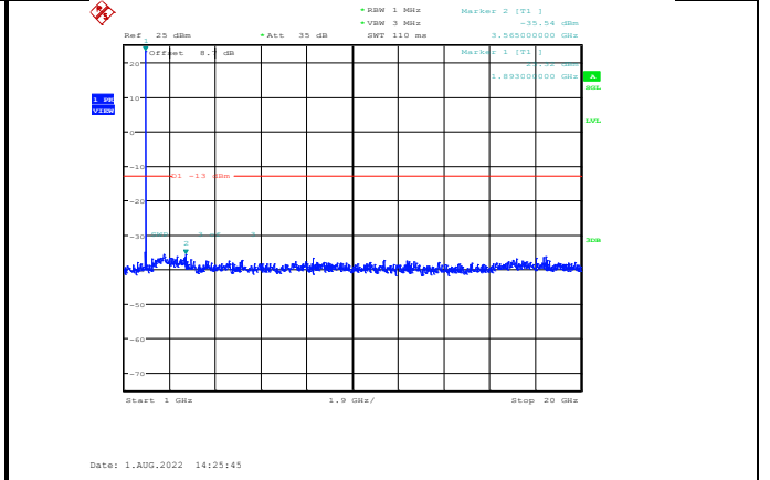
Band2-15MHz-64QAM-19125-1RB#0-Range2:1000~20000MHz
