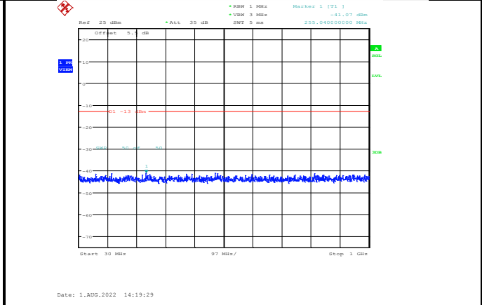
Band2-3MHz-64QAM-19185-1RB#0-Range1:30~1000MHz
