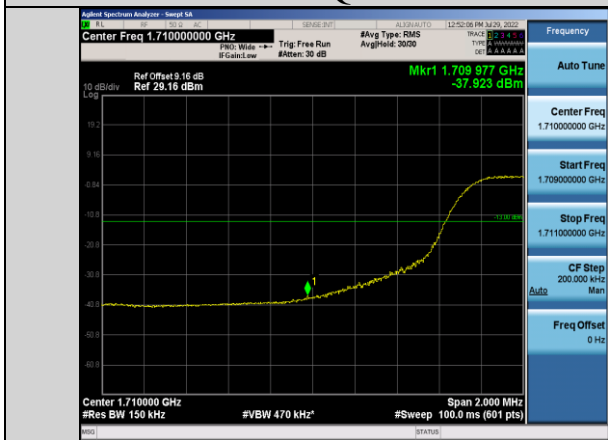
Band66-15MHz-16QAM-132047-75RB#0
