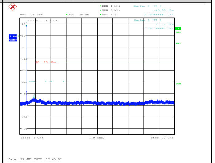
Band IV-1513-1000~20000MHz
