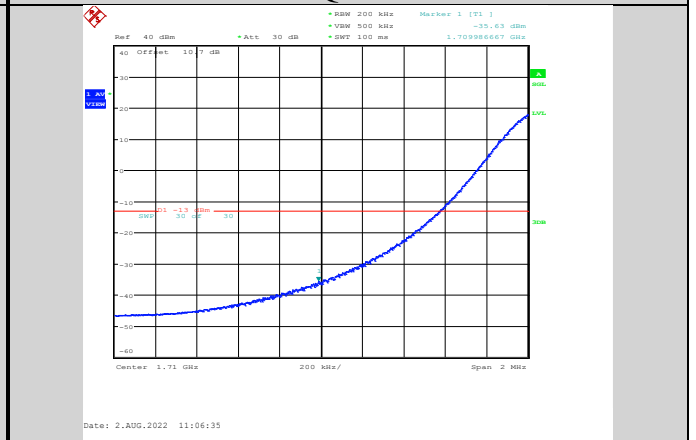
Band66-20MHz-64QAM-132072-1RB#0
