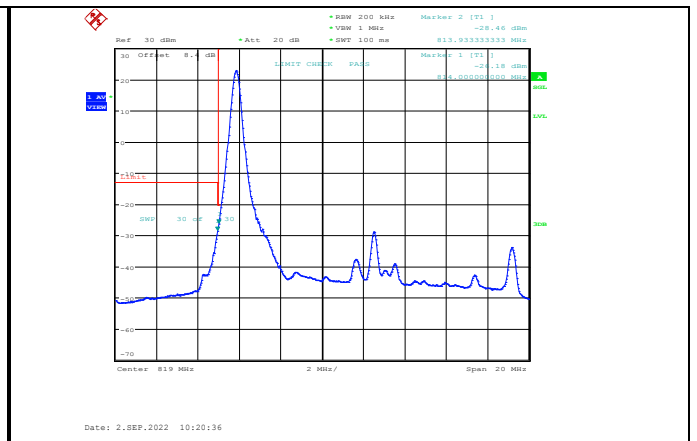
Band26-15MHz-16QAM-26765-1RB#0
