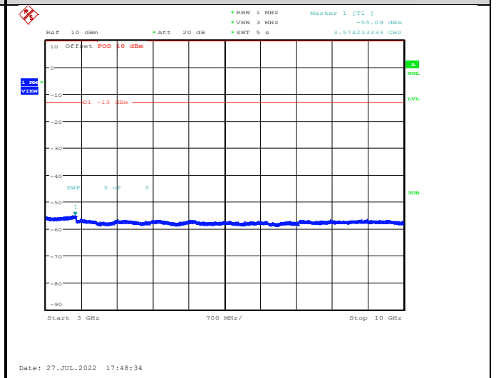
Band V-4182-3000~10000MHz
