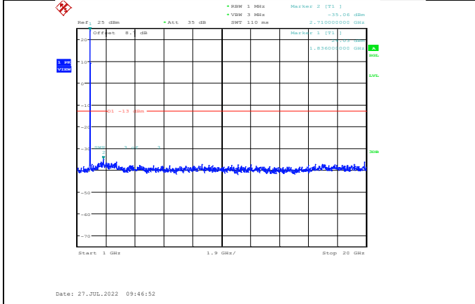
Band2-15MHz-QPSK-18675-1RB#0- Range2:1000~20000MHz
