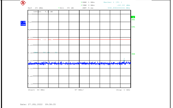
Band2-3MHz-16QAM-19185-1RB#0-Range1:30~1000MHz
