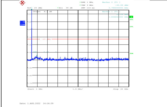
Band2-1.4MHz-64QAM-18607-1RB#0-Range2:1000~20000MHz
