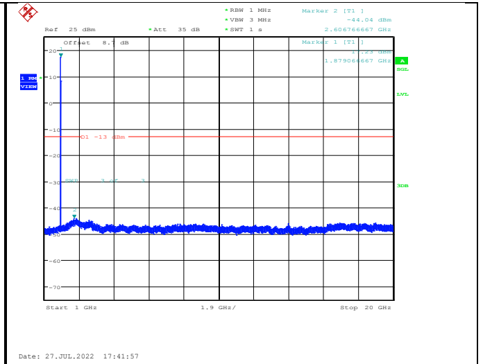
Band II-9400-1000~20000MHz
