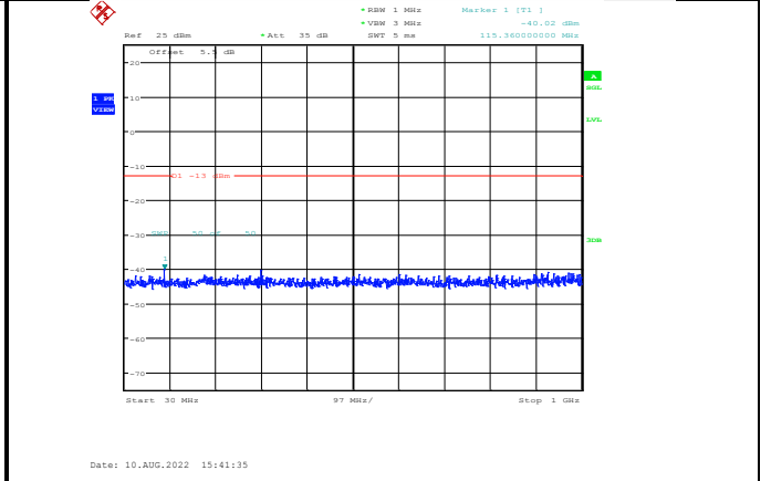
Band4-1.4MHz-64QAM-20393-1RB#0-Range1:30~1000MHz
