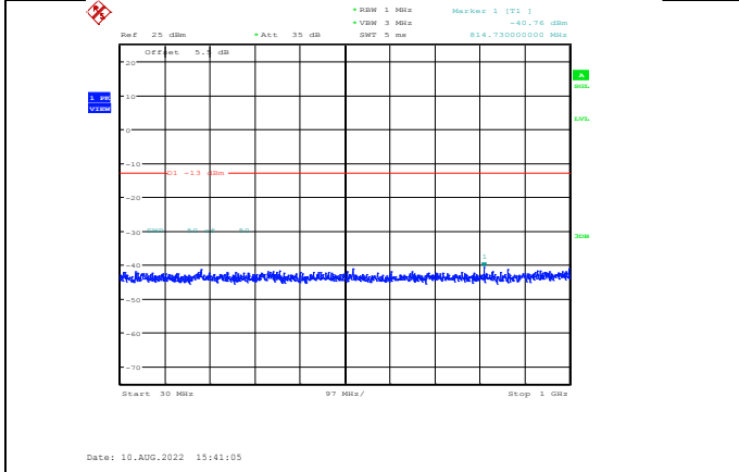
Band4-1.4MHz-64QAM-20175-1RB#0-Range1:30~1000MHz
