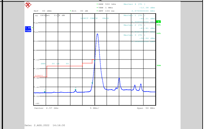
Band38-20MHz-64QAM-37850-1RB#0
