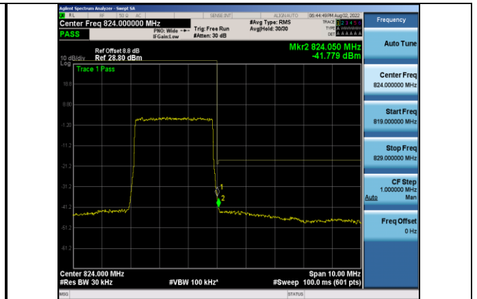
Band26-3MHz-16QAM-26775-15RB#0
