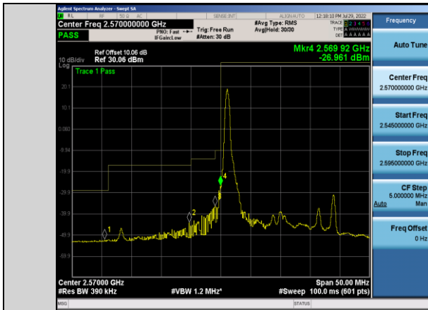
Band38-20MHz-16QAM-37850-1RB#0
