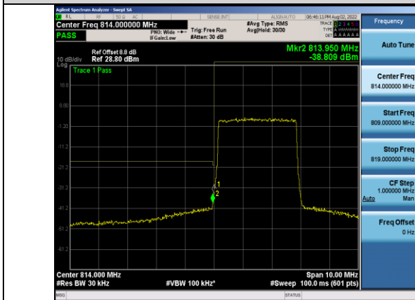
Band26-3MHz-16QAM-26705-15RB#0
