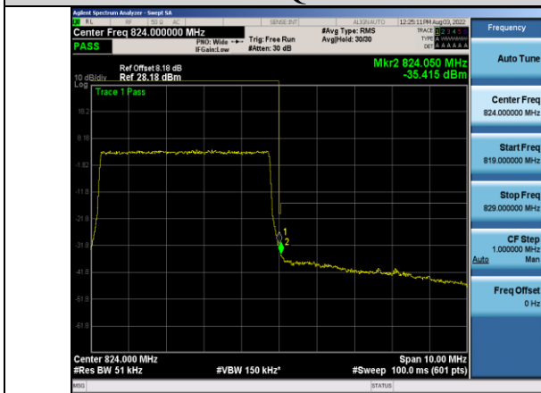
Band26-5MHz-64QAM-26765-25RB#0
