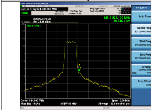
Band26-1.4MHz-64QAM-26783-6RB#0
