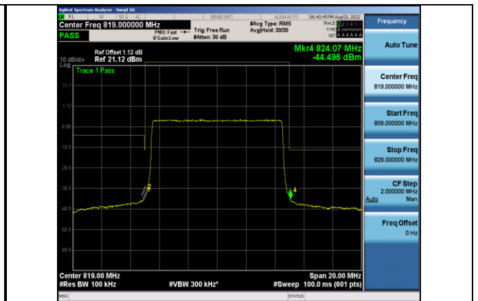
Band26-10MHz-16QAM-26740_Right-50RB#0
