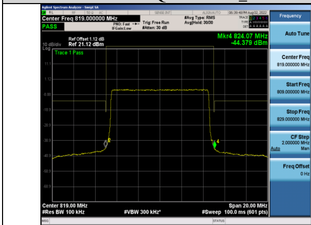
Band26-10MHz-16QAM-26740_Left-50RB#0
