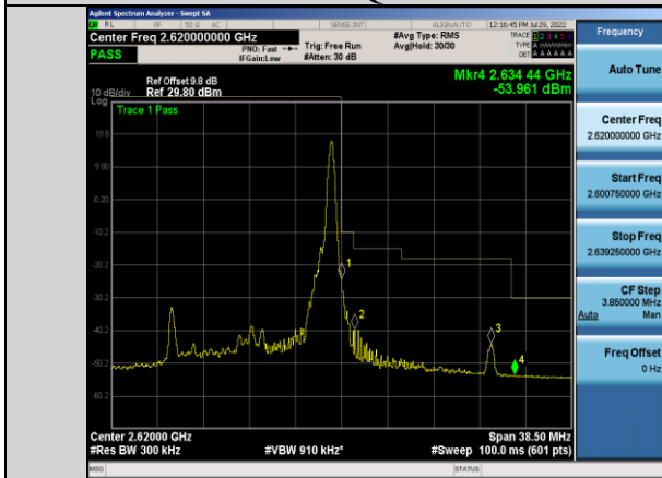
Band38-15MHz-16QAM-38175-1RB#74
