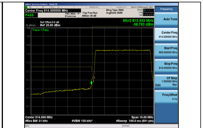
Band26-5MHz-QPSK-26715-25RB#0
