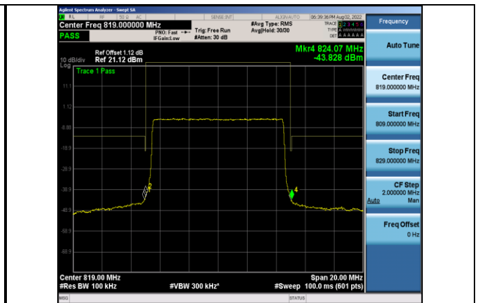
Band26-10MHz-QPSK-26740_Left-50RB#0
