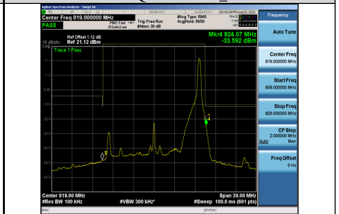
Band26-10MHz-QPSK-26740_Right-1RB#49
