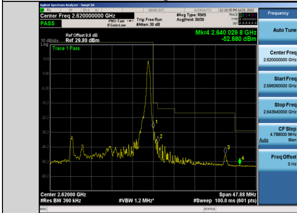
Band38-20MHz-16QAM-38150-1RB#99
