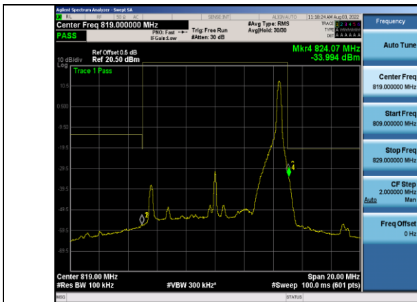
Band26-10MHz-64QAM-26740_Right-1RB#49
