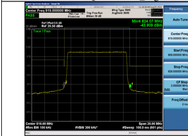
Band26-10MHz-64QAM-26740_Right-50RB#0
