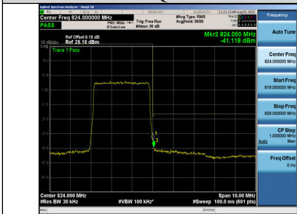
Band26-3MHz-64QAM-26775-15RB#0
