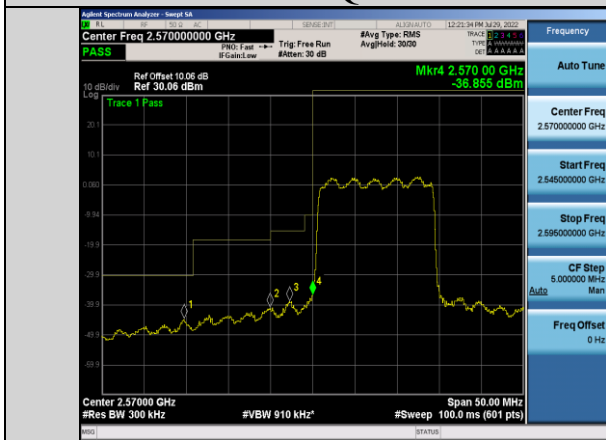
Band38-15MHz-16QAM-37825-75RB#0
