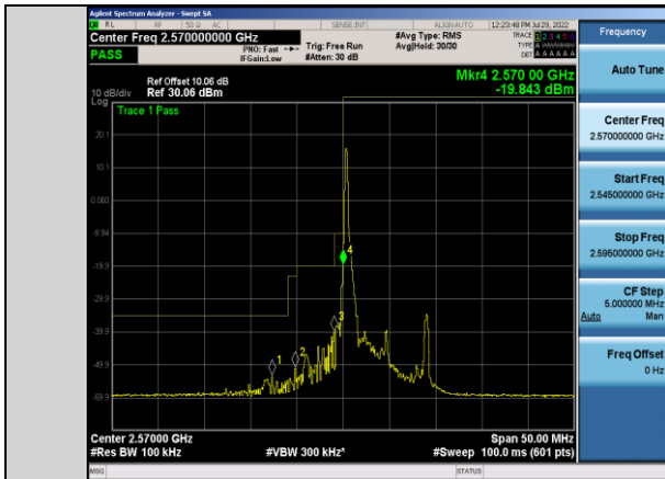
Band38-5MHz-16QAM-37775-1RB#0
