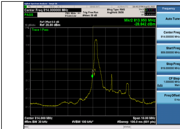
Band26-3MHz-16QAM-26705-1RB#0
