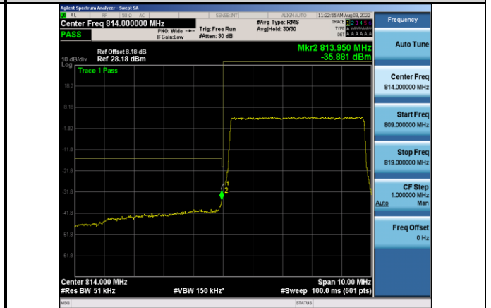
Band26-5MHz-64QAM-26715-25RB#0
