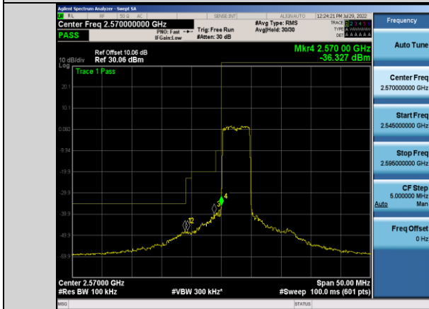
Band38-5MHz-16QAM-37775-25RB#0
