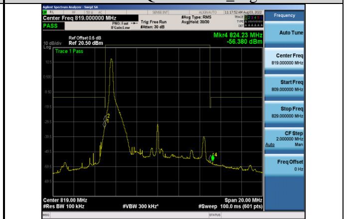
Band26-10MHz-64QAM-26740_Left-1RB#0
