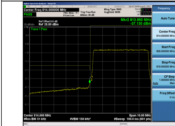
Band26-5MHz-16QAM-26715-25RB#0
