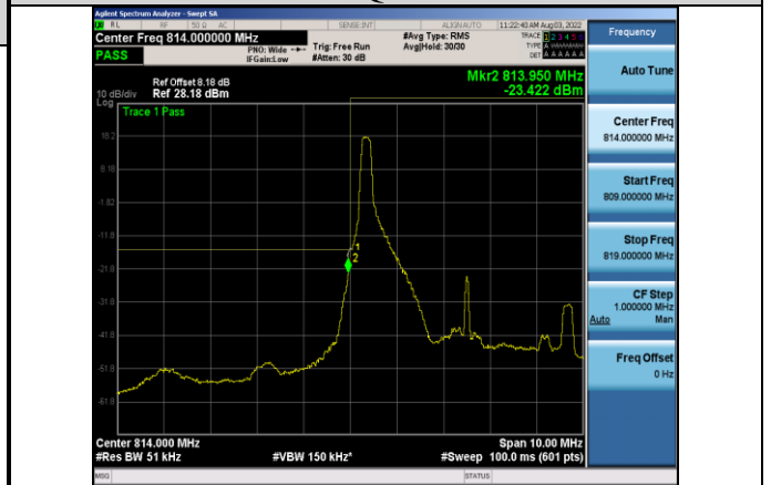
Band26-5MHz-64QAM-26715-1RB#0
