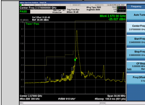
Band38-15MHz-QPSK-37825-1RB#0
