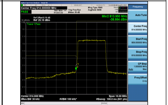
Band26-3MHz-64QAM-26705-15RB#0
