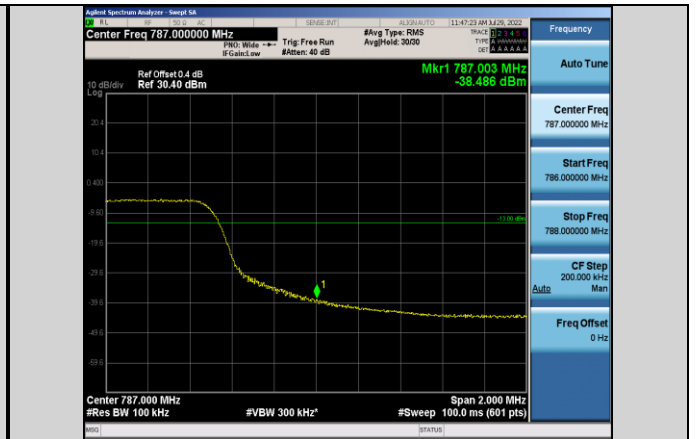
Band13-10MHz-16QAM-23230-50RB#0
