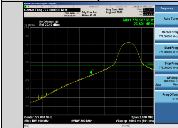
Band13-10MHz-QPSK-23230-1RB#0
