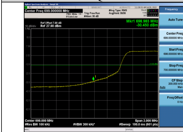
Band12-10MHz-QPSK-23060-50RB#0
