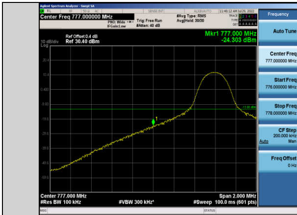
Band13-10MHz-16QAM-23230-1RB#0
