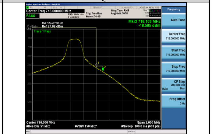
Band12-5MHz-16QAM-23155-1RB#24
