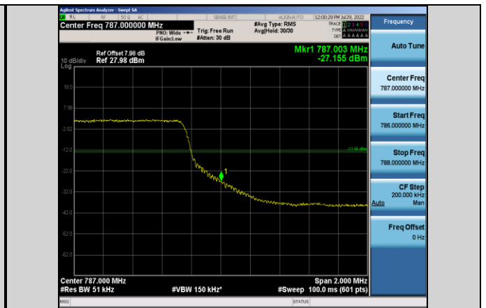
Band13-5MHz-16QAM-23255-25RB#0
