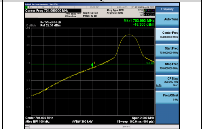
Band17-10MHz-64QAM-23780-1RB#0
