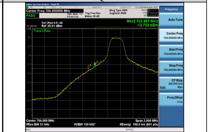
Band17-5MHz-64QAM-23755-1RB#0
