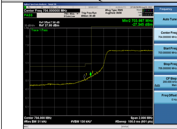
Band17-5MHz-16QAM-23755-25RB#0
