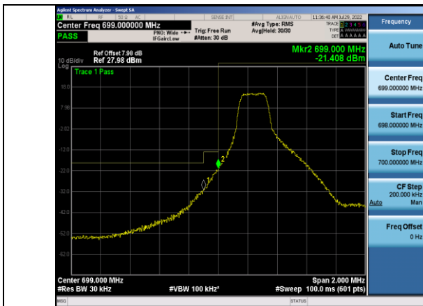
Band12-3MHz-16QAM-23025-1RB#0
