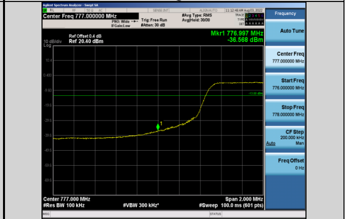
Band13-10MHz-64QAM-23230-50RB#0
