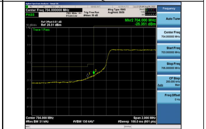
Band17-5MHz-64QAM-23755-25RB#0
