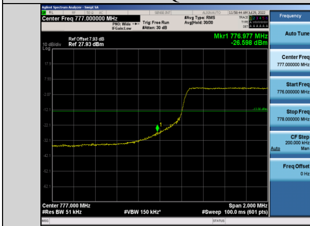
Band13-5MHz-16QAM-23205-25RB#0
