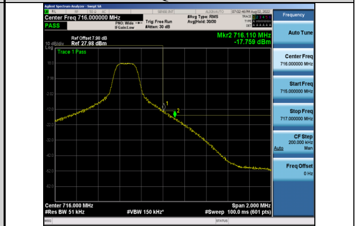
Band17-5MHz-QPSK-23825-1RB#24
