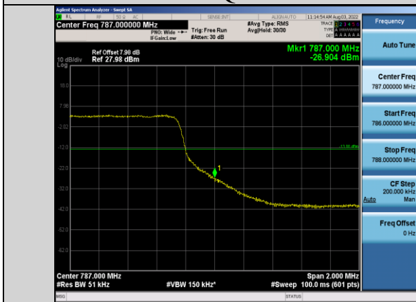
Band13-5MHz-64QAM-23255-25RB#0
