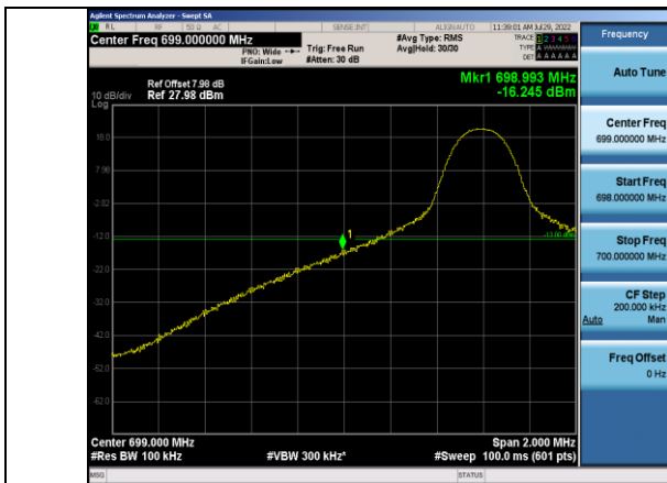
Band12-10MHz-QPSK-23060-1RB#0
