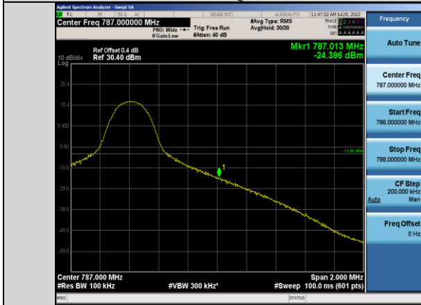
Band13-10MHz-16QAM-23230-1RB#49
