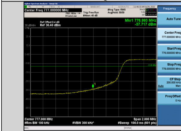
Band13-10MHz-16QAM-23230-50RB#0
