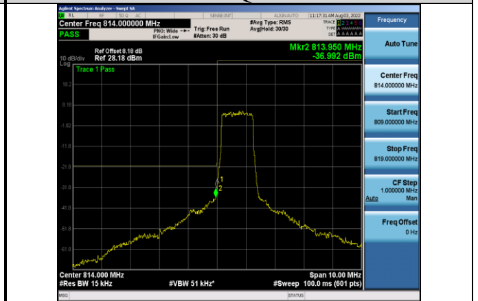
Band26-1.4MHz-64QAM-26697-6RB#0
