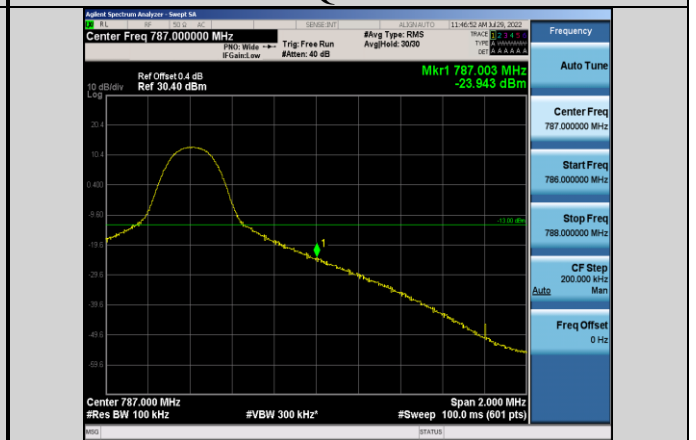
Band13-10MHz-QPSK-23230-1RB#49
