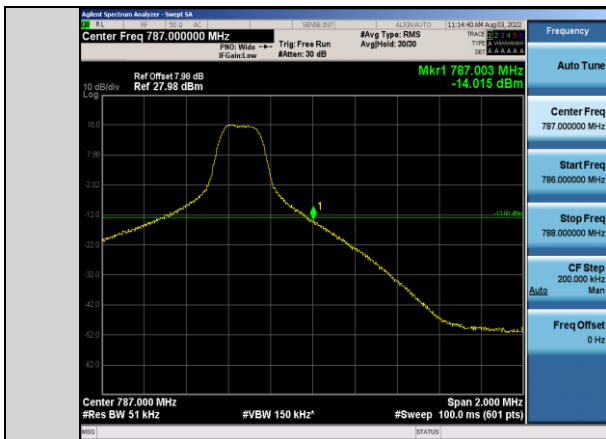
Band13-5MHz-64QAM-23255-1RB#24
