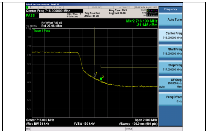
Band17-5MHz-16QAM-23825-25RB#0
