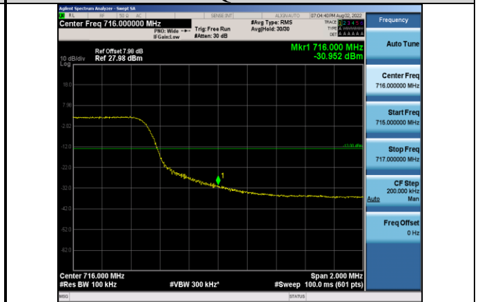
Band17-10MHz-QPSK-23800-50RB#0
