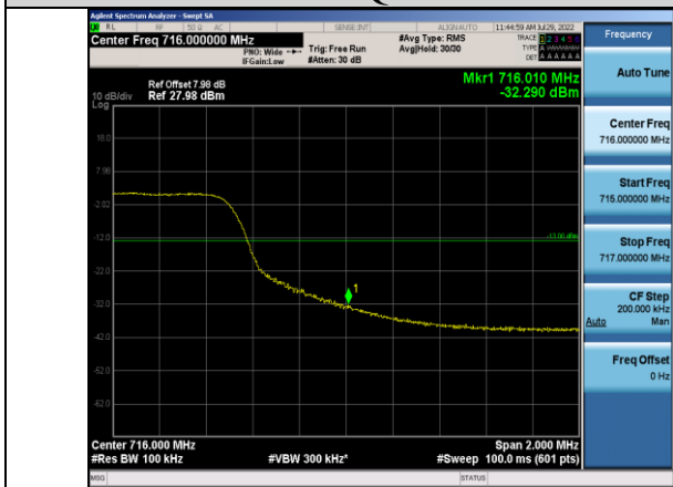
Band12-10MHz-16QAM-23130-50RB#0
