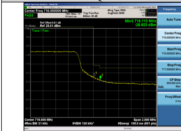
Band17-5MHz-64QAM-23825-25RB#0
