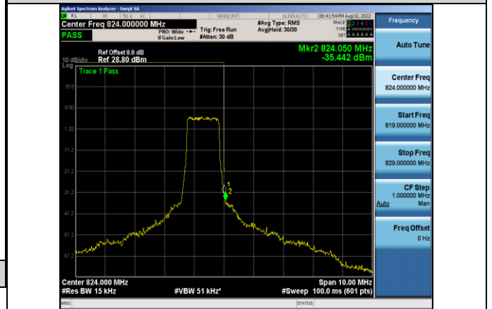
Band26-1.4MHz-QPSK-26783-1RB#5
