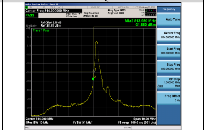
Band26-1.4MHz-64QAM-26697-1RB#0
