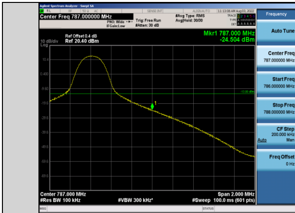
Band13-10MHz-64QAM-23230-1RB#49
