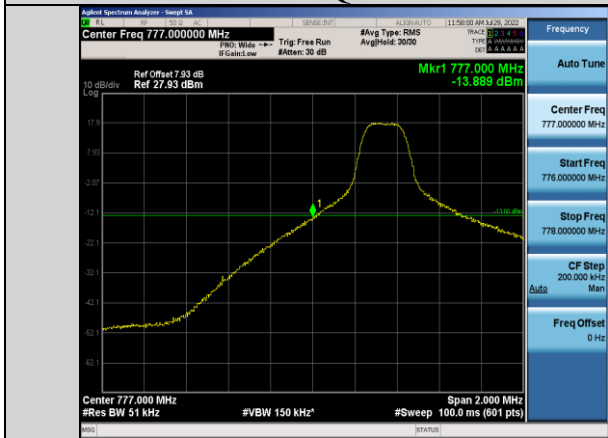
Band13-5MHz-QPSK-23205-1RB#0
