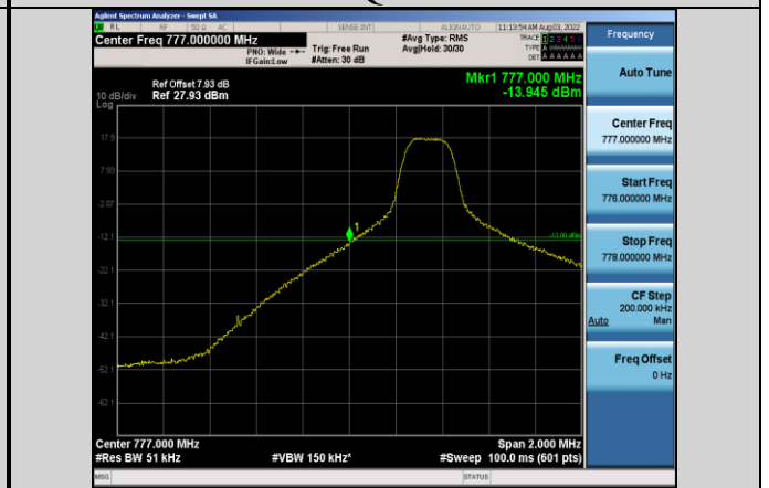
Band13-5MHz-64QAM-23205-1RB#0
