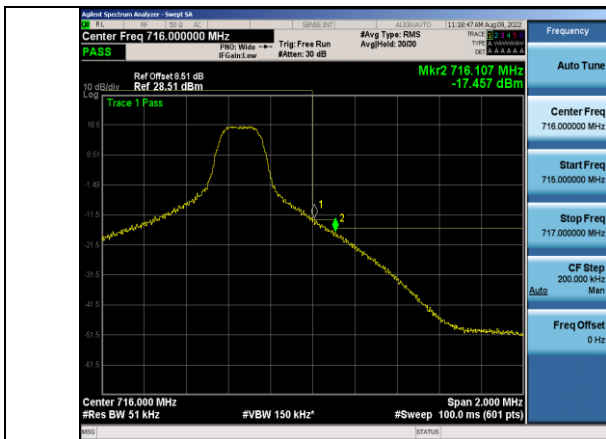
Band17-5MHz-64QAM-23825-1RB#24
