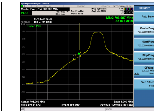
Band17-5MHz-16QAM-23755-1RB#0
