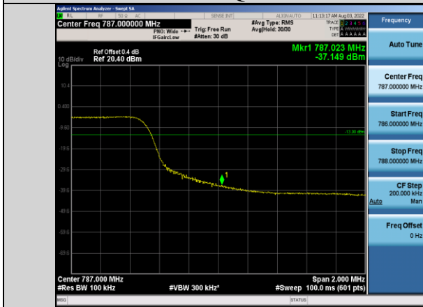
Band13-10MHz-64QAM-23230-50RB#0
