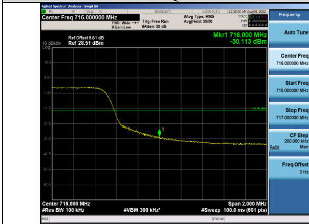
Band17-10MHz-64QAM-23800-50RB#0
