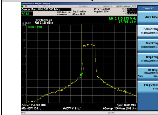
Band26-1.4MHz-16QAM-26697-6RB#0
