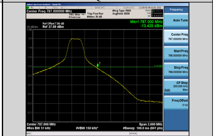
Band13-5MHz-QPSK-23255-1RB#24
