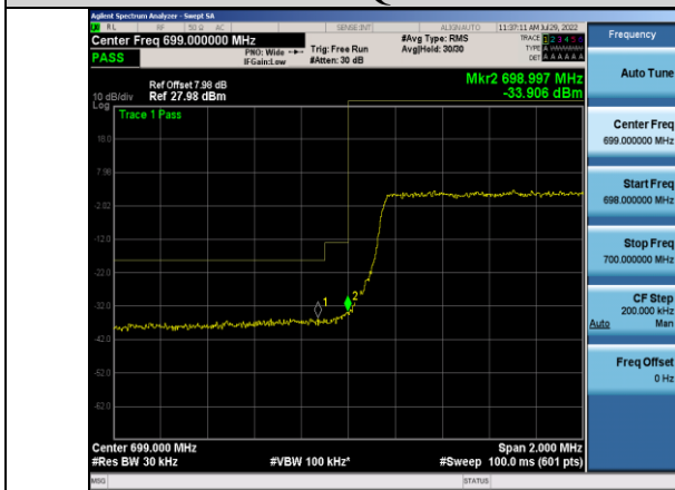
Band12-3MHz-16QAM-23025-15RB#0
