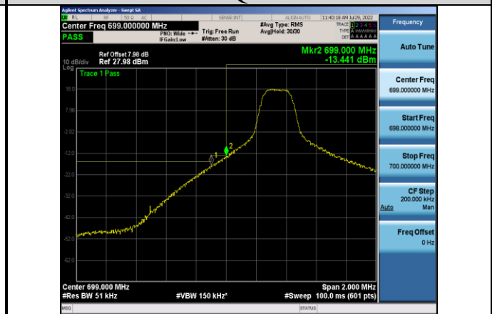
Band12-5MHz-QPSK-23035-1RB#0
