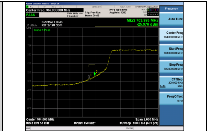
Band17-5MHz-QPSK-23755-25RB#0
