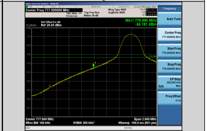
Band13-10MHz-64QAM-23230-1RB#0
