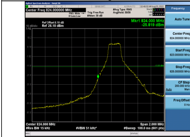
Band5-1.4MHz-64QAM-20407-1RB#0
