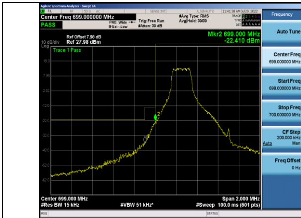
Band12-1.4MHz-QPSK-23017-1RB#0
