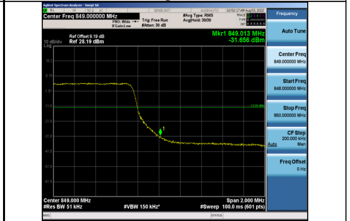
Band5-5MHz-64QAM-20625-25RB#0
