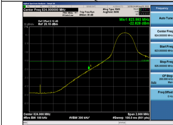
Band5-10MHz-64QAM-20450-1RB#0
