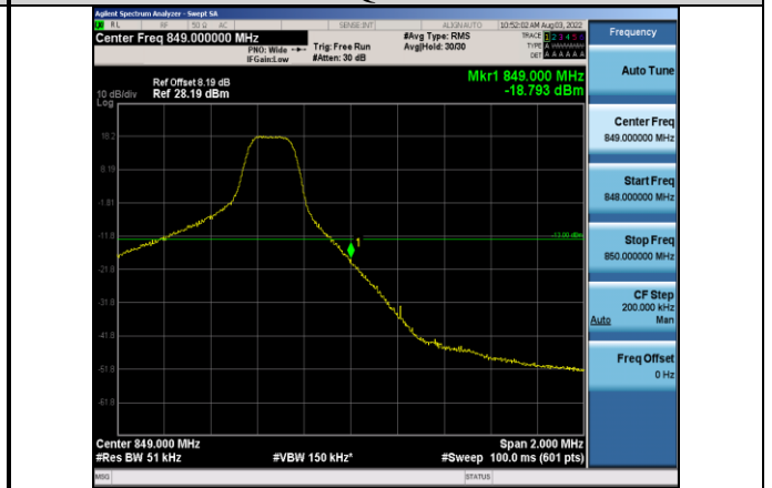
Band5-5MHz-64QAM-20625-1RB#24
