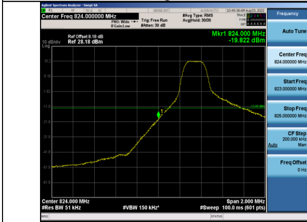
Band5-5MHz-64QAM-20425-1RB#0
