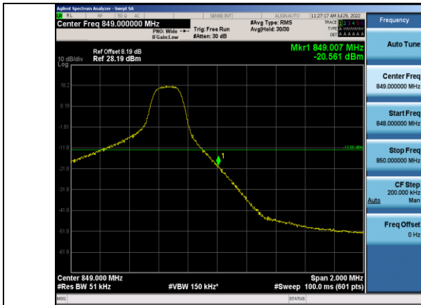
Band5-5MHz-16QAM-20625-1RB#24
