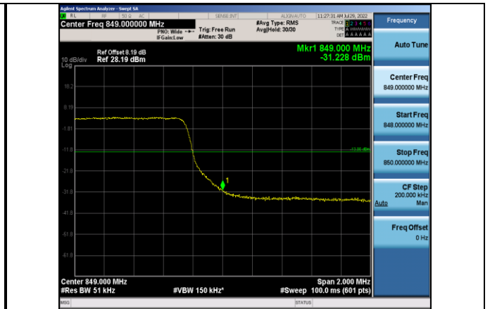
Band5-5MHz-QPSK-20625-25RB#0
