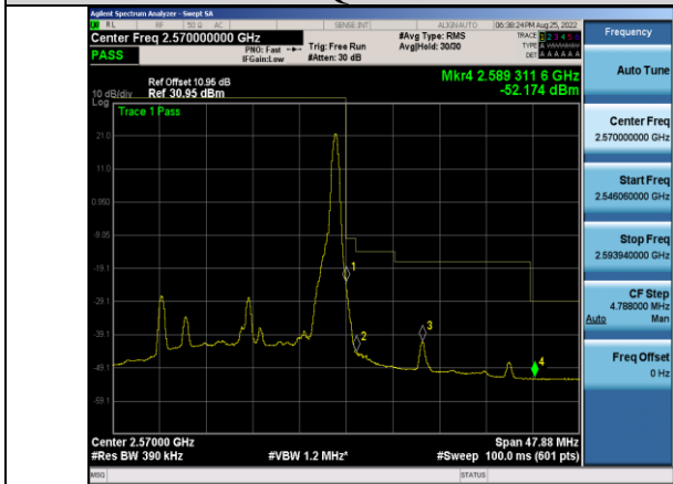
Band7-20MHz-QPSK-21350-1RB#99
