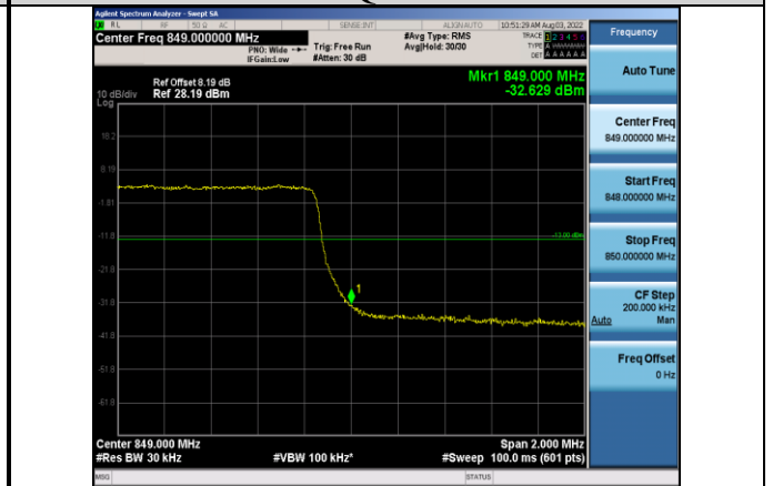
Band5-3MHz-64QAM-20635-15RB#0
