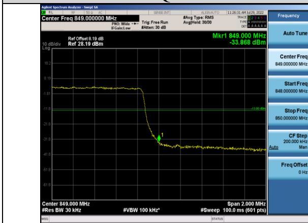
Band5-3MHz-16QAM-20635-15RB#0
