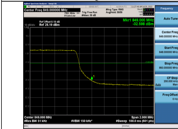
Band5-5MHz-16QAM-20625-25RB#0
