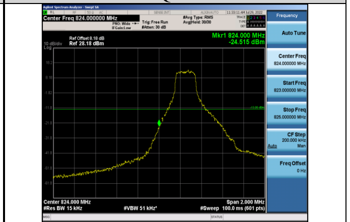
Band5-1.4MHz-16QAM-20407-1RB#0
