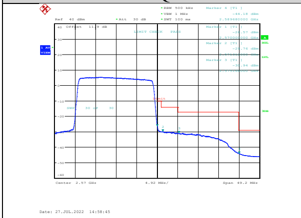
Band7-20MHz-16QAM-21350-100RB#0
