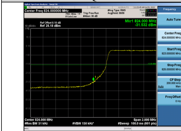
Band5-5MHz-QPSK-20425-25RB#0
