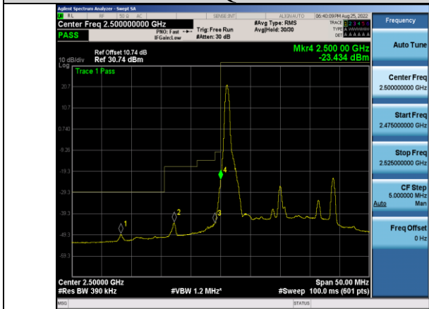
Band7-20MHz-64QAM-20850-1RB#0
