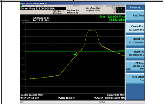
Band5-5MHz-16QAM-20425-1RB#0
