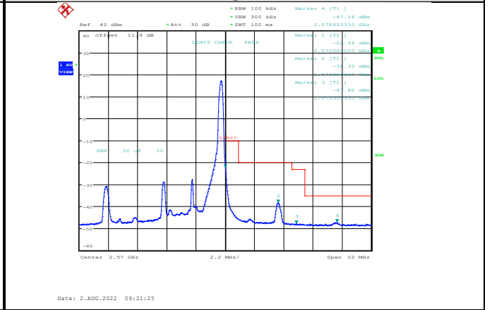
Band7-5MHz-64QAM-21425-1RB#24
