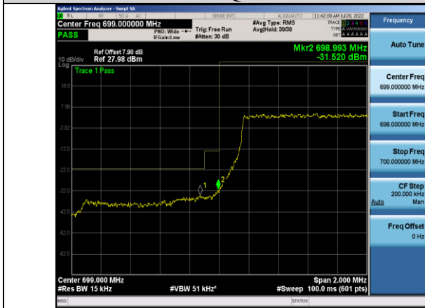
Band12-1.4MHz-QPSK-23017-6RB#0
