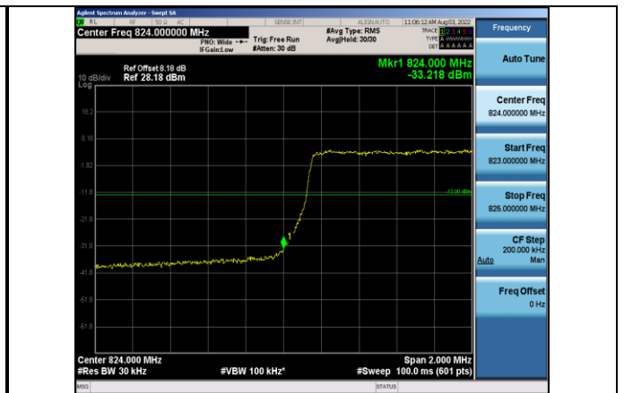
Band5-3MHz-64QAM-20415-15RB#0
