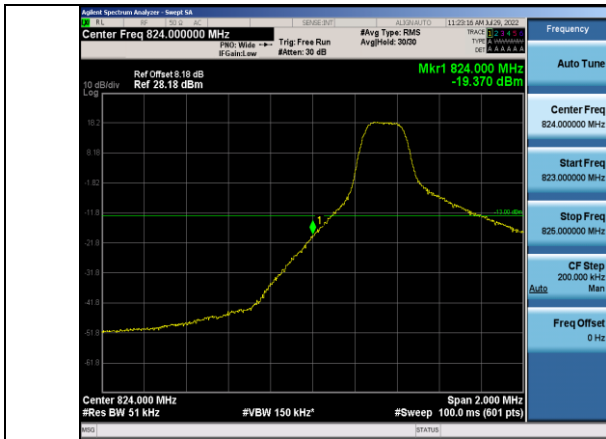
Band5-5MHz-QPSK-20425-1RB#0
