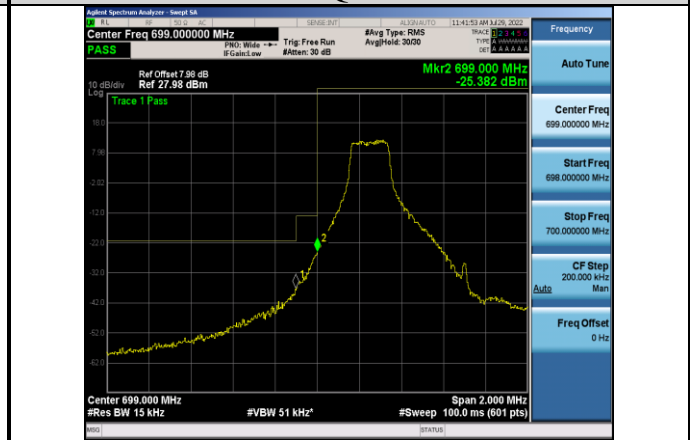
Band12-1.4MHz-16QAM-23017-1RB#0
