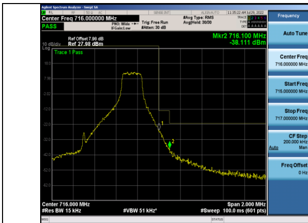
Band12-1.4MHz-16QAM-23173-1RB#5
