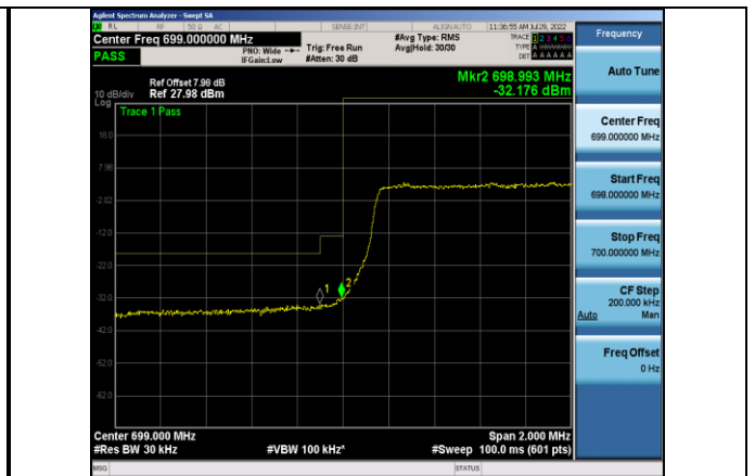
Band12-3MHz-QPSK-23025-15RB#0
