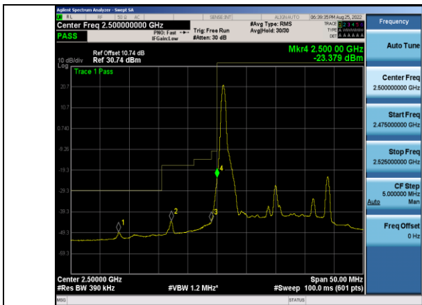
Band7-20MHz-QPSK-20850-1RB#0
