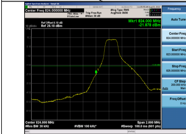
Band5-3MHz-64QAM-20415-1RB#0
