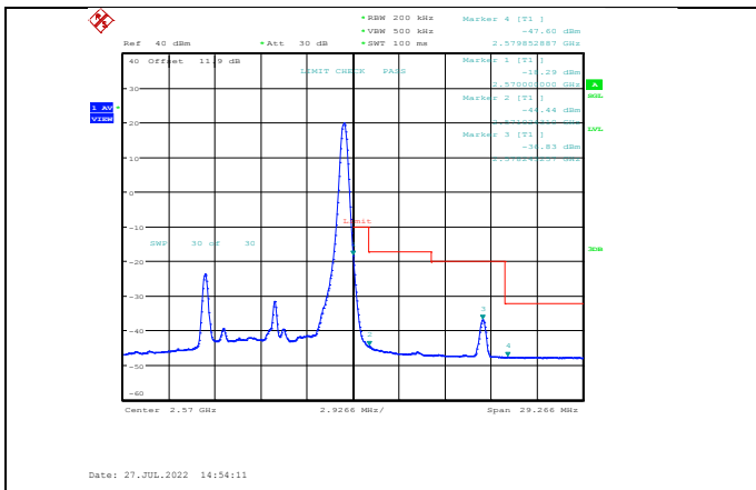
Band7-10MHz-16QAM-21400-1RB#49
