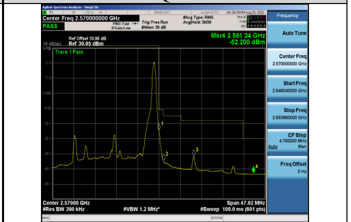
Band7-20MHz-64QAM-21350-1RB#99
