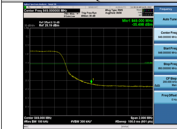
Band5-10MHz-16QAM-20600-50RB#0
