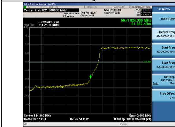
Band5-1.4MHz-QPSK-20407-6RB#0
