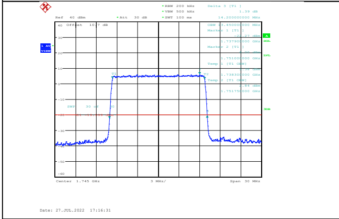
Band66-15MHz-QPSK-132322-75RB#0
