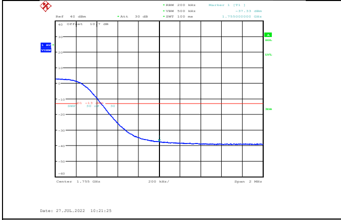
Band4-15MHz-16QAM-20325-75RB#0
