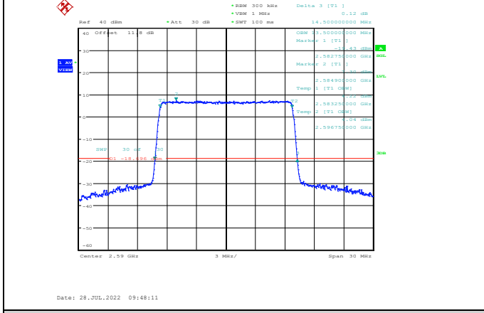
Band41-15MHz-QPSK-40590-75RB#0
