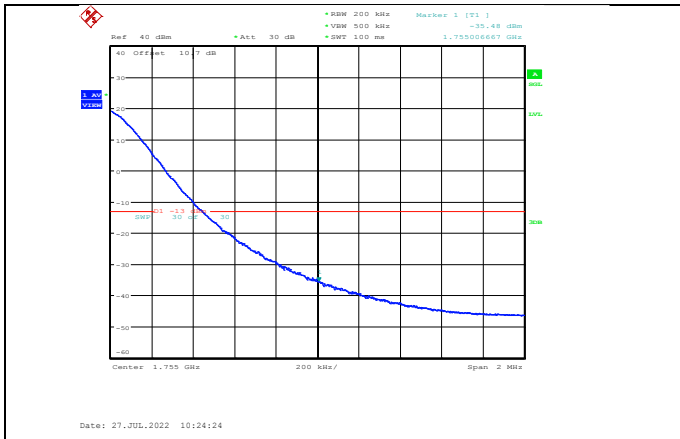
Band4-20MHz-16QAM-20300-1RB#99
