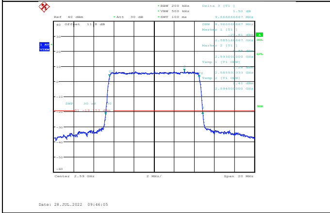
Band41-10MHz-16QAM-40590-50RB#0
