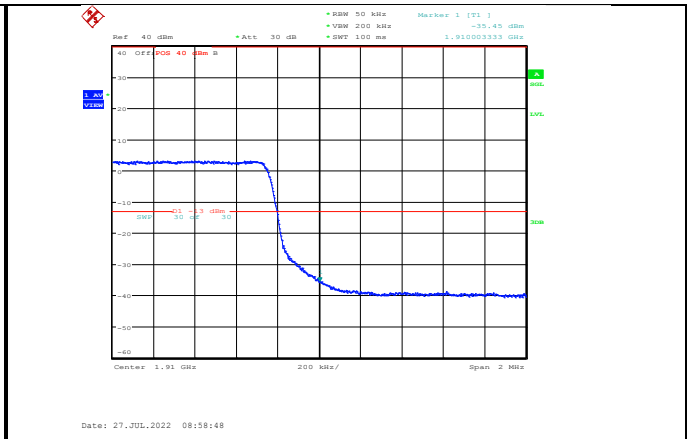
Band2-5MHz-QPSK-19175-25RB#0
