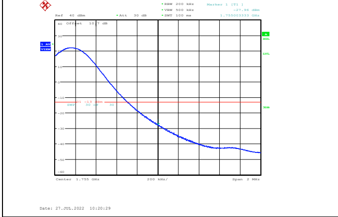
Band4-15MHz-QPSK-20325-1RB#74
