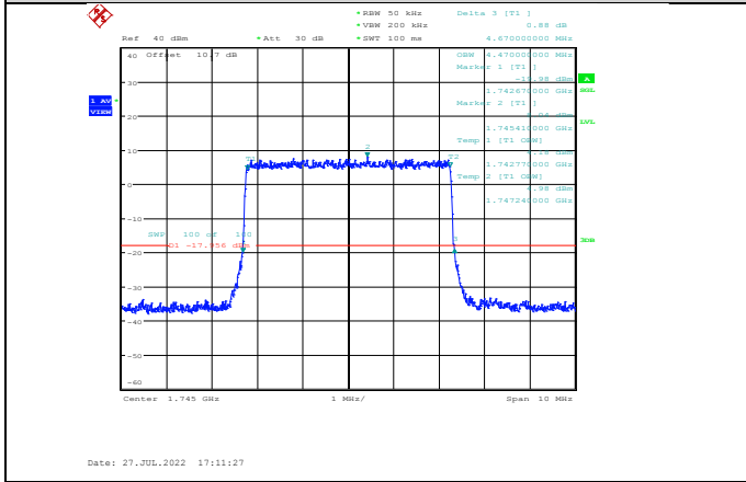
Band66-5MHz-QPSK-132322-25RB#0
