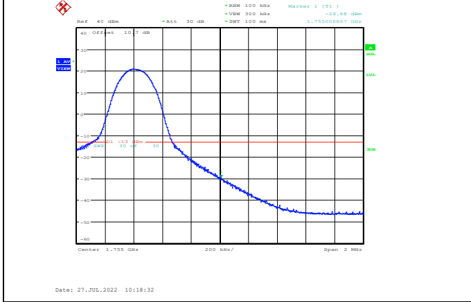
Band4-10MHz-QPSK-20350-1RB#49
