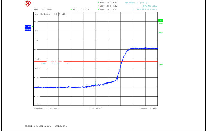
Band4-10MHz-16QAM-20000-50RB#0
