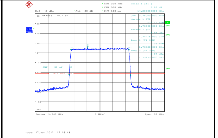
Band66-15MHz-16QAM-132322-75RB#0
