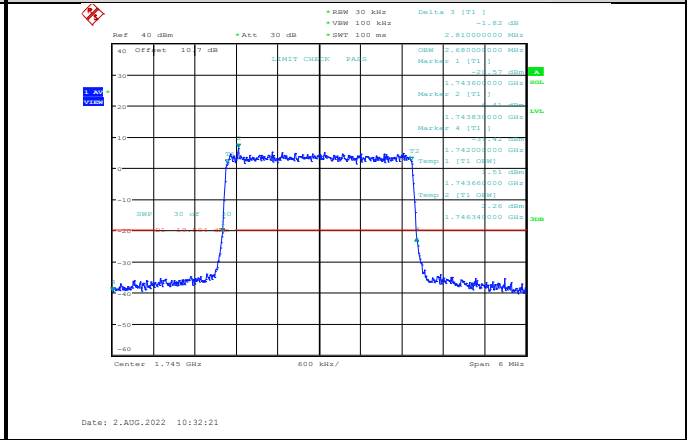
Band66-3MHz-64QAM-132322-15RB#0
