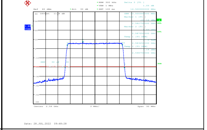
Band41-15MHz-16QAM-40590-75RB#0
