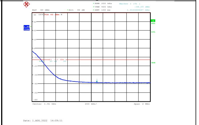
Band2-20MHz-64QAM-19100-100RB#0
