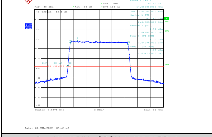
Band41-15MHz-QPSK-41165-75RB#0
