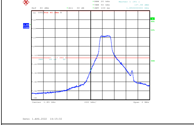
Band2-1.4MHz-16QAM-18607-1RB#0
