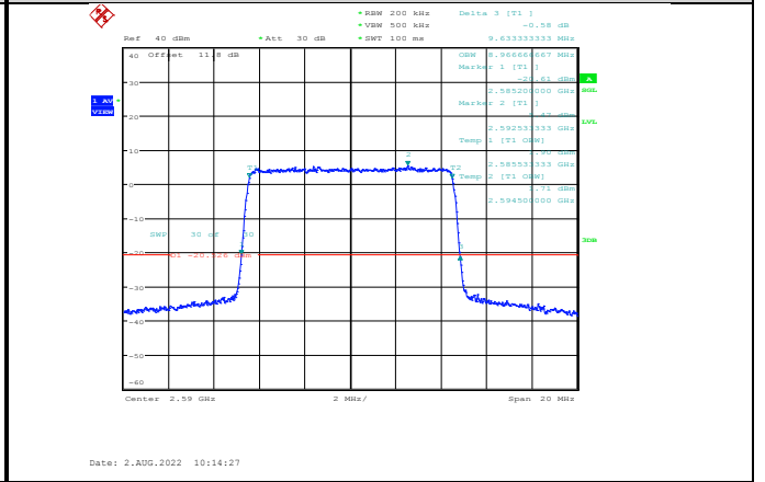
Band41-10MHz-64QAM-40590-50RB#0
