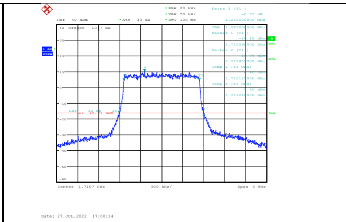
Band66-1.4MHz-16QAM-131979-6RB#0
