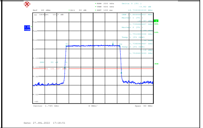
Band66-20MHz-QPSK-132322-100RB#0
