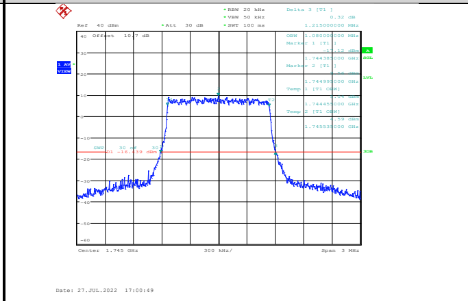
Band66-1.4MHz-16QAM-132322-6RB#0
