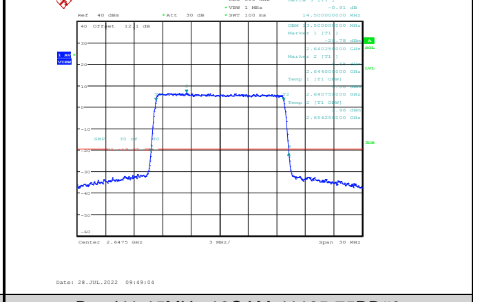
Band41-15MHz-16QAM-41165-75RB#0
