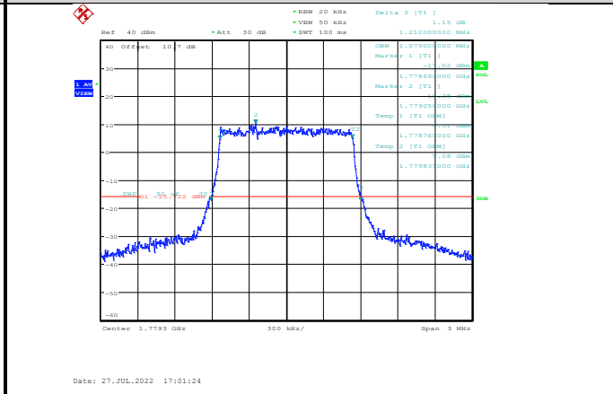
Band66-1.4MHz-16QAM-132665-6RB#0
