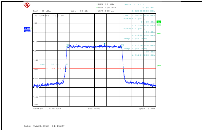
Band66-3MHz-16QAM-131987-15RB#0
