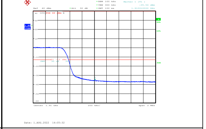
Band2-10MHz-64QAM-18650-1RB#0
