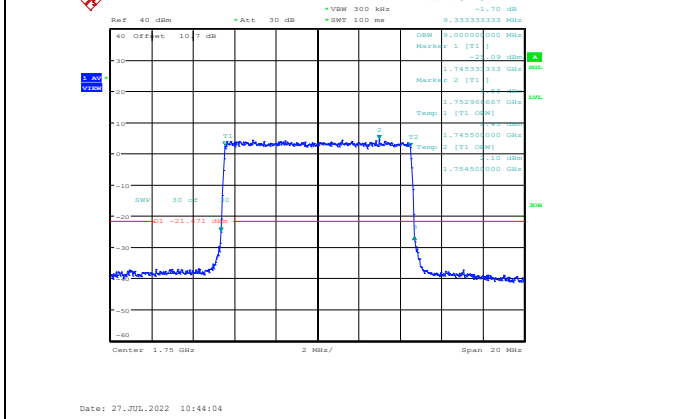
Band4-10MHz-16QAM-20350-50RB#0
