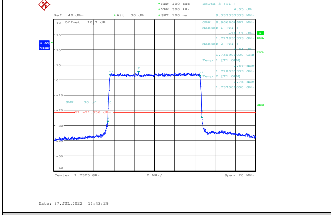
Band4-10MHz-16QAM-20175-50RB#0
