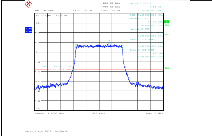
Band2-1.4MHz-64QAM-19193-6RB#0
