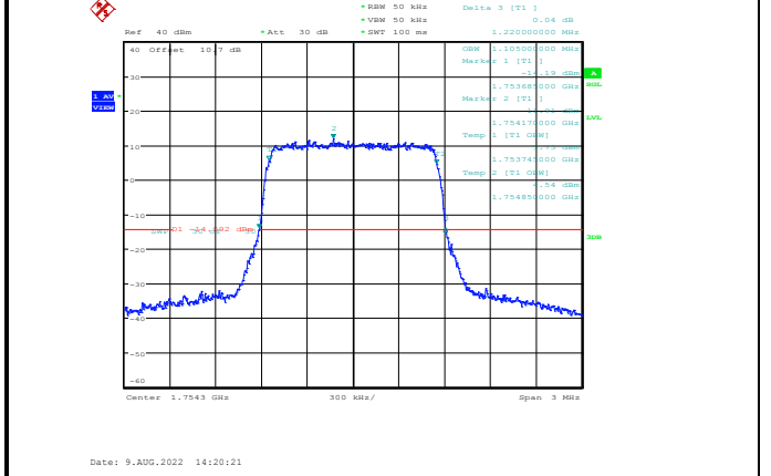
Band4-1.4MHz-16QAM-20393-6RB#0
