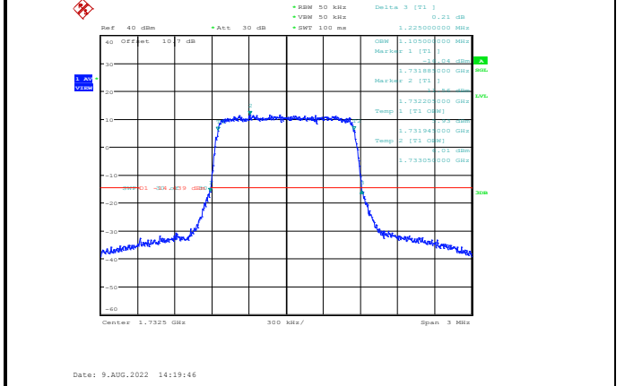
Band4-1.4MHz-16QAM-20175-6RB#0
