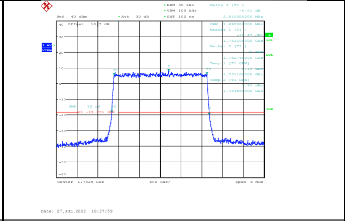
Band4-3MHz-QPSK-20175-15RB#0
