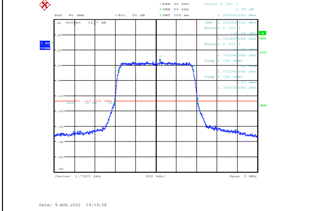
Band4-1.4MHz-QPSK-20175-6RB#0
