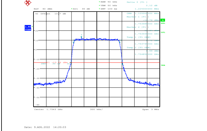
Band4-1.4MHz-QPSK-20393-6RB#0
