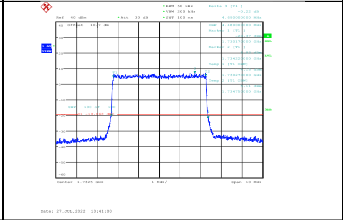
Band4-5MHz-16QAM-20175-25RB#0
