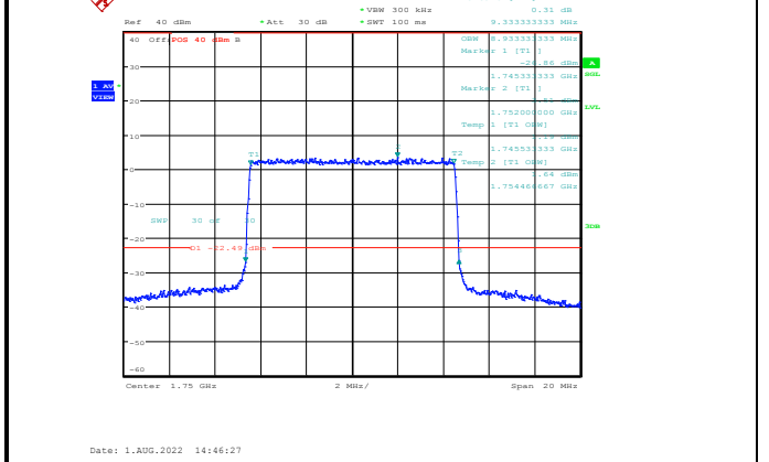
Band4-10MHz-64QAM-20350-50RB#0
