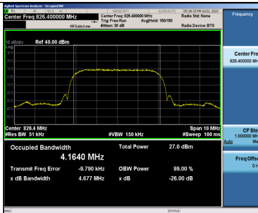
Band V-4132-4.677
