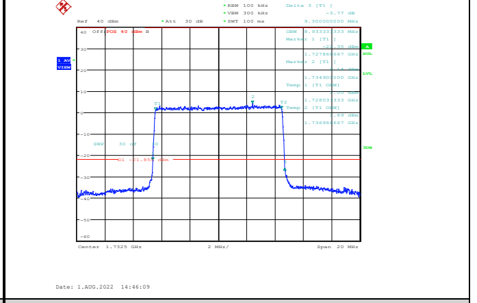
Band4-10MHz-64QAM-20175-50RB#0
