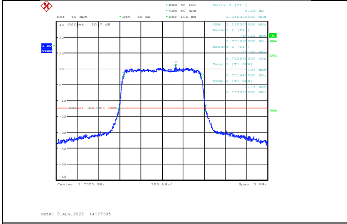
Band4-1.4MHz-64QAM-20175-6RB#0
