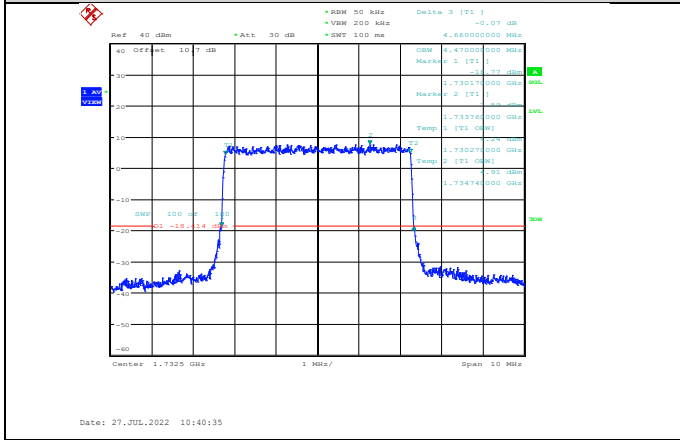
Band4-5MHz-QPSK-20175-25RB#0
