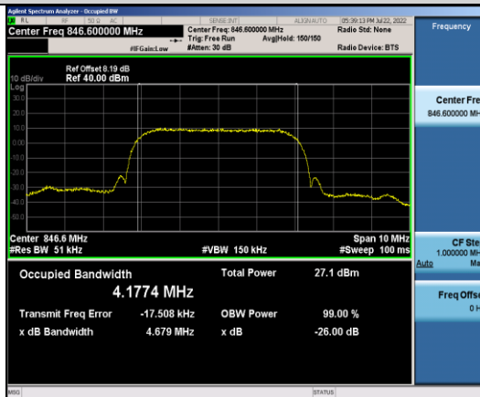
Band V-4233-4.679
