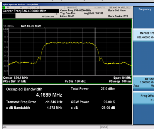
Band V-4182-4.678
