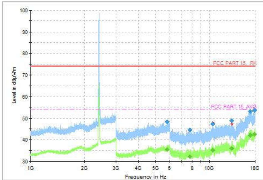
Fig.86 Radiated Spurious Emission (802.11g, CH1, 1GHz-18GHz)
