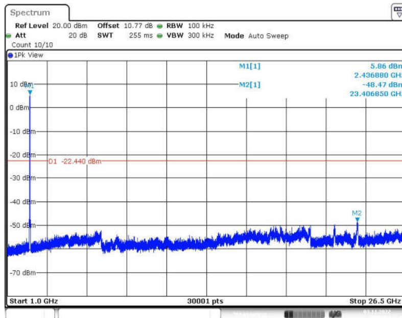
Fig.63 Conducted Spurious Emission (1GHz-26.5GHz, 802.11n-HT20, CH6)
