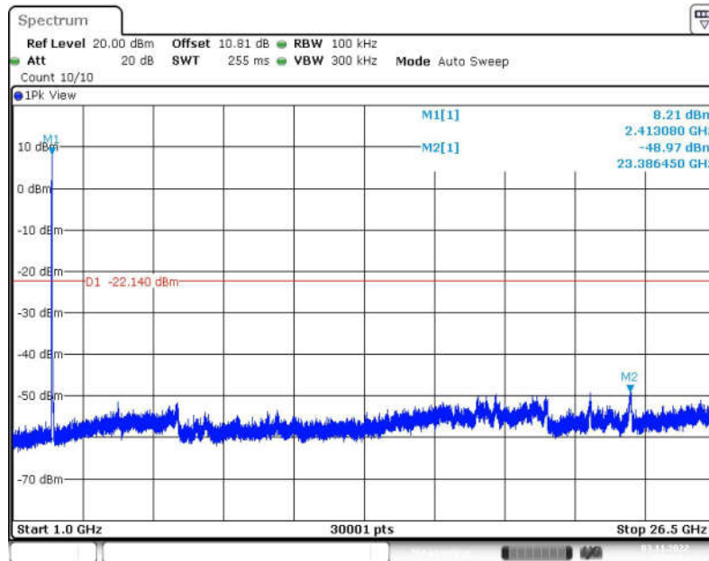
Fig.62 Conducted Spurious Emission (1GHz-26.5GHz, 802.11n-HT20, CH1)
