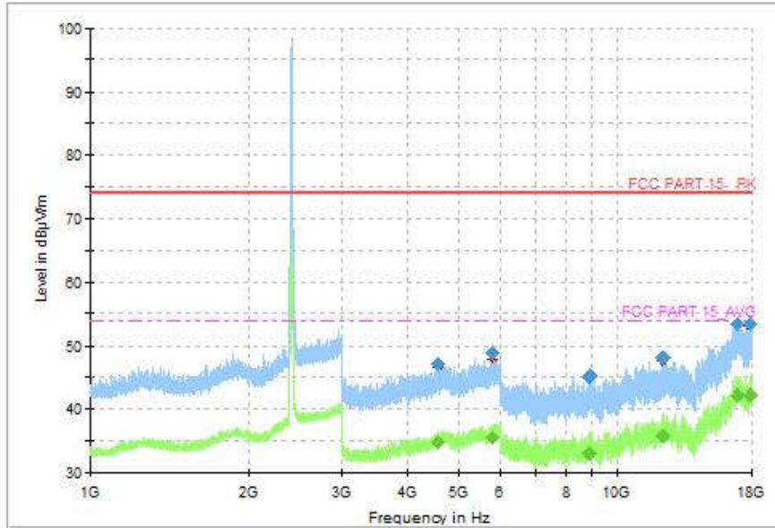
Fig.91 Radiated Spurious Emission (802.11n-HT20, CH1, 1GHz-18GHz)
