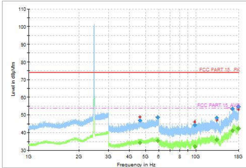
Fig.83 Radiated Spurious Emission (802.11b, CH11, 1GHz-18GHz)
