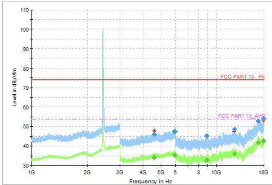
Fig.87 Radiated Spurious Emission (802.11g, CH6, 1GHz-18GHz)
