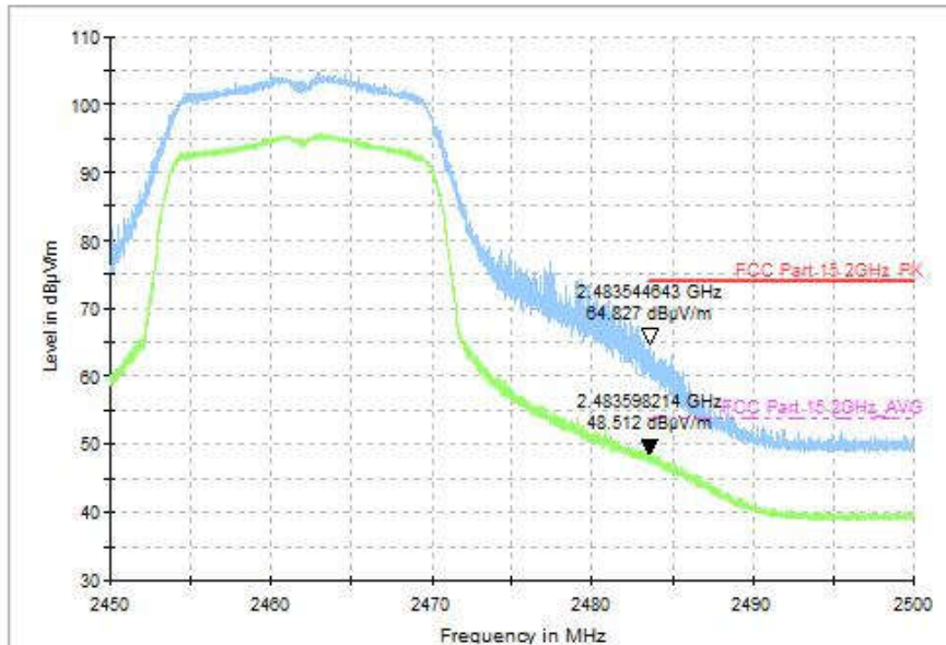
Fig.90 Radiated Restricted Band (802.11g, CH11, 2.45GHz~2.50GHz)
