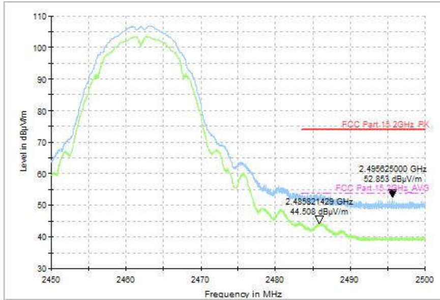
Fig.85 Radiated Restricted Band (802.11b, CH11, 2.45GHz~2.50GHz)
