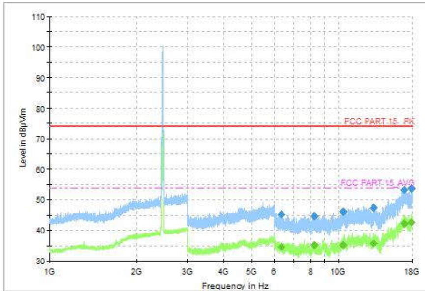
Fig.98 Radiated Spurious Emission (802.11-VHT20, CH11, 1GHz-18GHz)
