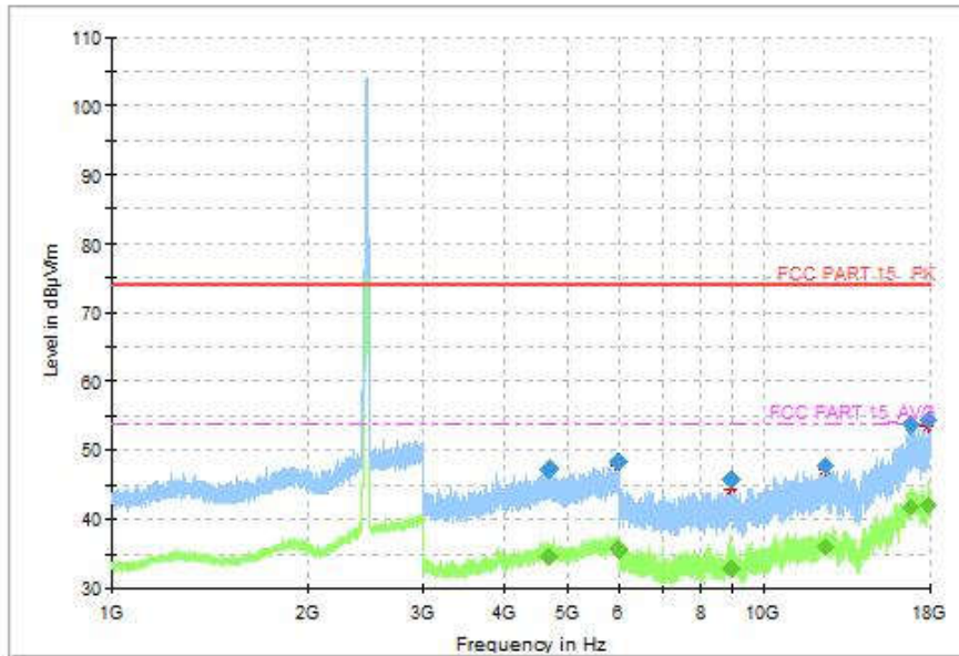
Fig.88 Radiated Spurious Emission (802.11g, CH11, 1GHz-18GHz)
