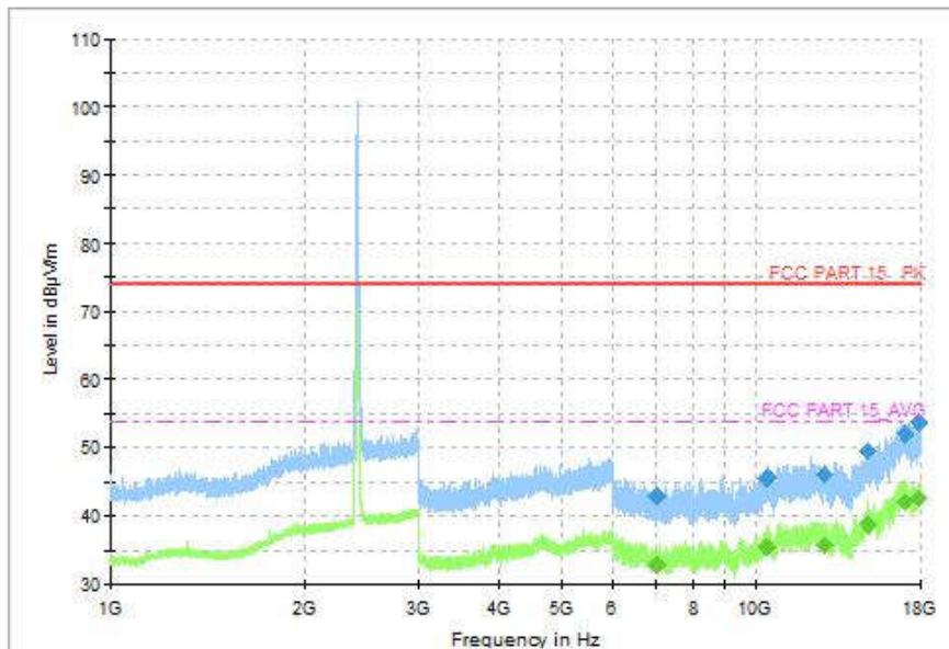
Fig.96 Radiated Spurious Emission (802.11-VHT20, CH1, 1GHz-18GHz)
