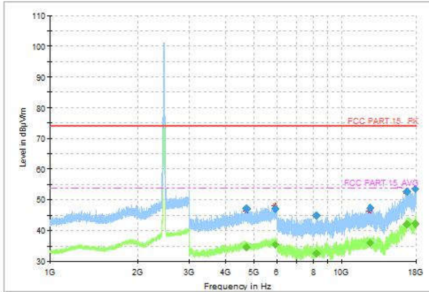
Fig.93 Radiated Spurious Emission (802.11n-HT20, CH11, 1GHz-18GHz)
