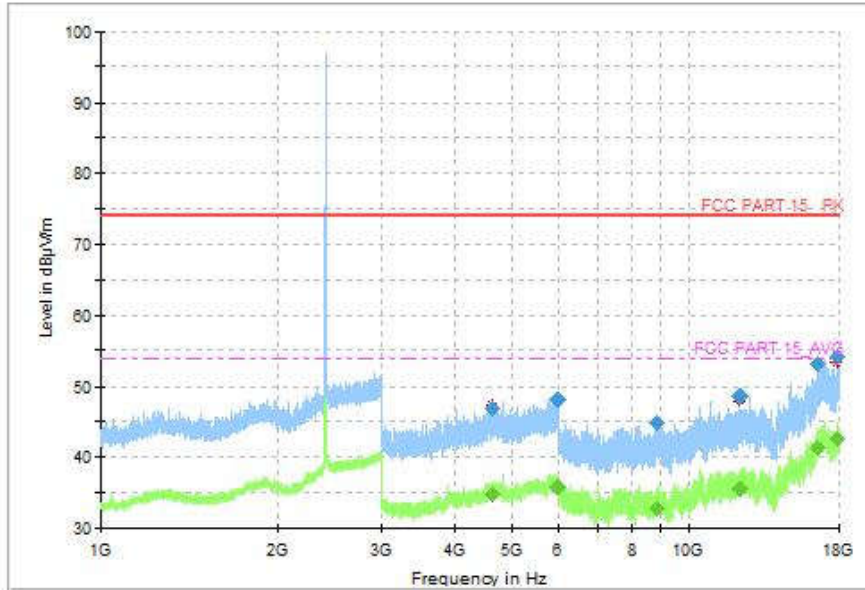
Fig.81 Radiated Spurious Emission (802.11b, CH1, 1GHz-18GHz)
