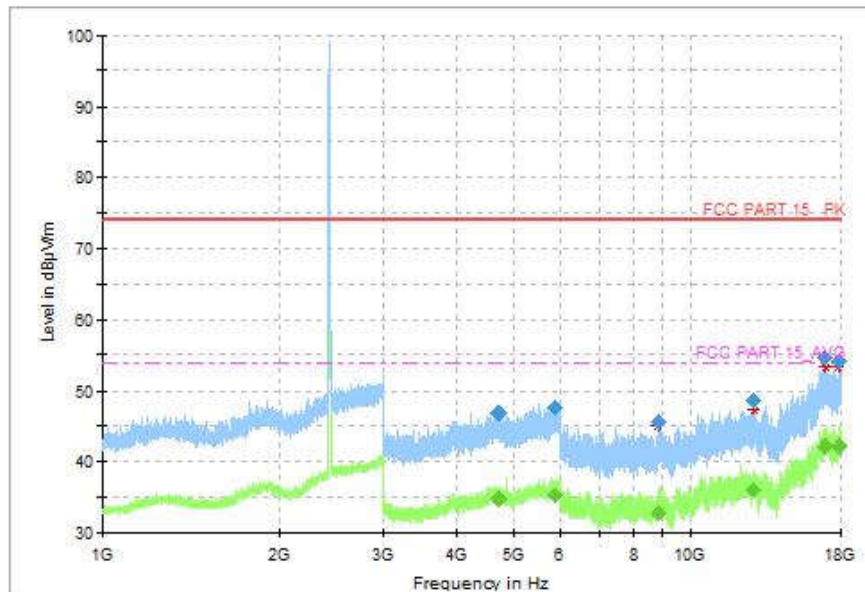
Fig.82 Radiated Spurious Emission (802.11b, CH6, 1GHz-18GHz)
