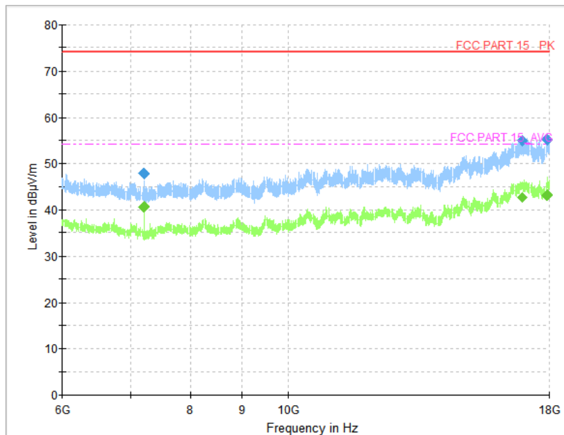
Fig. 41 Radiated Spurious Emission (GFSK, CH0, 6 GHz ~18 GHz)
