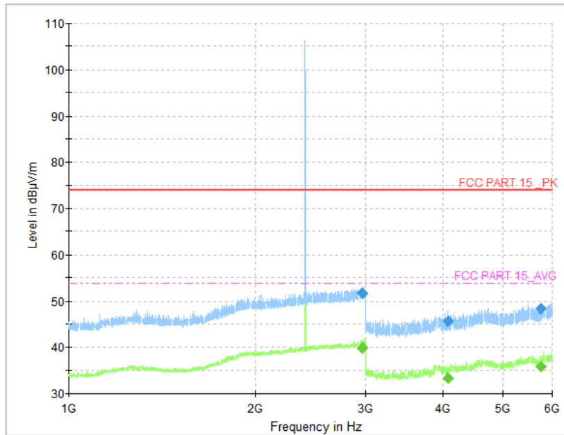
Fig. 40 Radiated Spurious Emission (GFSK, CH0, 1 GHz ~6 GHz)
