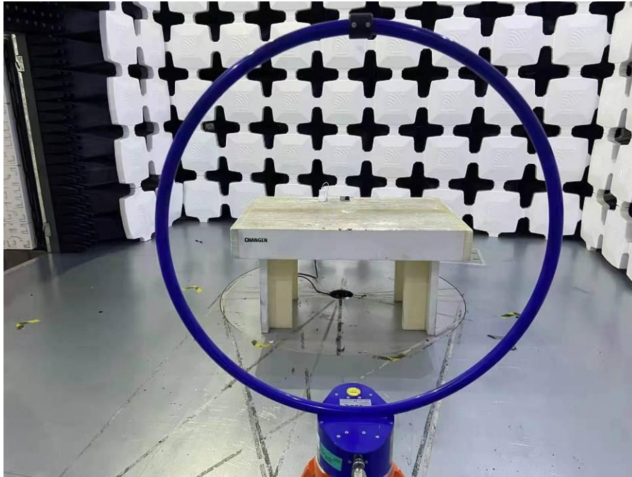
17. Radiated Emissions (Part 15C&Part 15E, 9kHz-30MHz)
