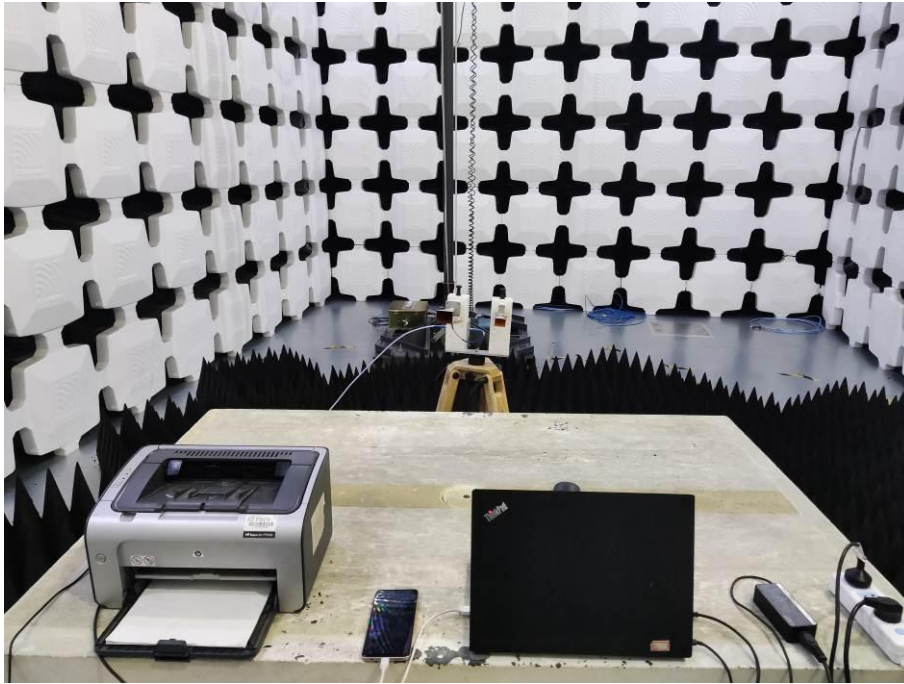
7. Radiated Emissions (Part 15B, Leather Material Shell, Data Transfer, 18GHz-26.5GHz)
