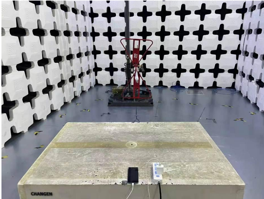
9. Radiated Emissions (Part 15B, Camera/Video Player/GSM receiver/WCDMA receiver/LTE receiver,30MHz-1GHz)
