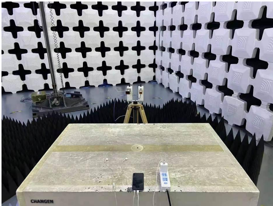
16. Radiated Emissions (Part 15B, FM receiver,26.5GHz-40GHz)
