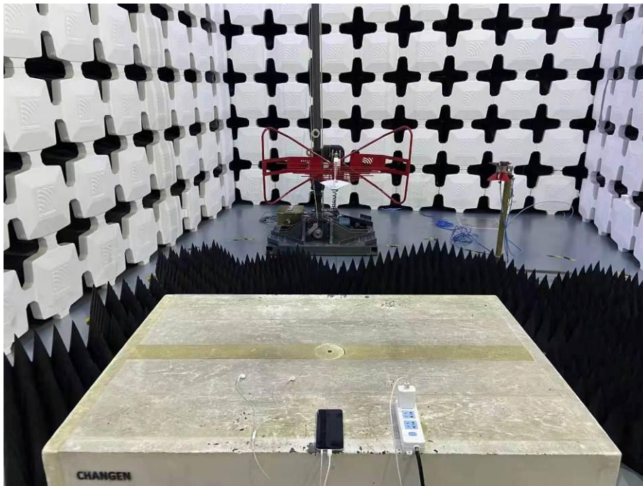
14. Radiated Emissions (Part 15B, FM receiver,1GHz-18GHz)
