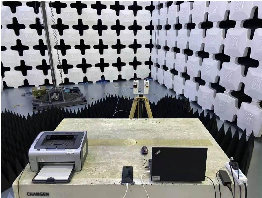
3. Radiated Emissions (Part 15B, Plate Material Shell, Data Transfer, 18GHz-26.5GHz)
