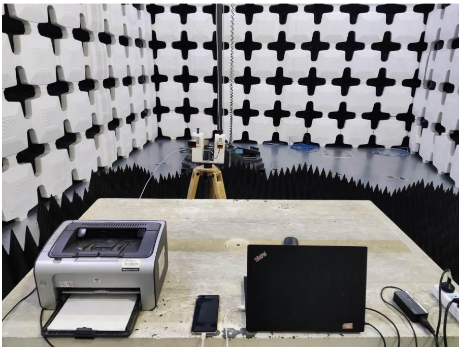
8. Radiated Emissions (Part 15B, Leather Material Shell, Data Transfer, 26.5GHz-40GHz)
