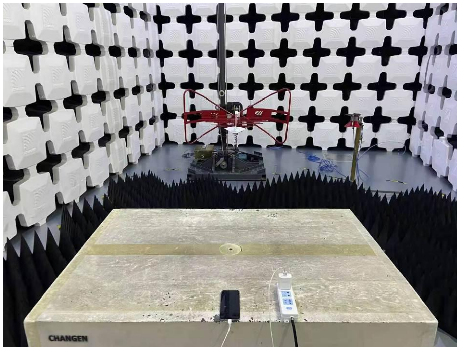
10. Radiated Emissions (Part 15B, Camera/Video Player/GSM receiver/WCDMA receiver/LTE receiver,1GHz-18GHz)
