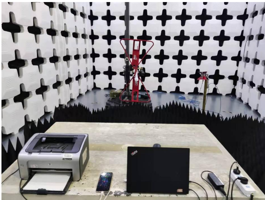
6. Radiated Emissions (Part 15B, Leather Material Shell, Data Transfer, 1GHz-18GHz)
