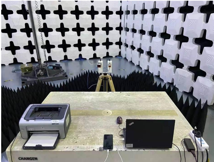
4. Radiated Emissions (Part 15B, Plate Material Shell, Data Transfer, 26.5GHz-40GHz)
