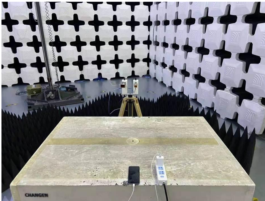
12. Radiated Emissions (Part 15B, Camera/Video Player/GSM receiver/WCDMA receiver/LTE receiver, 26.5GHz-40GHz)
