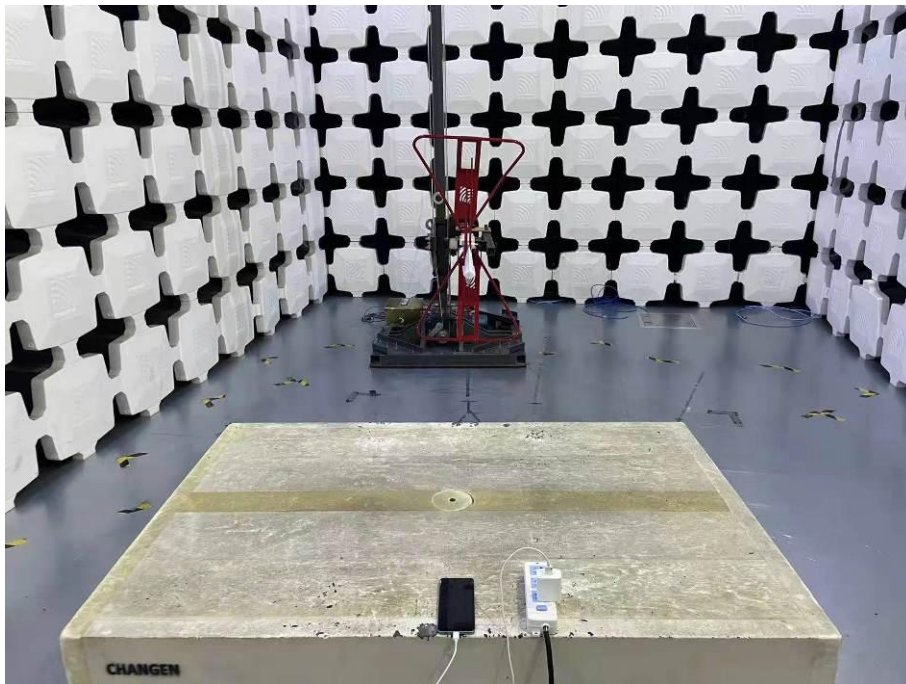
18. Radiated Emissions (Part 15C&Part 15E,30MHz-1GHz)
