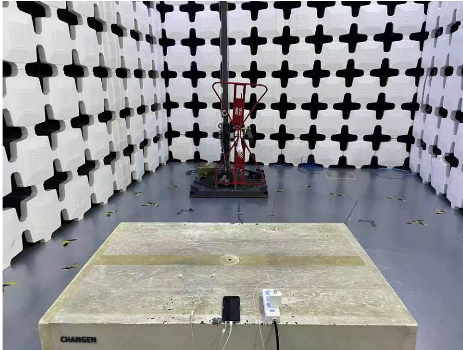
13. Radiated Emissions (Part 15B, FM receiver,30MHz-1GHz)
