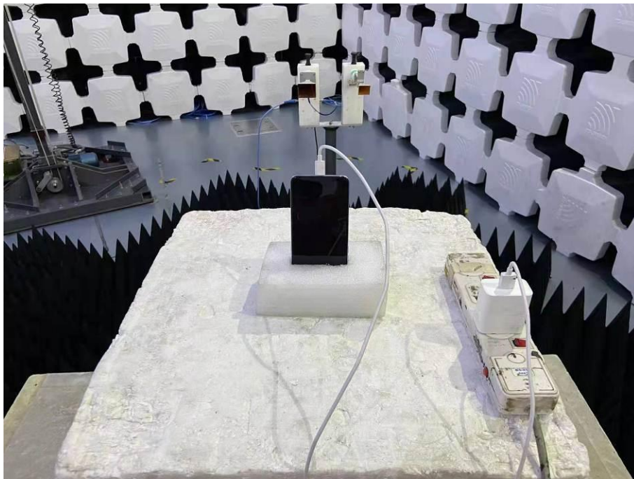
20. Radiated Emissions (Part 15C&Part 15E, 18GHz -26.5GHz)
