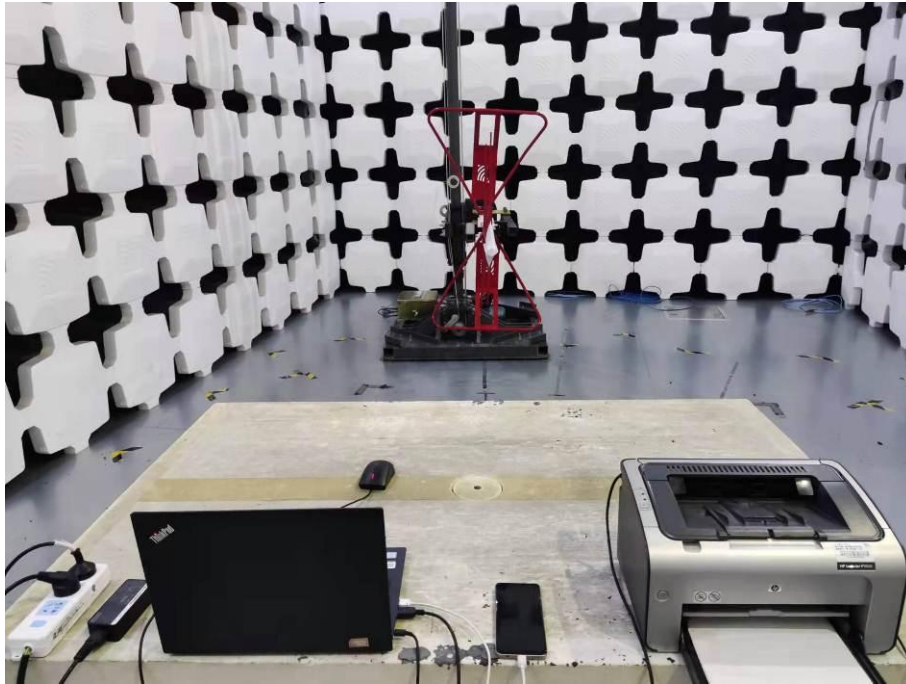
5. Radiated Emissions (Part 15B, Leather Material Shell, Data Transfer, 30MHz-1GHz)
