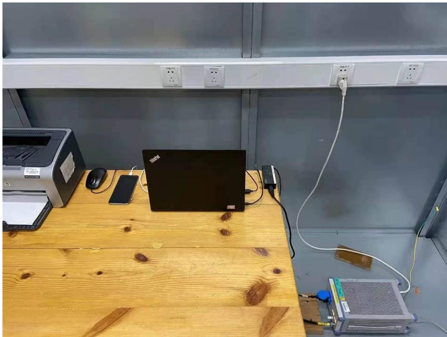
26. Conducted Emission (Part 15B& Part 15C&E)
