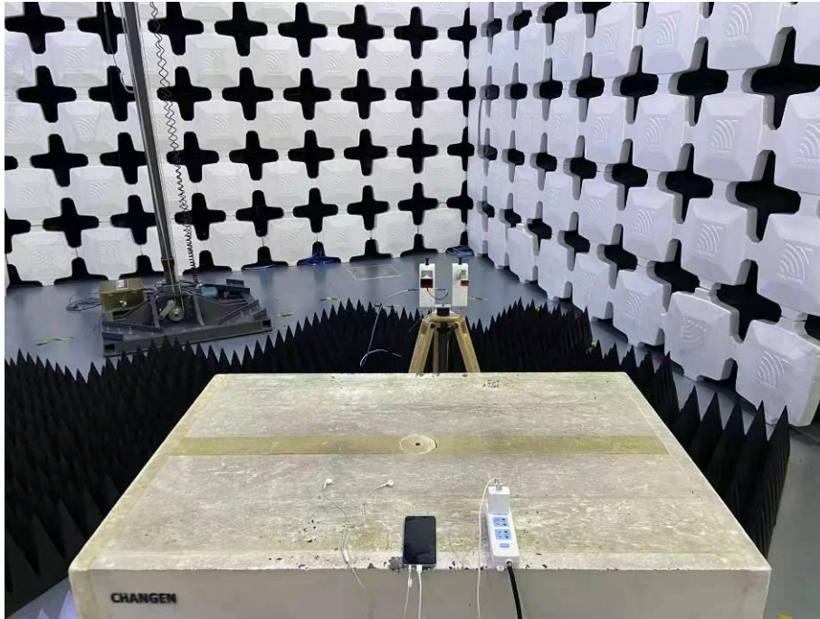
15. Radiated Emissions (Part 15B, FM receiver,18GHz-26.5GHz)
