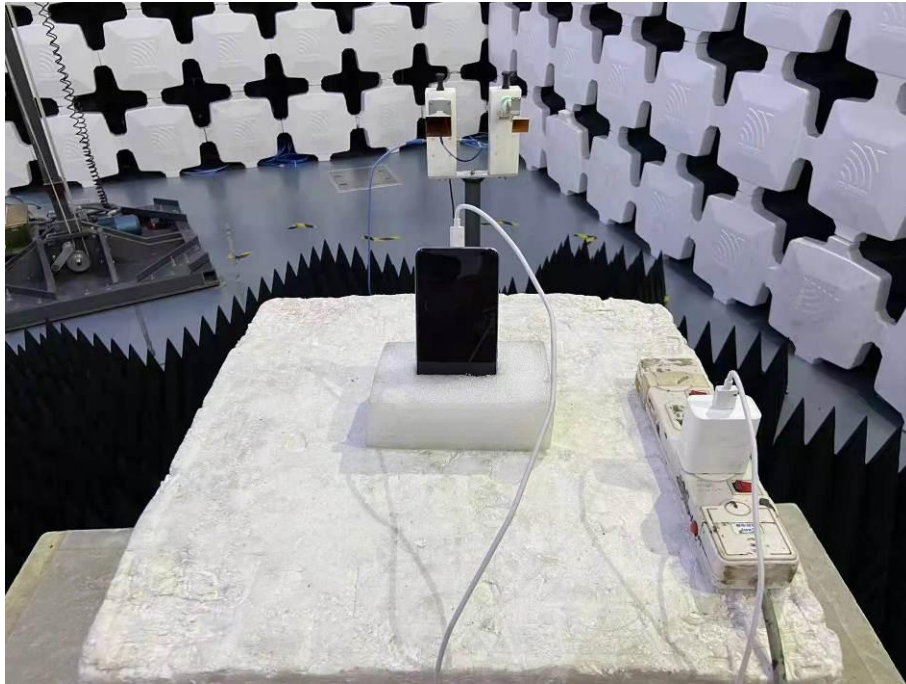
23. Radiated Emissions (Part 22/24/27/90, 18GHz-26.5GHz)
