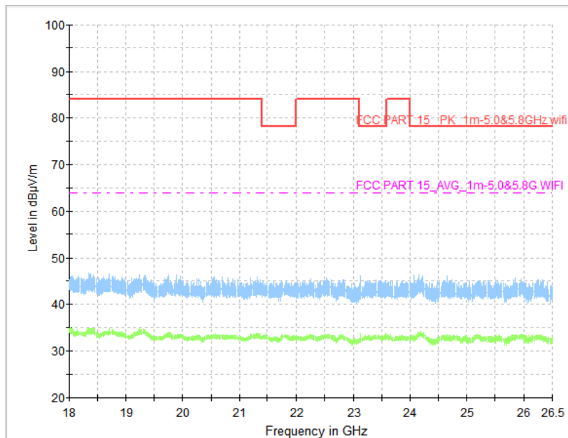
Fig. 107 Transmitter Spurious Emission (All channel, 18GHz~26.5GHz)
