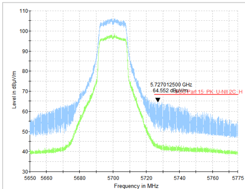
Fig. 66 Band Edges (802.11a, CH140 5700MHz)
