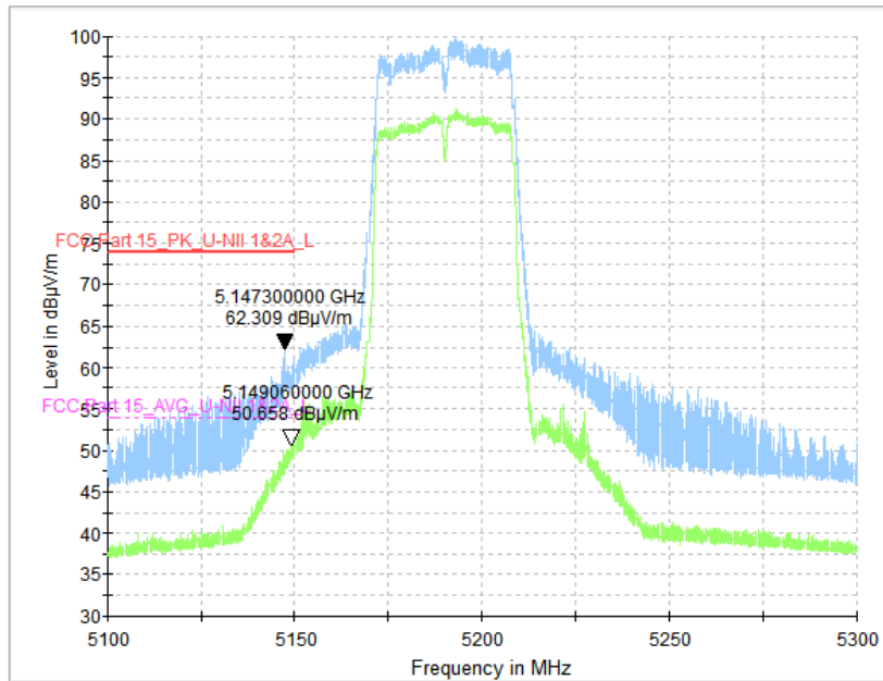
Fig. 69 Band Edges (802.11ac-VHT40, CH38 5190MHz)
