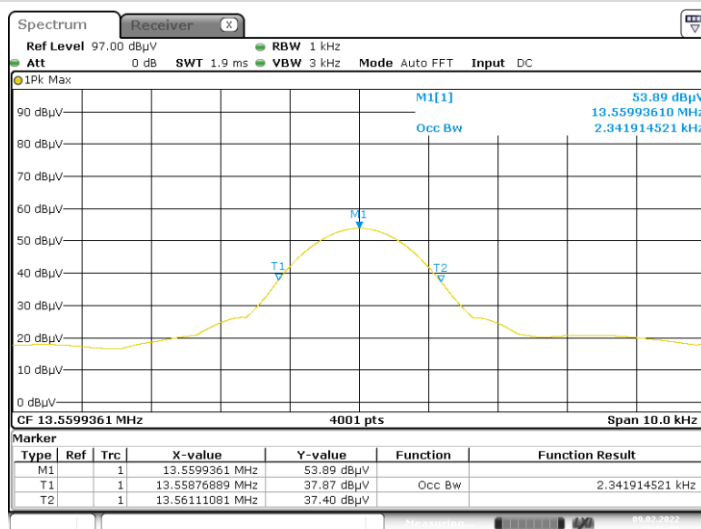
99% Occupied Bandwidth
