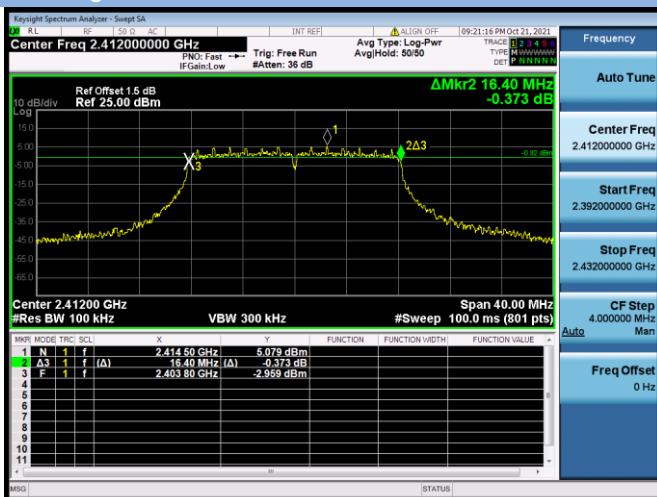
802.11g CHANNEL 1
