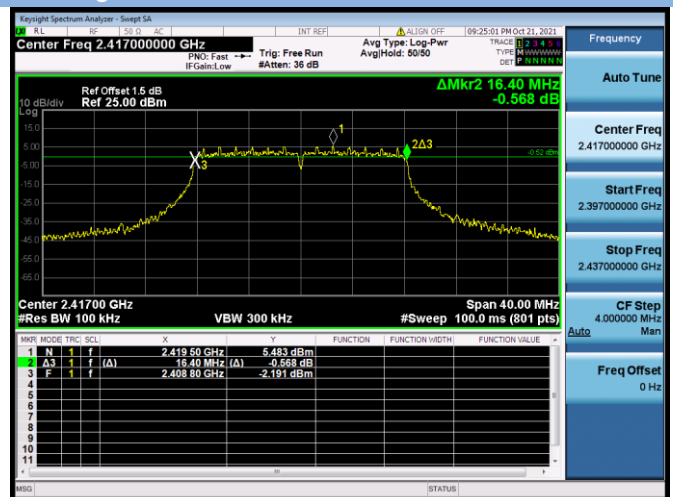
802.11g CHANNEL 2
