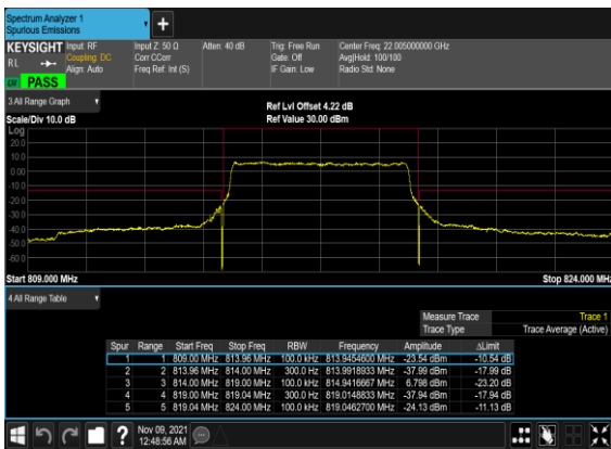
N26(5M)_DFT-s-OFDM_QPSK_Outer_Full_Low_CH
