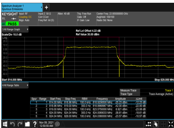
N26(5M)_DFT-s-OFDM_QPSK_Outer_Full_High_CH
