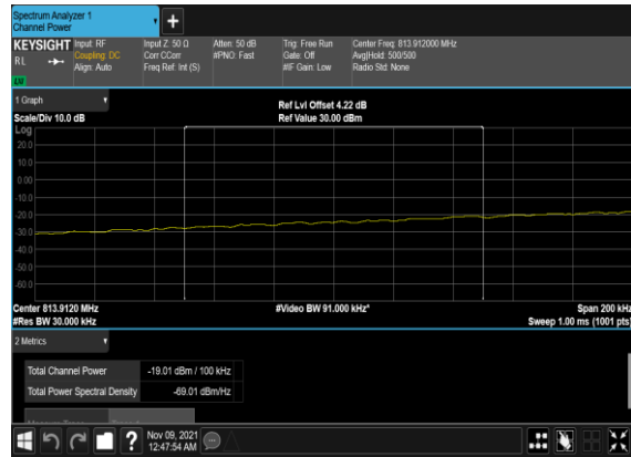
N26(5M)_DFT-s-OFDM_QPSK_Edge_1RB_Left_Low_CH_CHP_PASS
