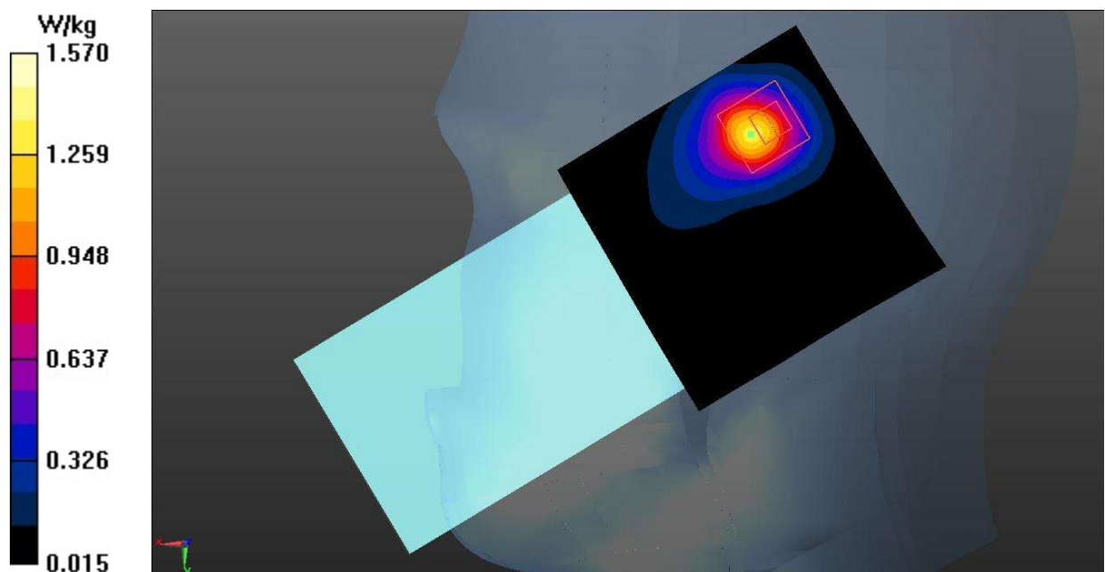
Fig.23 LTE Band 38
