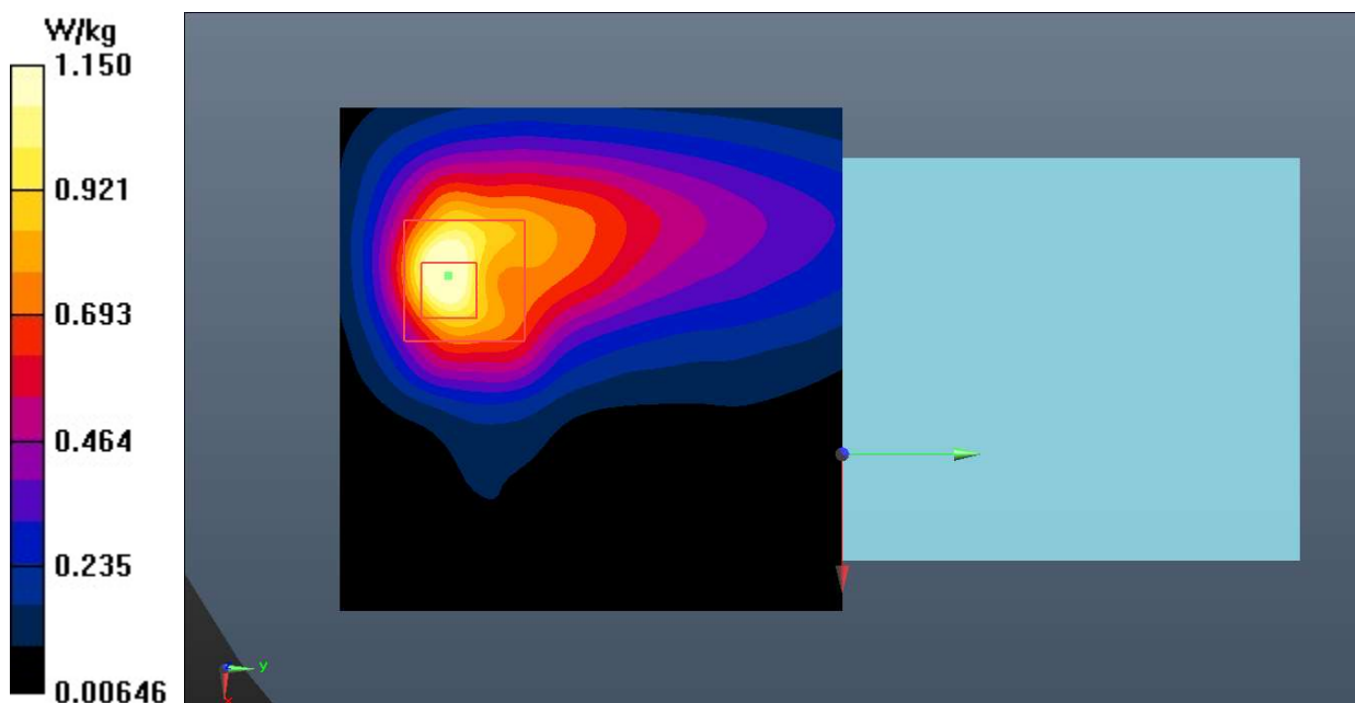
Fig.24 LTE Band 38
