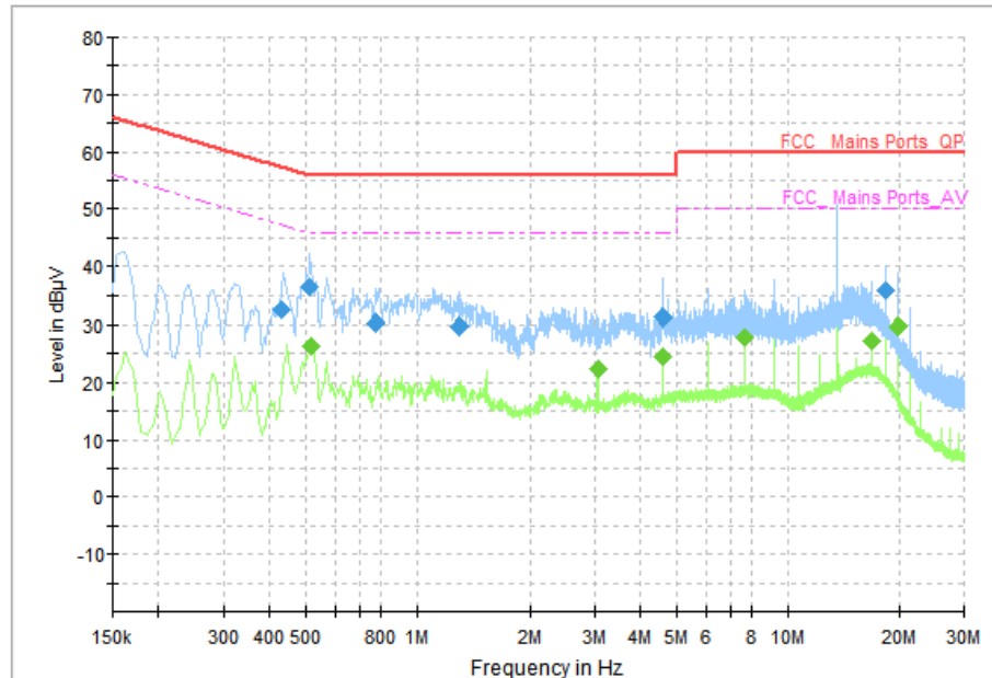
Figure A-5 Conducted Emission (Traffic)-AE4,AE5,AE6
