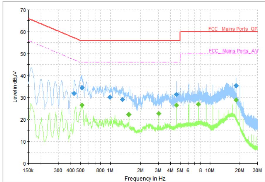
Figure A-6 Conducted Emission (Idle)-AE4,AE5,AE6
