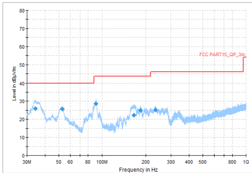
Fig. 56 Radiated Spurious Emission (All Channels, 30 MHz ~1 GHz)
