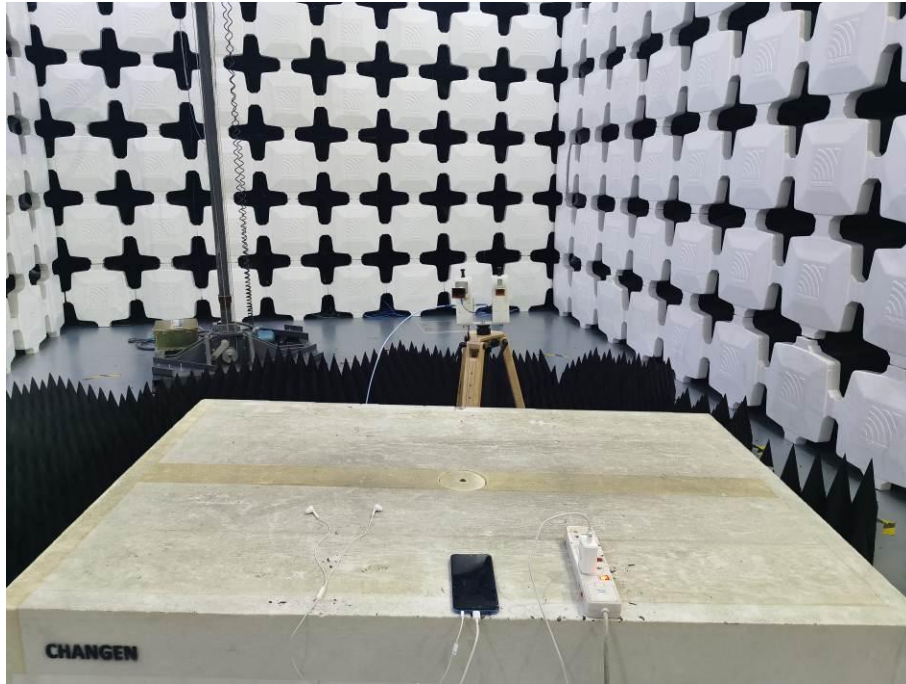
7. Radiated Emissions (Part 15B Camera/Video Player/FM receiver/GSM receiver/WCDMA receiver/LTE receiver,26.5GHz-40GHz)
