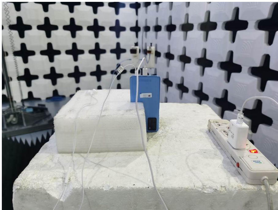
16. Radiated Emissions (Part 22/24/27/90, 26.5GHz-40GHz)
