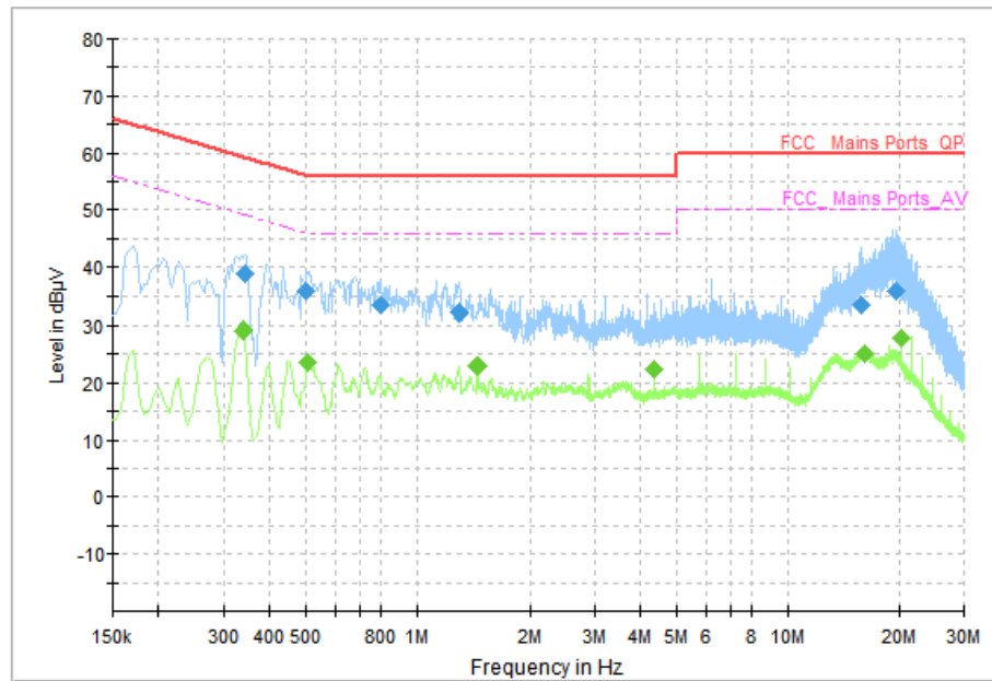
Fig.55 AC Power line Conducted Emission (Traffic), LE 1M
