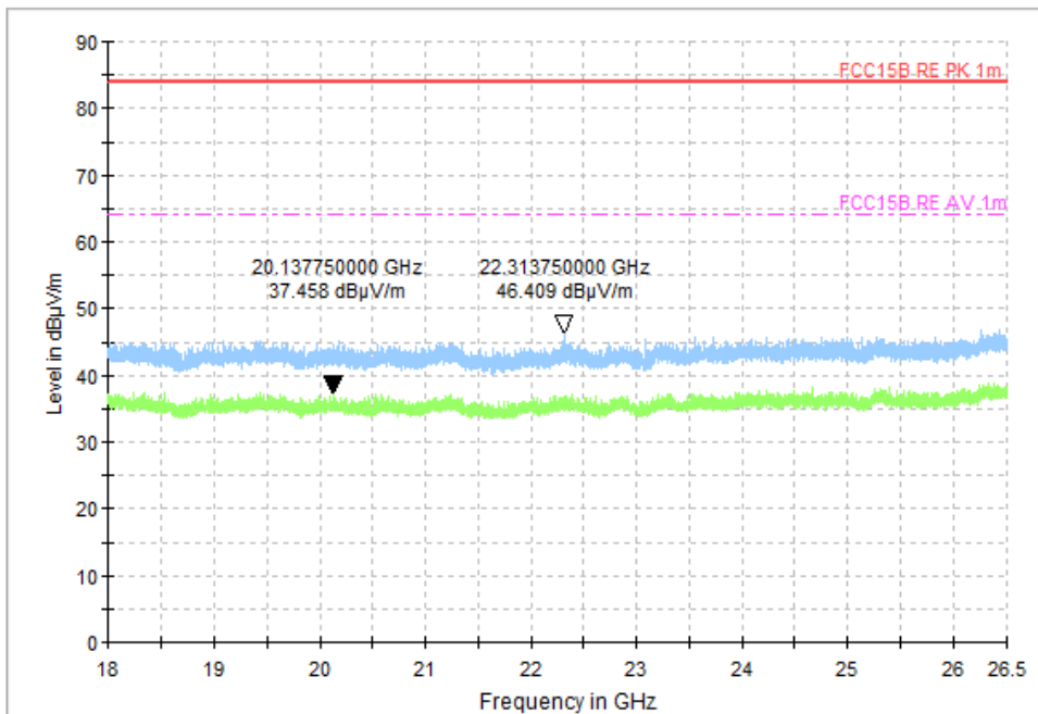
Fig.46 Radiated Spurious Emission (All Channels, 18 GHz-26.5 GHz), LE 1M
