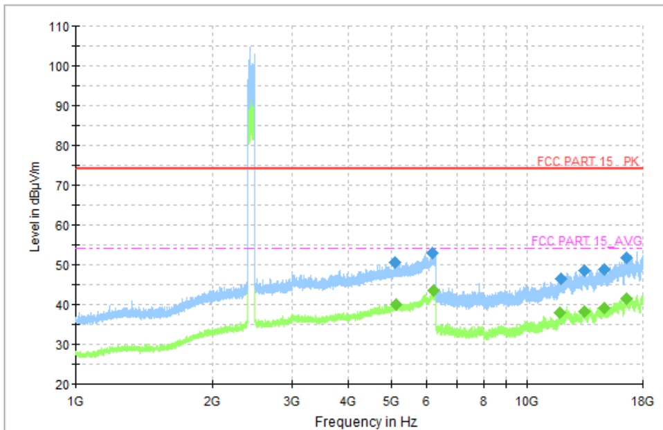
Fig.48 Radiated Spurious Emission (CH19, 1 GHz ~18 GHz), LE 2M
