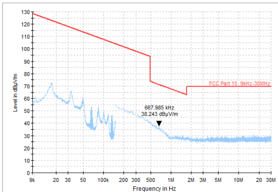
Fig.44 Radiated Spurious Emission (All Channels, 9 kHz-30 MHz), LE 1M
