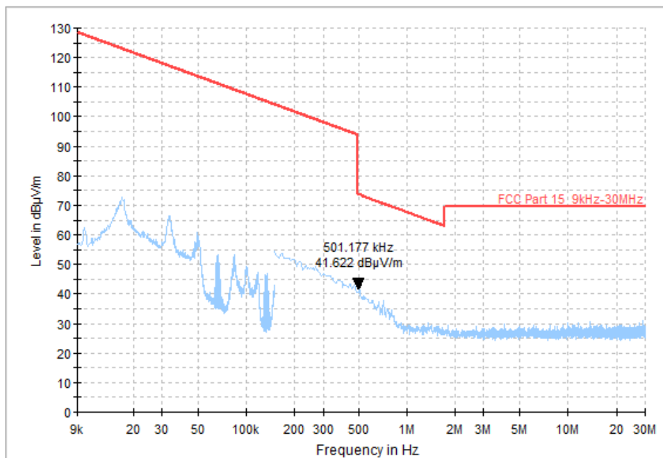
Fig.52 Radiated Spurious Emission (All Channels, 9 kHz-30 MHz), LE 2M
