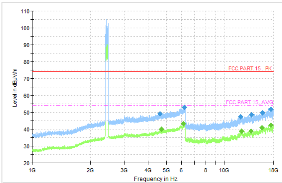
Fig.49 Radiated Spurious Emission (CH39, 1 GHz ~18 GHz), LE 2M
