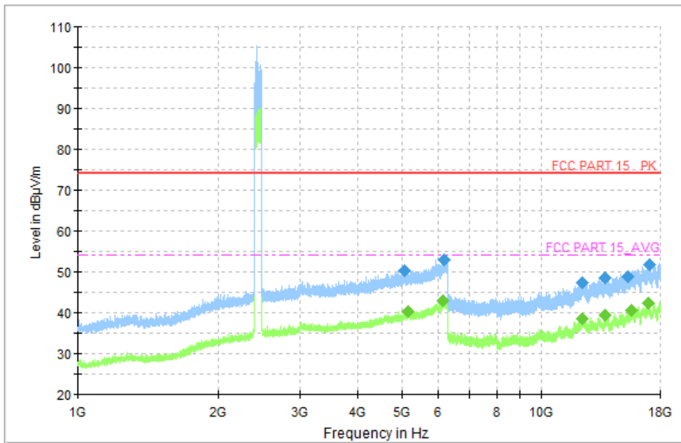
Fig.47 Radiated Spurious Emission (CH0, 1 GHz ~18 GHz), LE 2M
