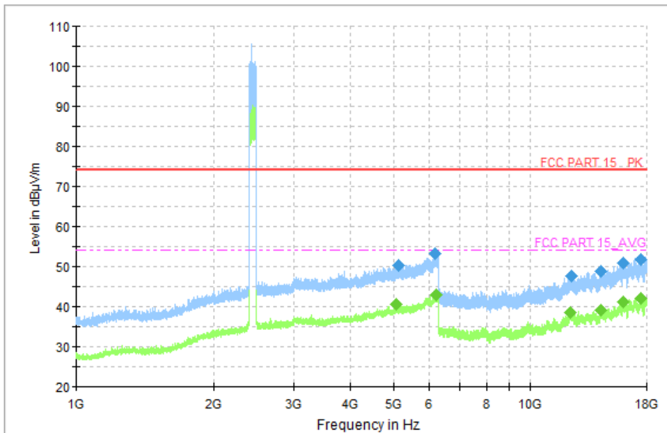
Fig.40 Radiated Spurious Emission (CH19, 1 GHz ~18 GHz), LE 1M
