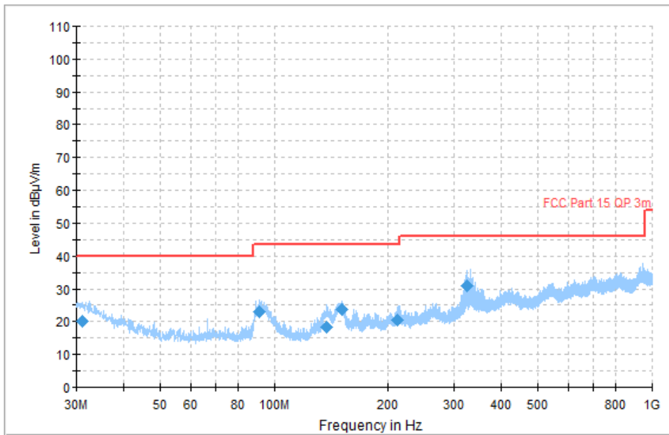
Fig.45 Radiated Spurious Emission (All Channels, 30 MHz-1 GHz), LE 1M
