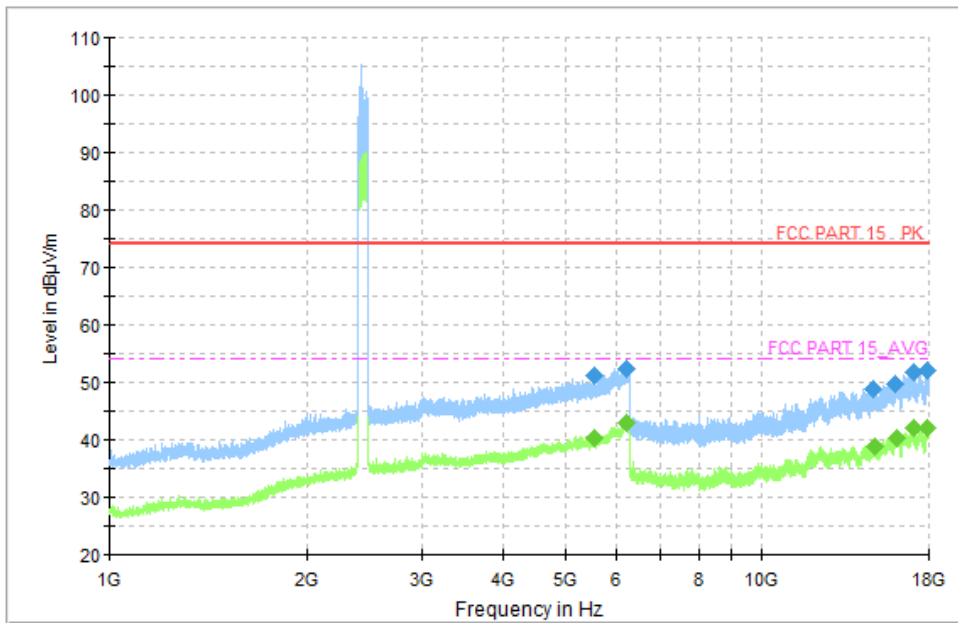
Fig.39 Radiated Spurious Emission (CH0, 1 GHz ~18 GHz), LE 1M
