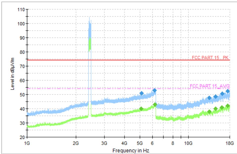
Fig.41 Radiated Spurious Emission (CH39, 1 GHz ~18 GHz), LE 1M
