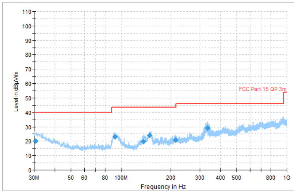
Fig.53 Radiated Spurious Emission (All Channels, 30 MHz-1 GHz), LE 2M
