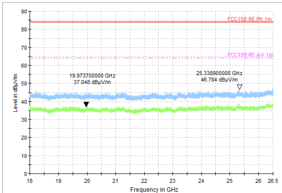
Fig.54 Radiated Spurious Emission (All Channels, 18 GHz-26.5 GHz), LE 2M
