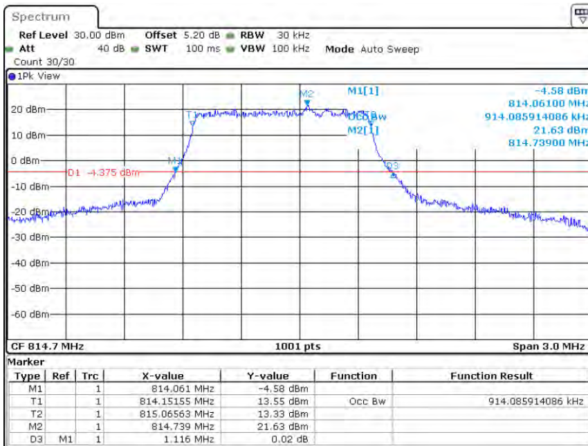
Band26-1.4MHz-QPSK-26697-6RB#0-0.914
