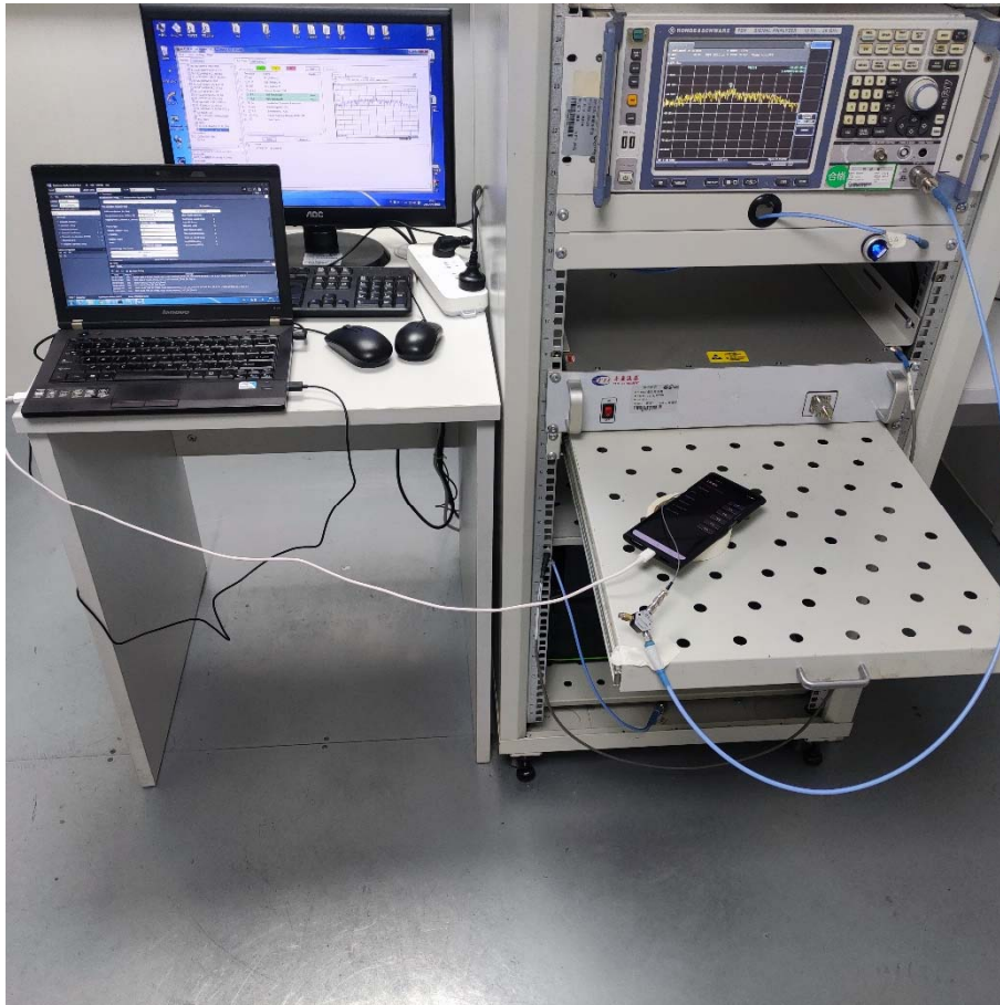
Conducted Test-BT3.0
