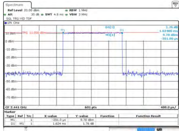
8-DPSK DH3
