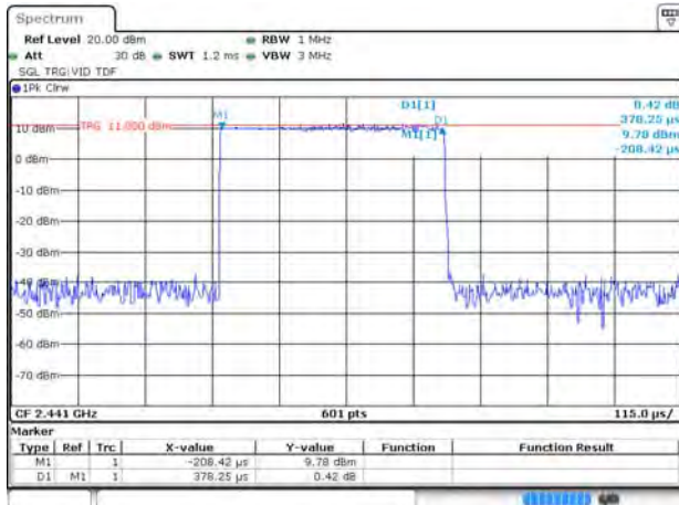
8-DPSK DH1
