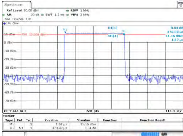
GFSK DH1
