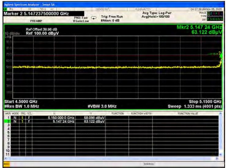
U-NII-1 11ac20 CH36 Peak
