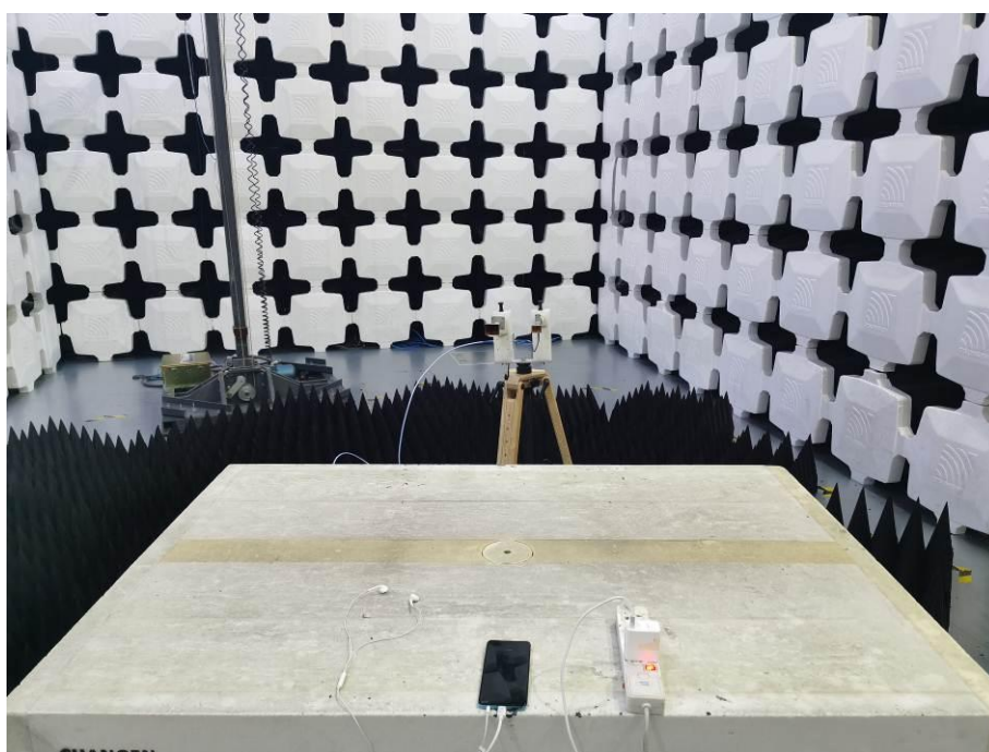
12. Radiated Emissions (Part 15B Camera/Video Player/GNSS/ FM receiver/NFC/GSM receiver/ WCDMA receiver/LTE receiver,26.5GHz-40GHz)
