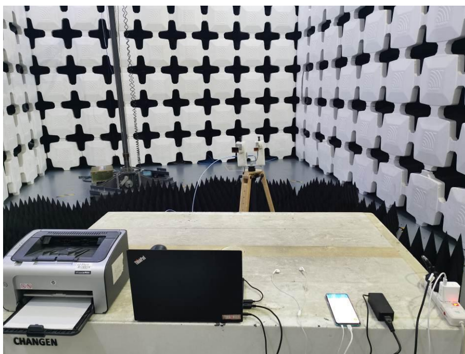
8. Radiated Emissions (Part 15B Bluetooth/Wi-Fi, 26.5GHz-40GHz)
