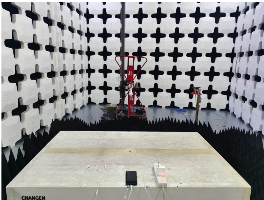
10. Radiated Emissions (Part 15B Camera/Video Player/GNSS/ FM receiver/NFC/GSM receiver/ WCDMA receiver/LTE receiver,1GHz-18GHz)
