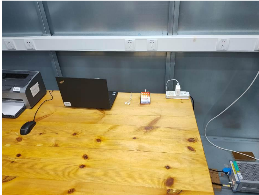
19. Conducted Emission (Part 15B, Bluetooth/Wi-Fi)
