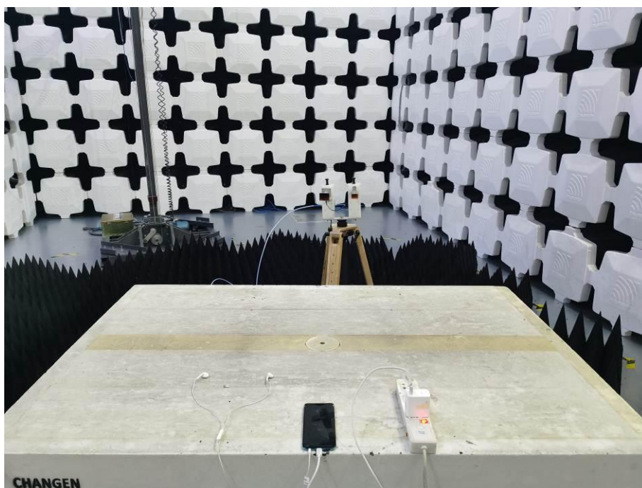
11. Radiated Emissions (Part 15B Camera/Video Player/GNSS/ FM receiver/NFC/GSM receiver/ WCDMA receiver/LTE receiver,26.5GHz-40GHz)
