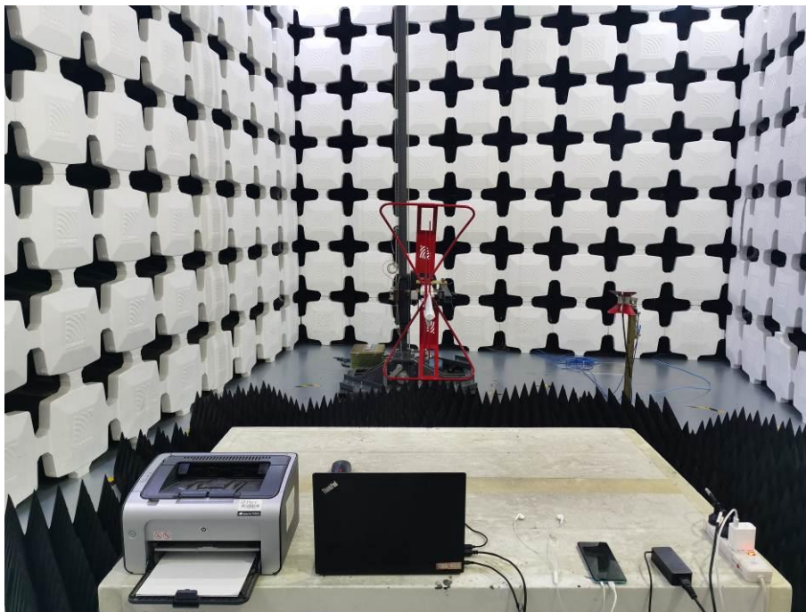
6. Radiated Emissions (Part 15B Bluetooth/Wi-Fi, 1GHz-18GHz)
