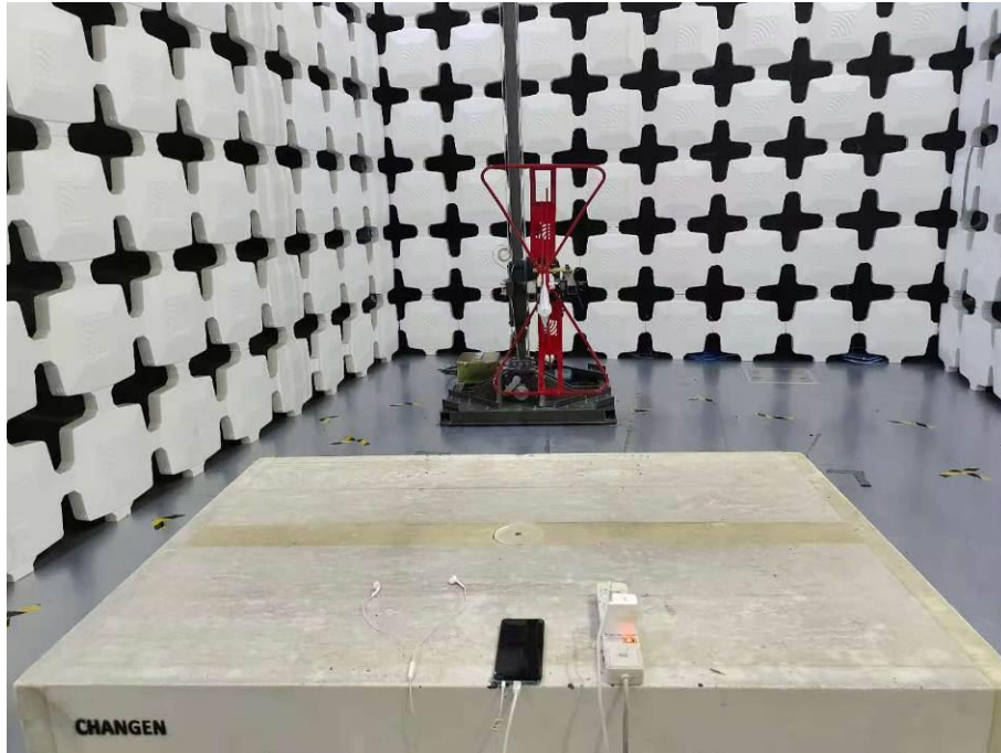
9. Radiated Emissions (Part 15B Camera/Video Player/GNSS/ FM receiver/NFC/GSM receiver/ WCDMA receiver/LTE receiver,30MHz-1GHz)
