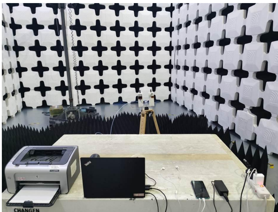
7. Radiated Emissions (Part 15B Bluetooth/Wi-Fi, 26.5GHz-40GHz)
