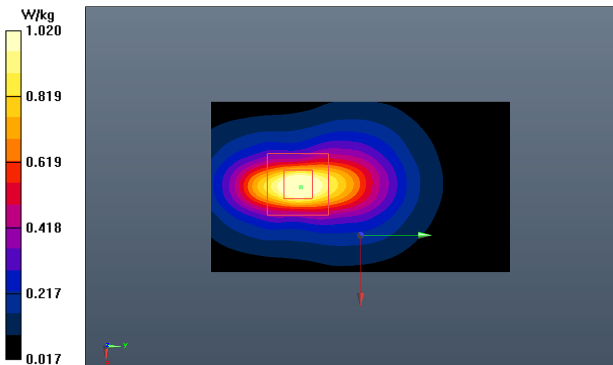
Fig.14 LTE Band 4
