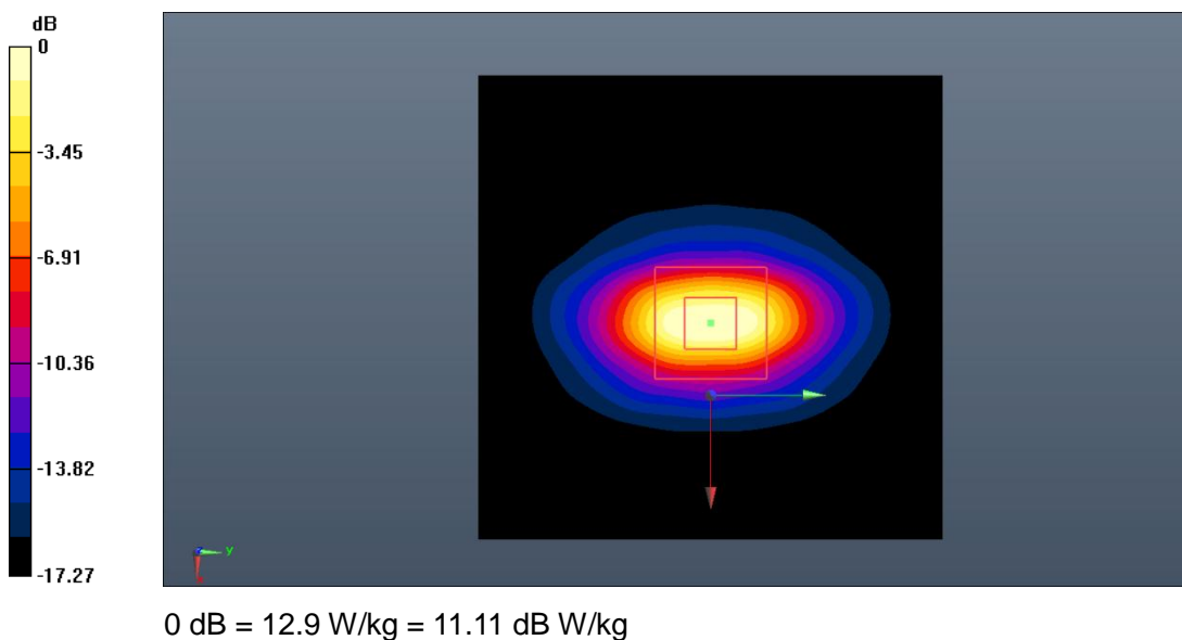
Fig.B.4. Validation 1900MHz 250mW
