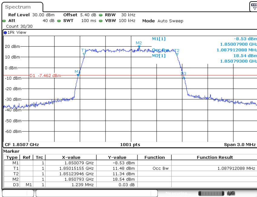
Band2-1.4MHz-QPSK-18607-6RB#0-1.088
