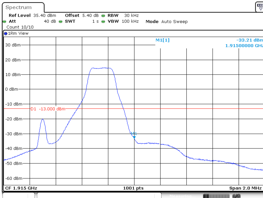
Band25-1.4MHz-64QAM-26683-1RB#5
