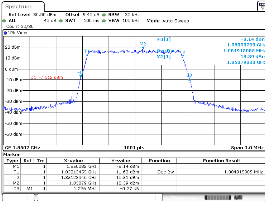
Band25-1.4MHz-QPSK-26047-6RB#0-1.085
