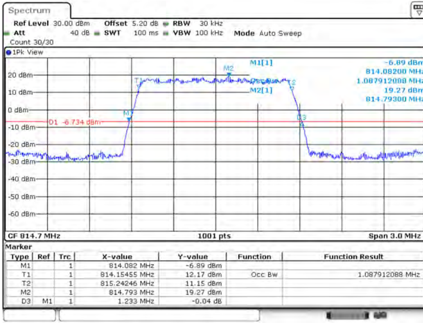
Band26-1.4MHz-QPSK-26697-6RB#0-1.088
