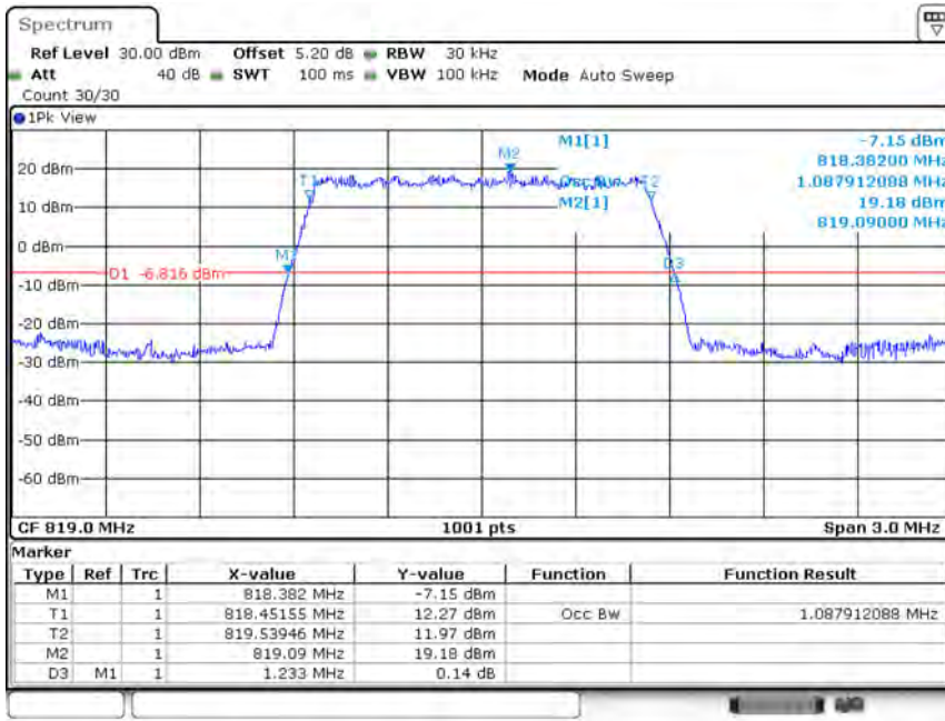
Band26-1.4MHz-QPSK-26740-6RB#0-1.088
