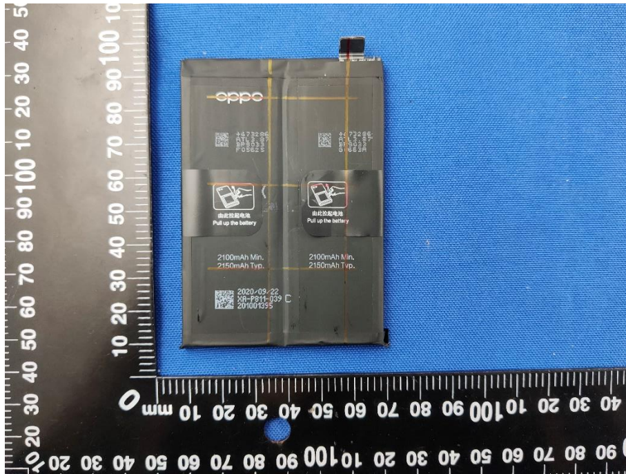
Battery Photo (BLP811 (Dongguan NVT Technology Co., Ltd.)) (FRONT)
