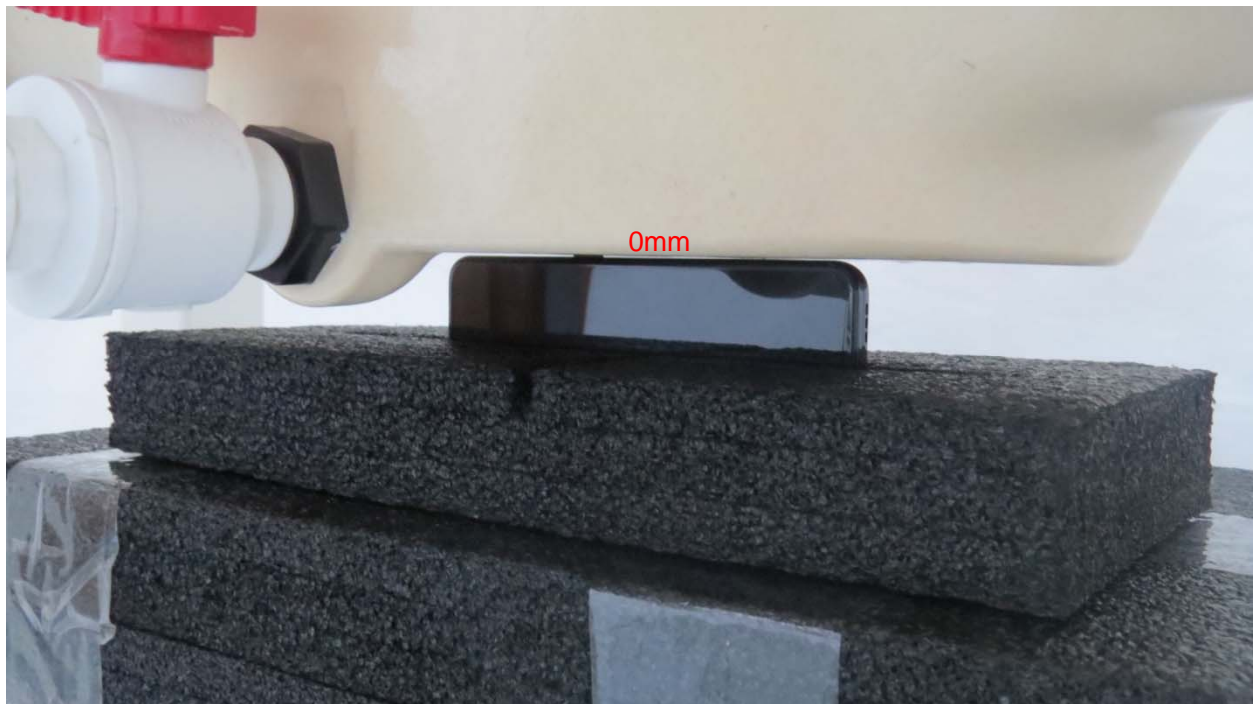
Picture 14: Right Side, the distance from handset to the bottom of the Phantom is 0mm
