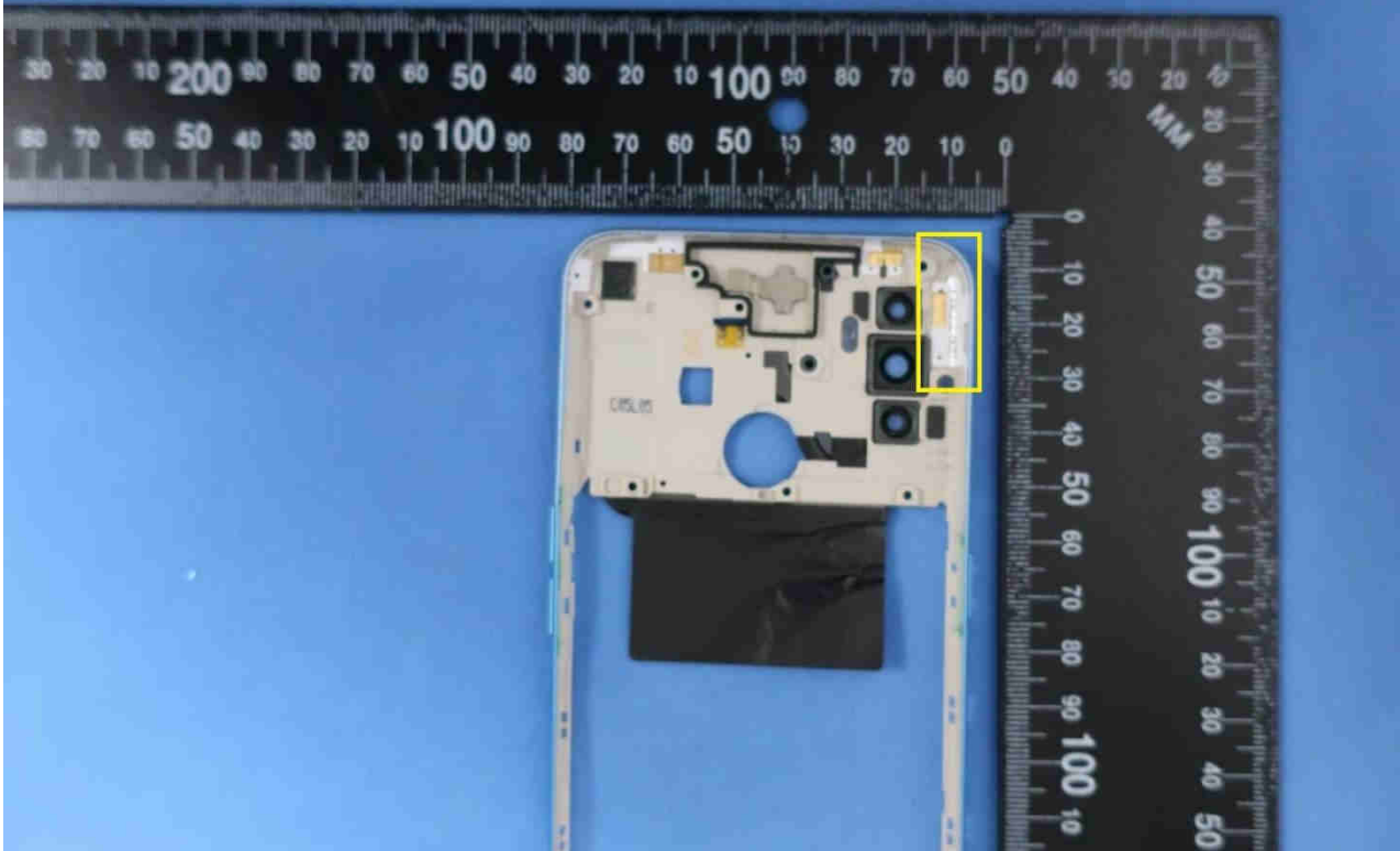
Bluetooth & WLAN 2.4&5G Antenna <Tx/Rx>
