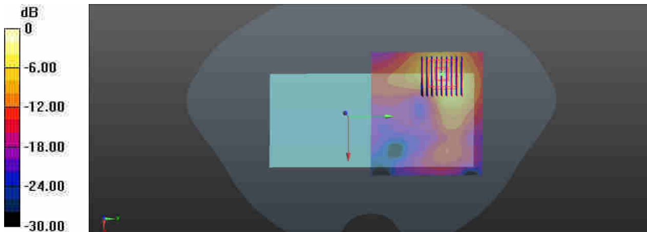
0 dB = 1.01 W/kg
