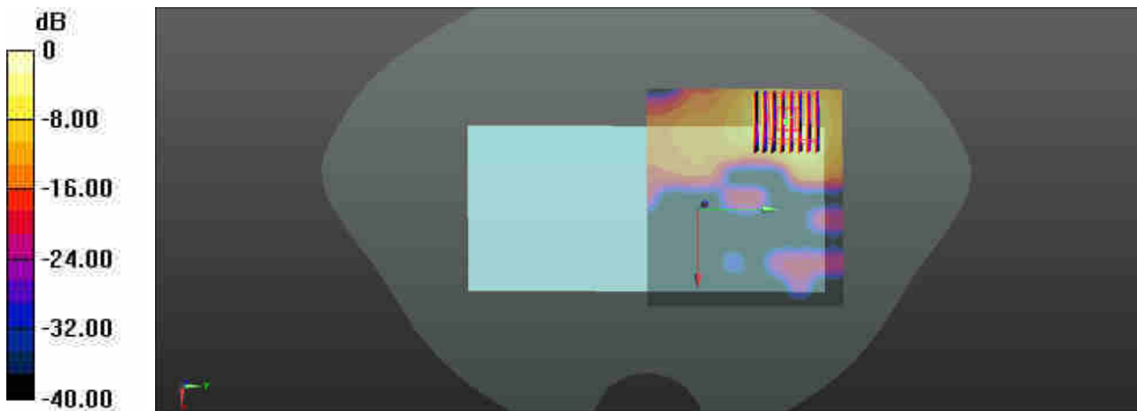
0 dB = 1.21 W/kg
