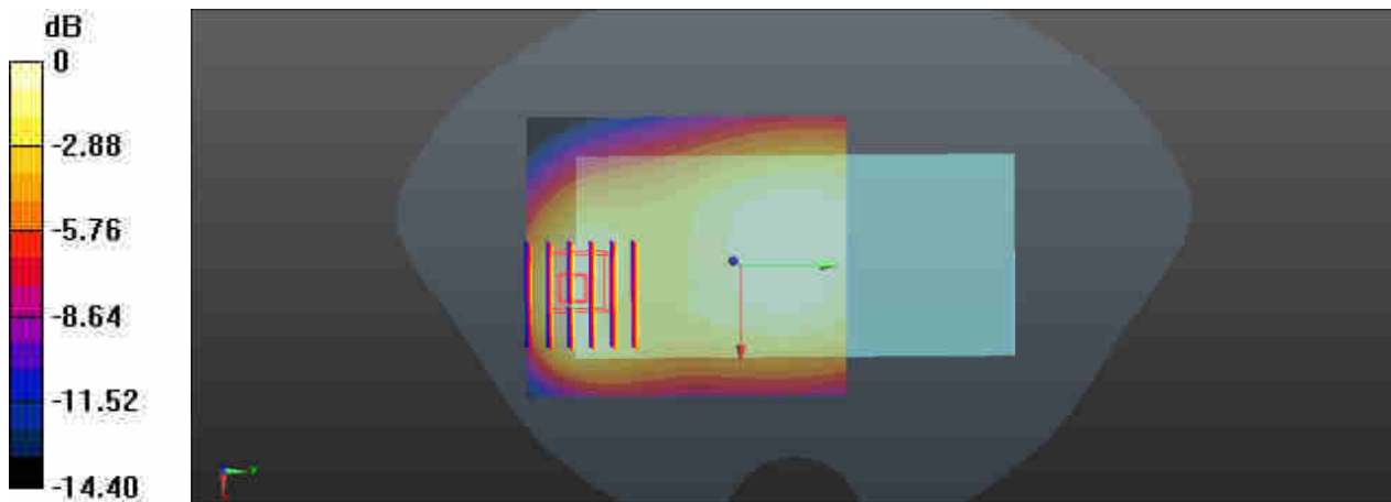
0 dB = 0.392 W/kg
