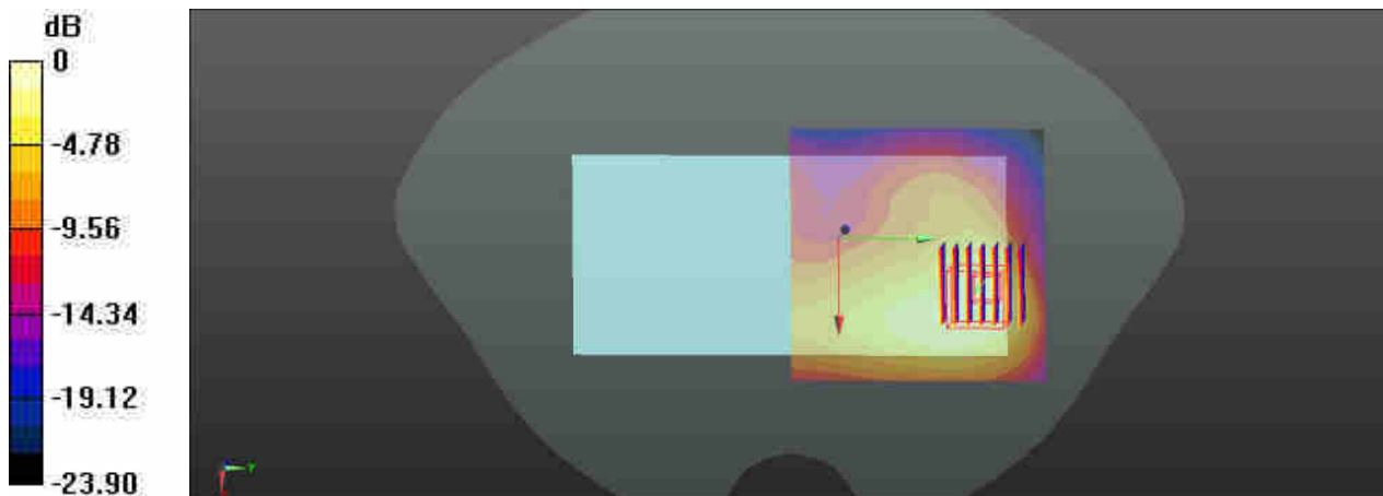
0 dB = 0.610 W/kg
