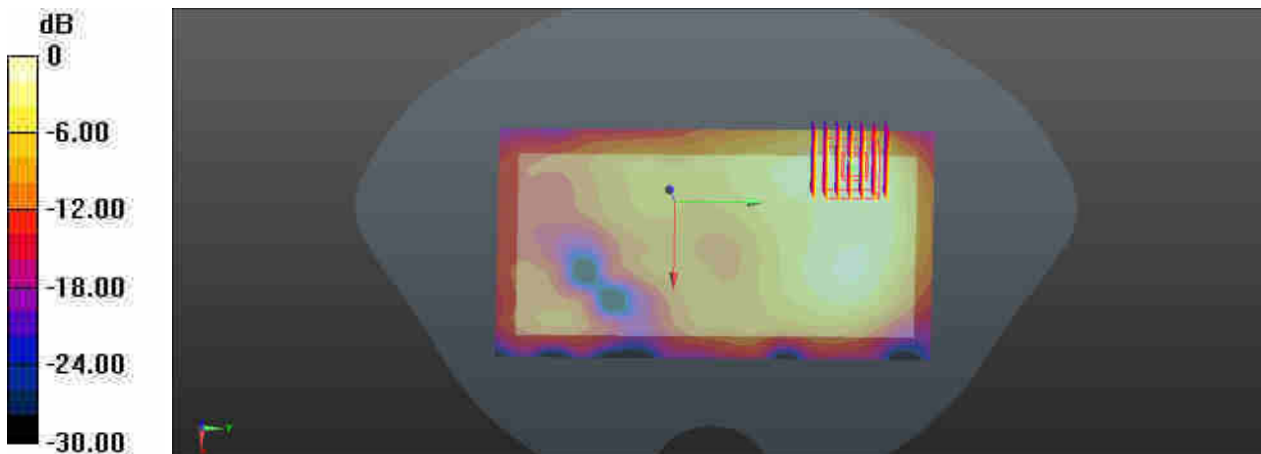
0 dB = 0.103 W/kg
