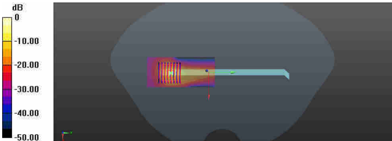
0 dB = 16.3 W/kg
