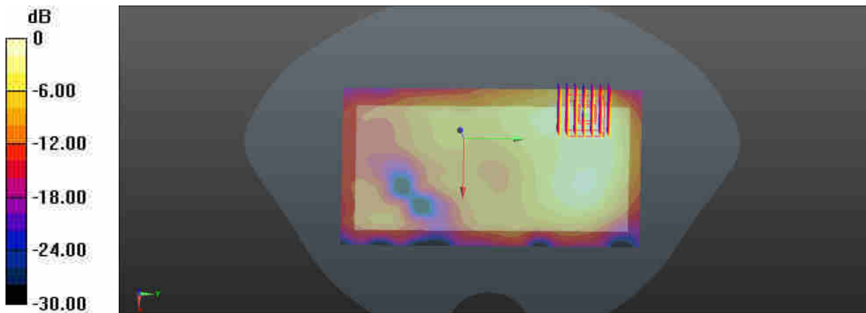
0 dB = 0.103 W/kg
