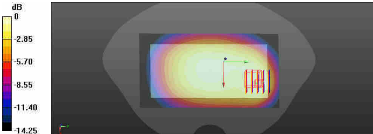
0 dB = 0.212 W/kg
