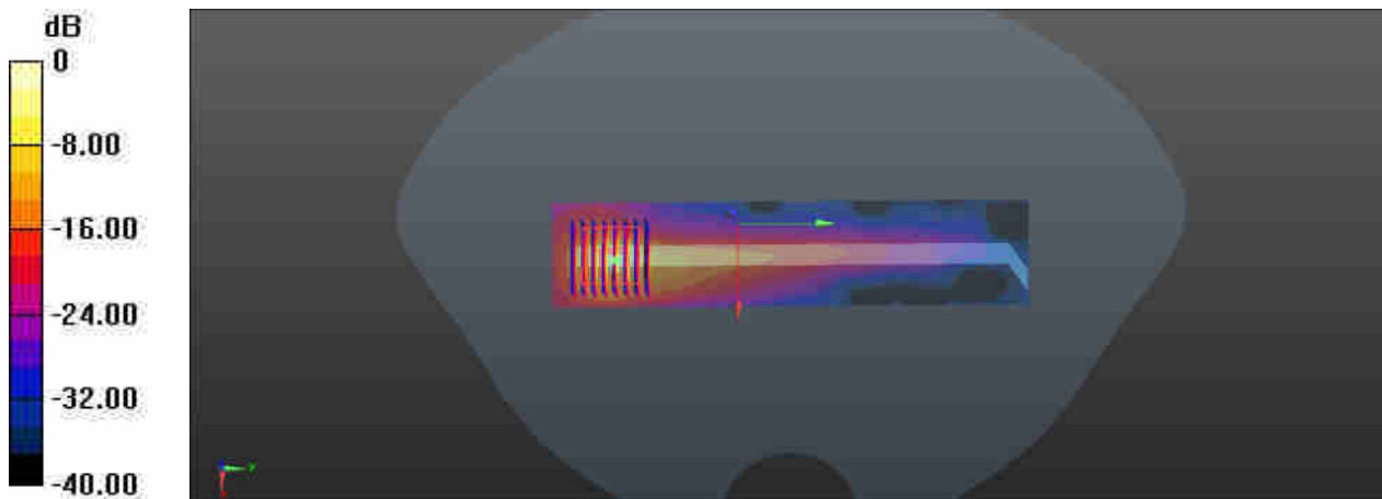
0 dB = 11.0 W/kg
