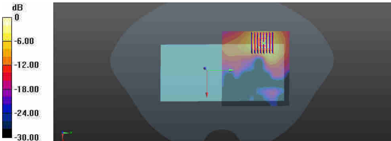
0 dB = 1.07 W/kg
