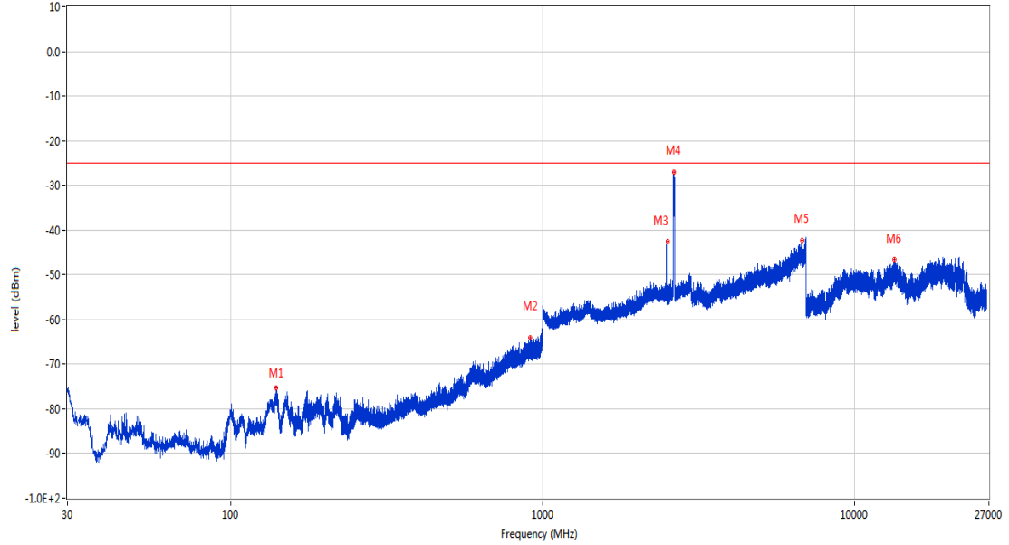
OPPO_RSE (RF )_FCC PART22&24&27_LTE Band 7 & 41(low)_2496-2570_30MHz-27GHz_
