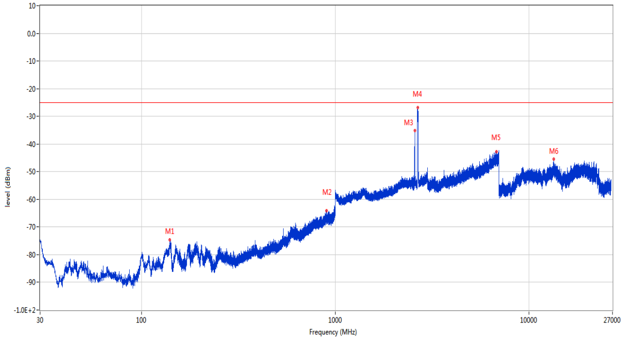
OPPO_RSE (RF) _FCC PART22&24&27_LTE Band 7 & 41(low) _2496-2570_30MHz-27GHz_
