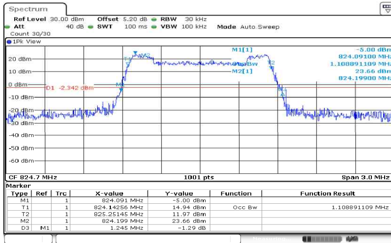
Band5-1.4MHz-QPSK-20407-6RB#0-1.109
