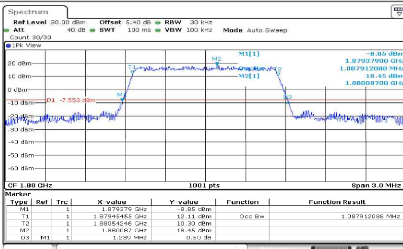
Band2-1.4MHz-QPSK-18900-6RB#0-1.088
