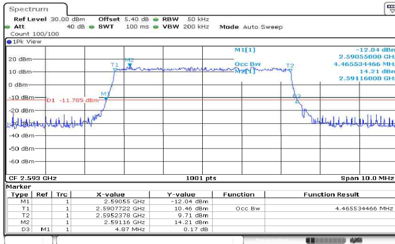
Band41-5MHz-QPSK-40620-25RB#0-4.466
