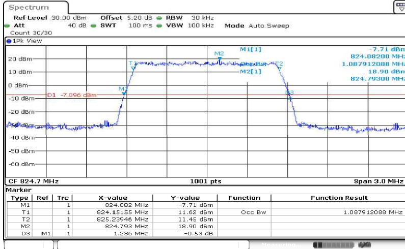
Band26-1.4MHz-QPSK-26797-6RB#0-1.088
