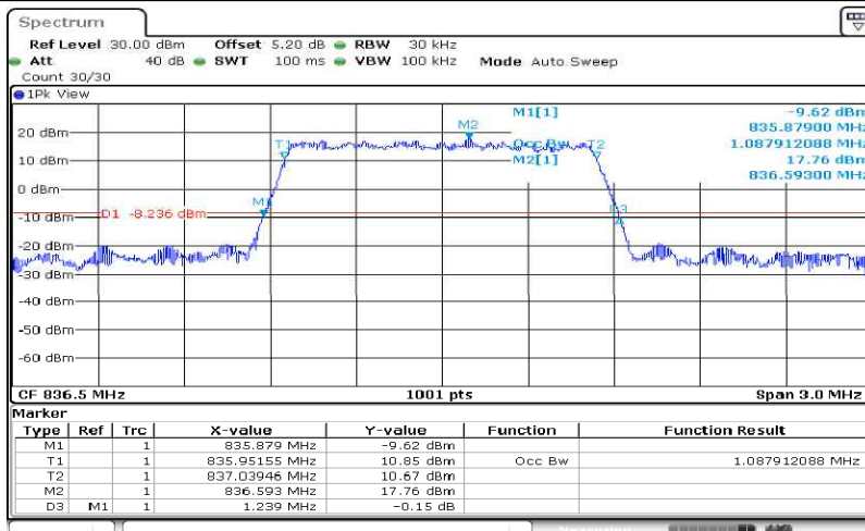
Band26-1.4MHz-QPSK-26915-6RB#0-1.088
