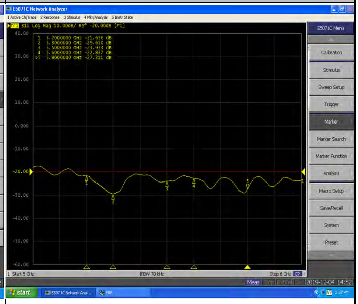
Return Loss-Head
