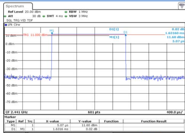
GFSK DH3
