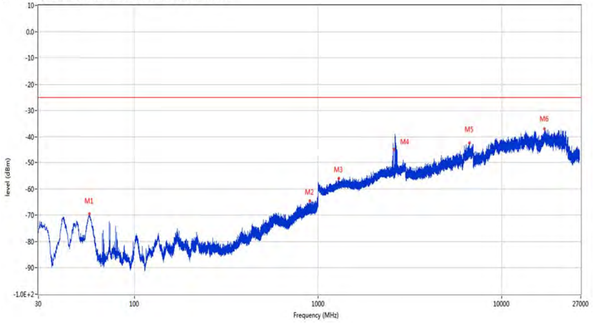
OPPO 特殊要求_RSE Test case_FCC PART228&248&27_FCC PART 27_2535_LTE B38 & B41
