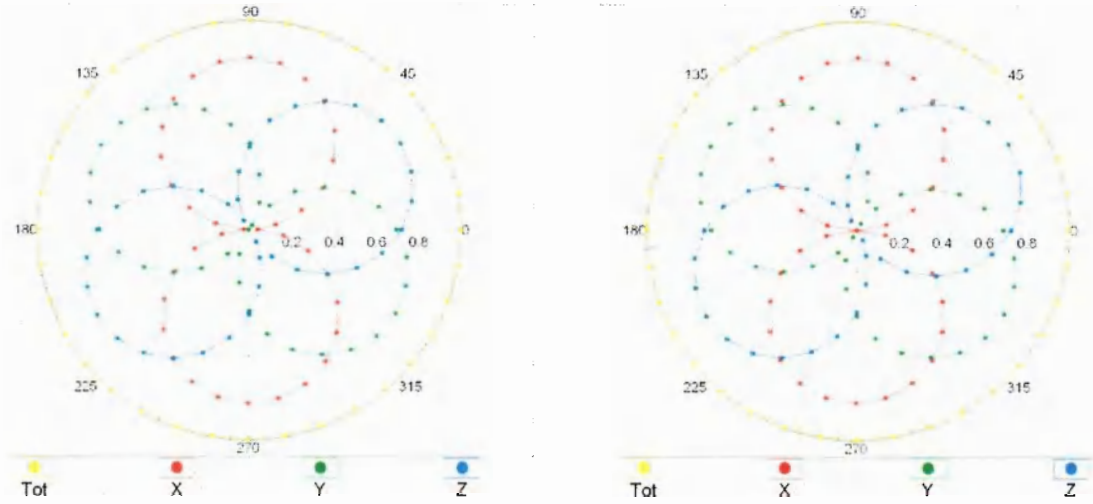
f=600 MHz,TEM
