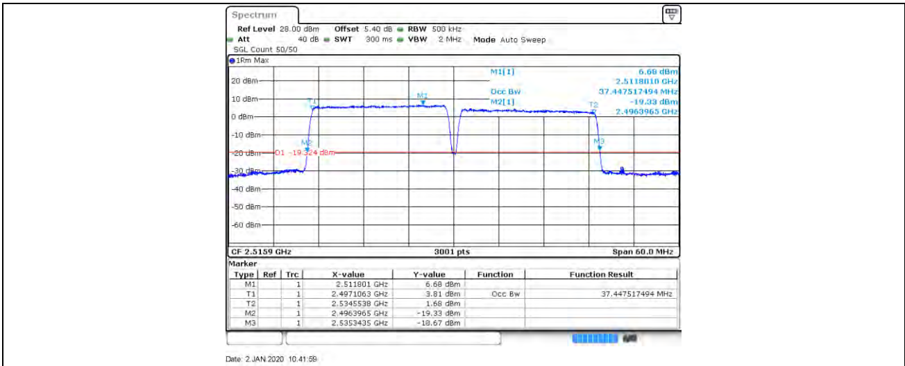
LTE Band CA 41C_100RB+100RB_64QAM_40521+40719_100RB#0+100RB#0
