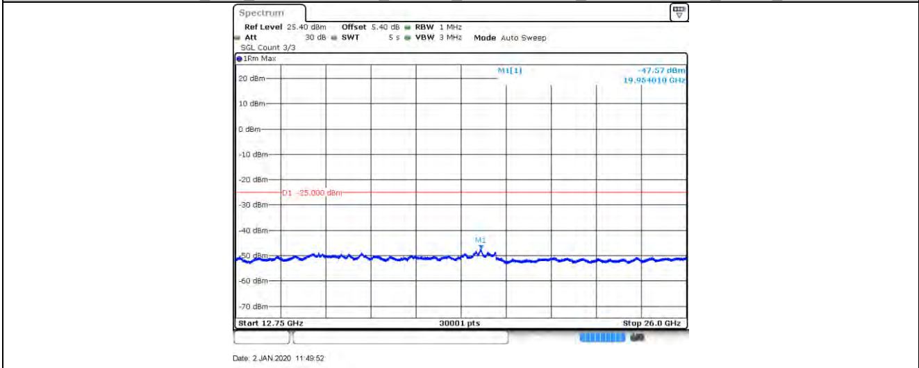
LTE Band CA_41C_100RB+100RB_64QAM_39750+39948_1RB#0+0RB#0_30_1000
