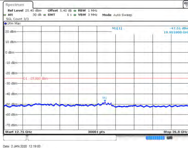
LTE Band CA_41C_100RB+100RB_QPSK_39948+39750_1RB#0+0RB#0_30_1000
