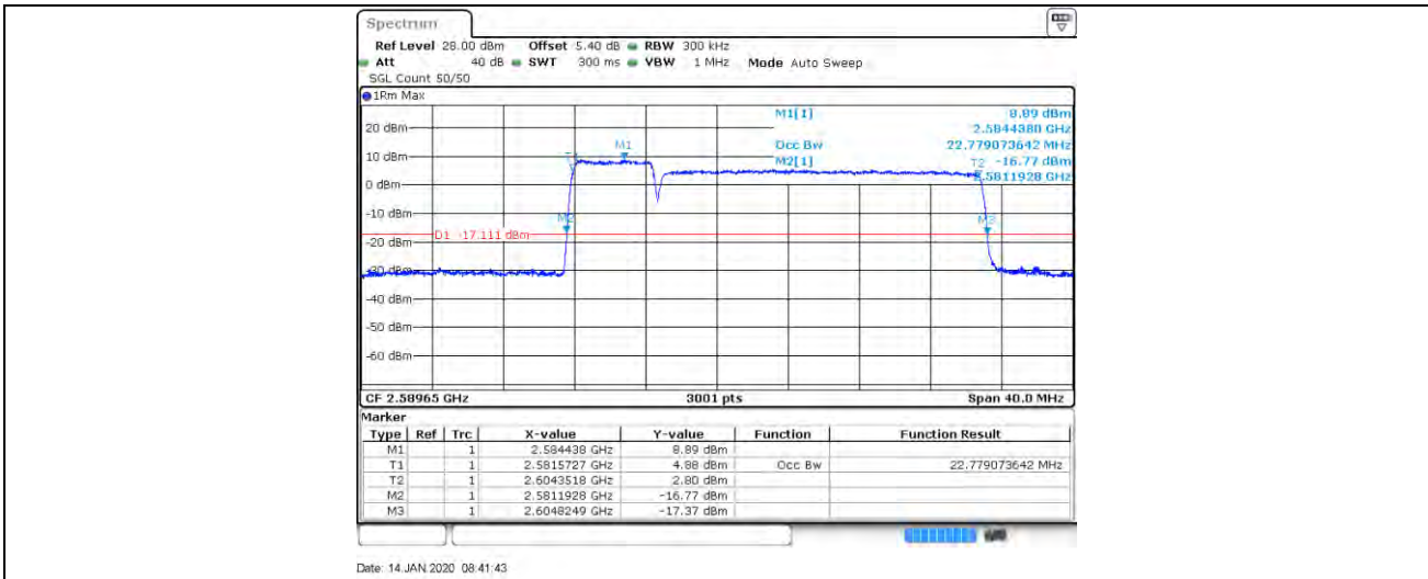
LTE Band CA_41C_25RB+100RB_QPSK_41490+41373_100RB#0+25RB#0
