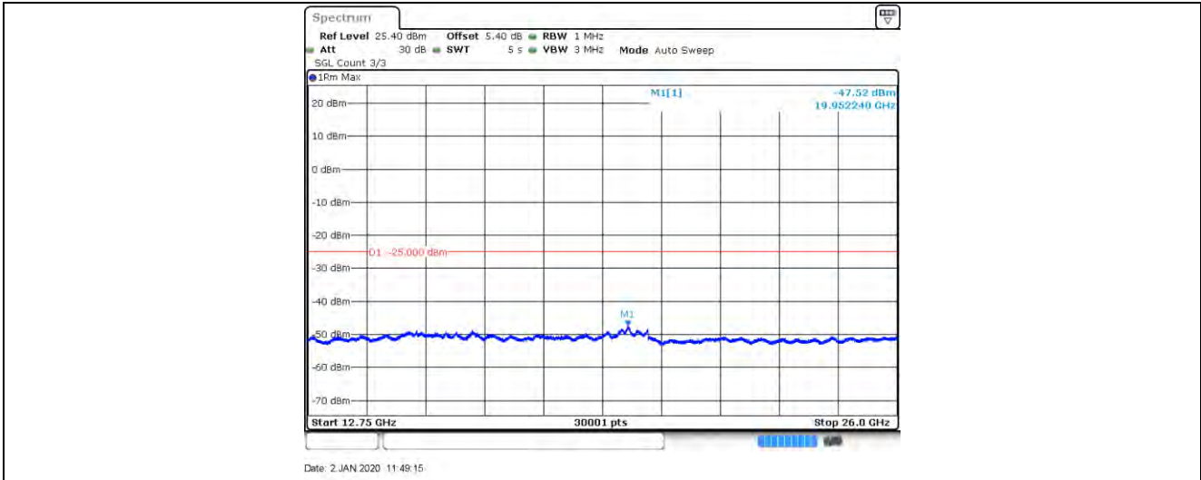
LTE Band CA_41C_100RB+100RB_64QAM_41490+41292_1RB#0+0RB#0_30_1000
