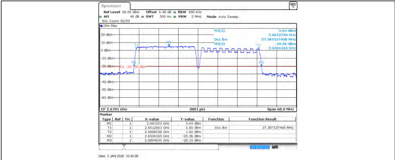
LTE Band CA 41C_100RB+100RB_16QAM_39948+39750_100RB#0+100RB#0
