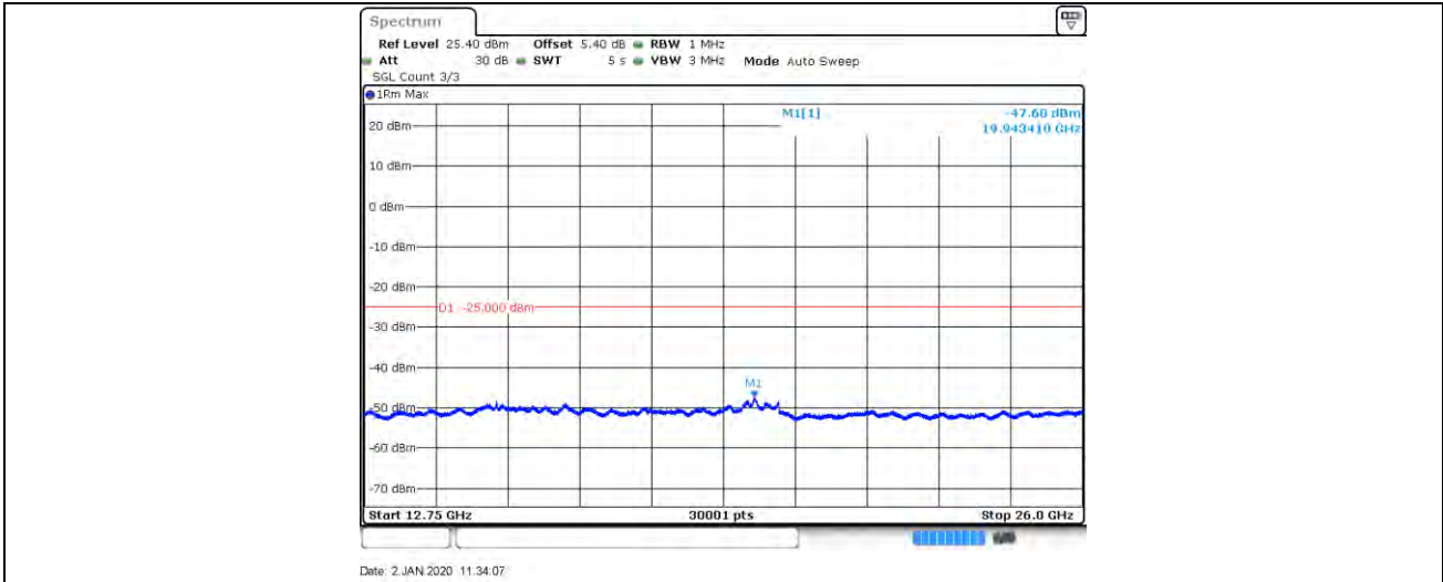
LTE Band CA_7C_100RB+100RB_64QAM_21001+21199_1RB#0+0RB#0_30_1000
