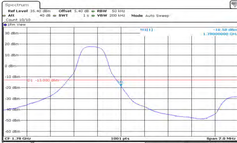
Band66-3MHz-QPSK-132657-15RB#0
