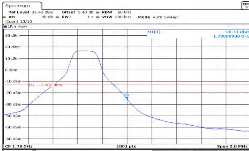
Band66-5MHz-16QAM-132647-25RB#0
