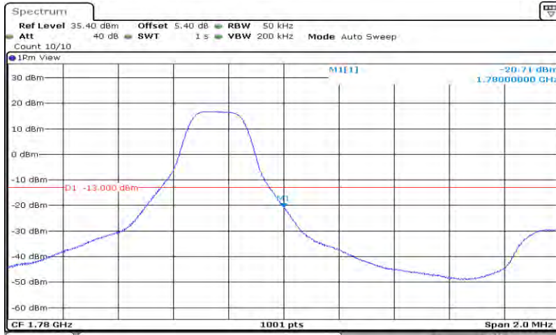
Band66-3MHz-16QAM-132657-15RB#0
