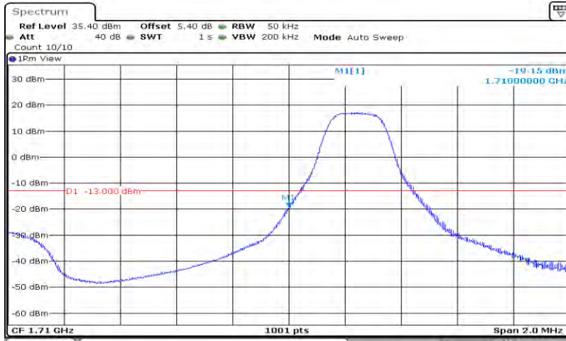
Band66-3MHz-16QAM-131987-15RB#0
