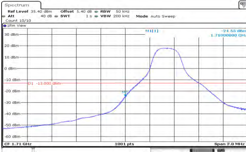
Band66-5MHz-QPSK-131997-25RB#0
