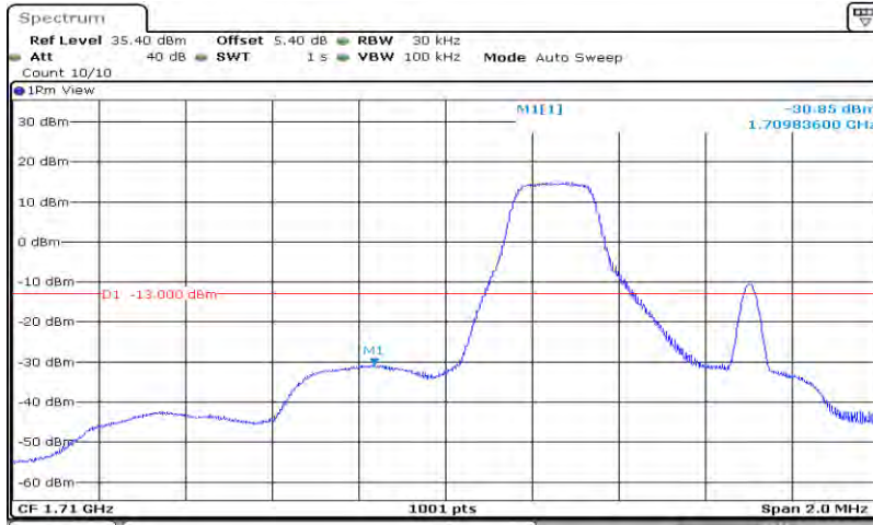
Band66-1.4MHz-64QAM-131979-6RB#0
