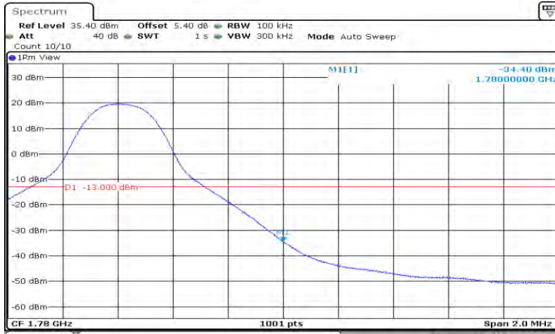
Band66-10MHz-16QAM-132622-50RB#0
