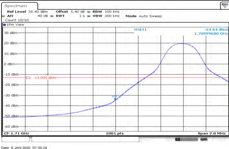
Band66-10MHz-16QAM-132022-50RB#0
