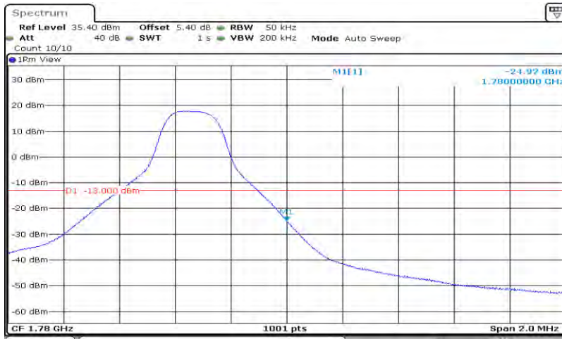
Band66-5MHz-QPSK-132647-25RB#0
