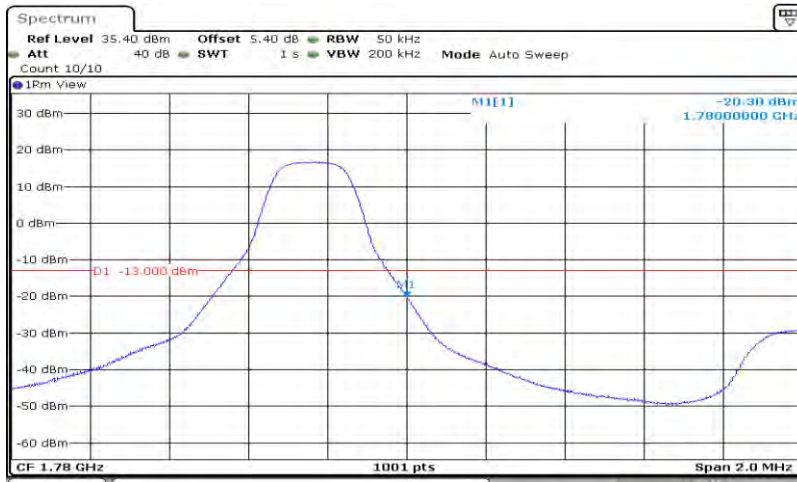
Band66-3MHz-64QAM-132657-15RB#0
