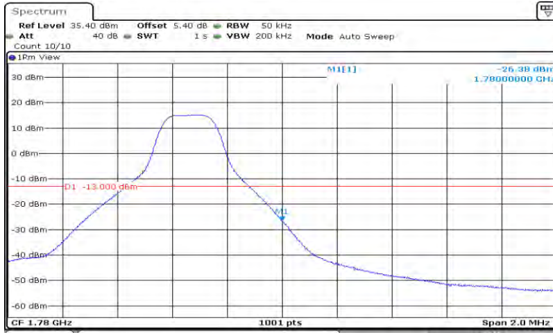
Band66-5MHz-64QAM-132647-25RB#0
