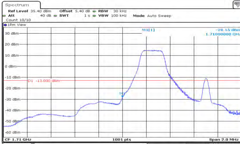
Band66-1.4MHz-16QAM-131979-6RB#0
