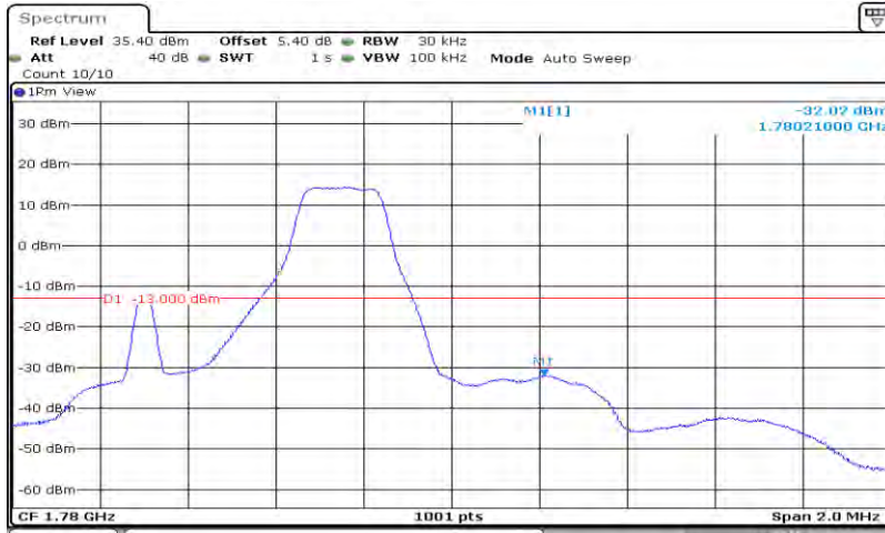
Band66-1.4MHz-16QAM-132665-6RB#0
