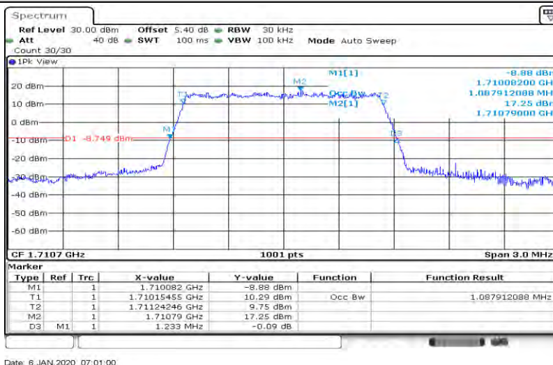
Band66-1.4MHz-QPSK-132322-6RB#0-1.088
