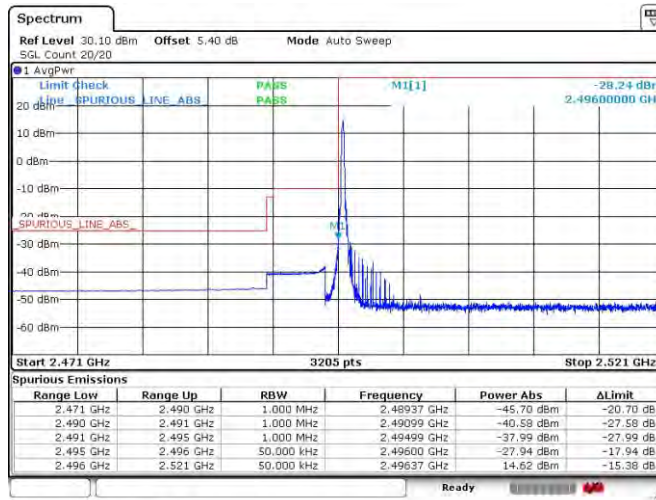
Band41_5MHz_64QAM_39675_25RB#0
