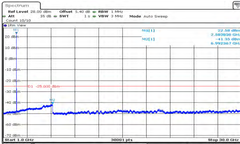
Band41-20MHz-16QAM-40620-1RB#0-Range2:1000~30000MHz
