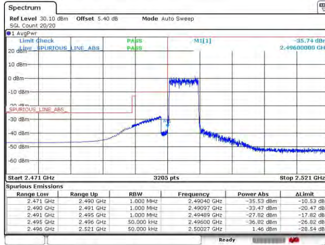
Band41_5MHz_64QAM_39675_25RB#0
