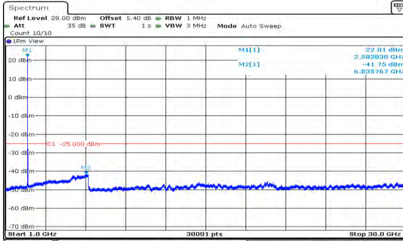
Band41-20MHz-64QAM-40620-1RB#0-Range2:1000~30000MHz
