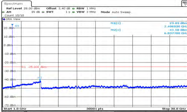
Band41-20MHz-64QAM-39750-1RB#0-Range2:1000~30000MHz
