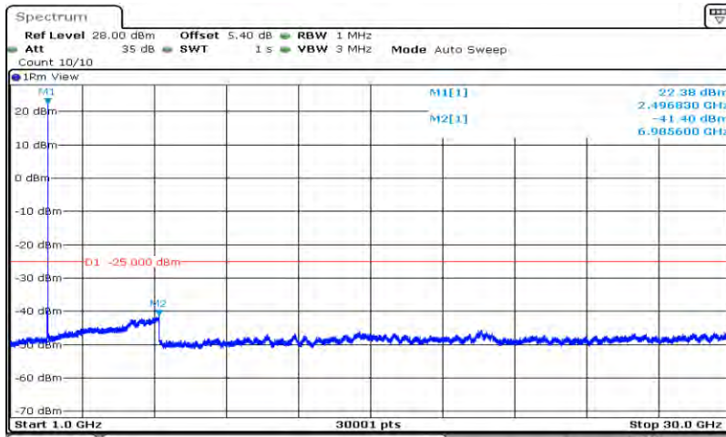
Band41-20MHz-16QAM-39750-1RB#0-Range2:1000~30000MHz
