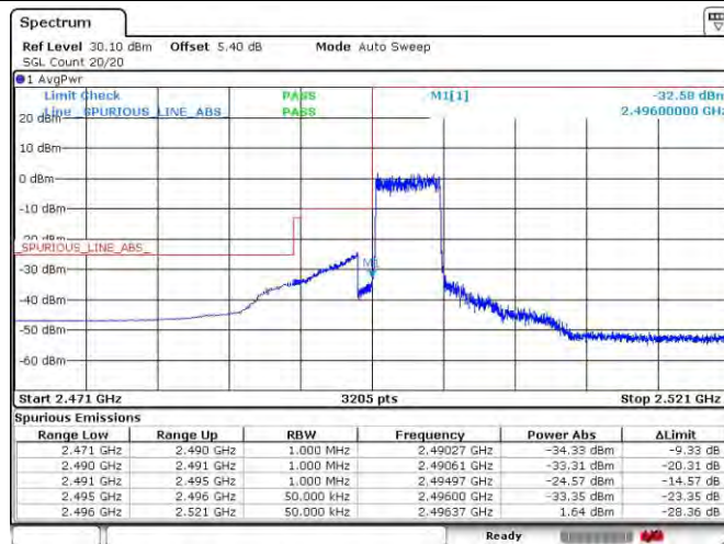
Band41_5MHz_QPSK_39675_25RB#0
