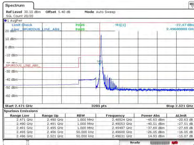
Band41_5MHz_QPSK_39675_1RB#0
