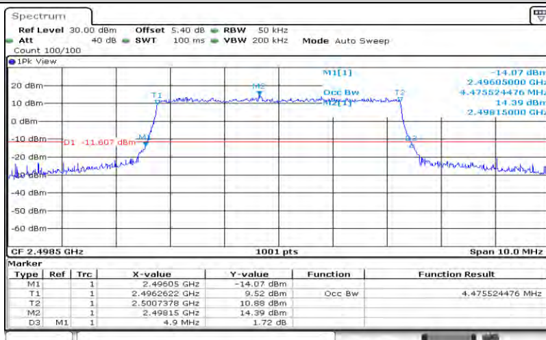
Band41-5MHz-QPSK-39675-25RB#0-4.476
