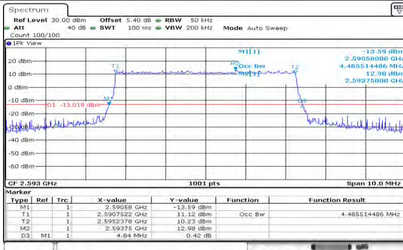
Band41-5MHz-QPSK-40620-25RB#0-4.486
